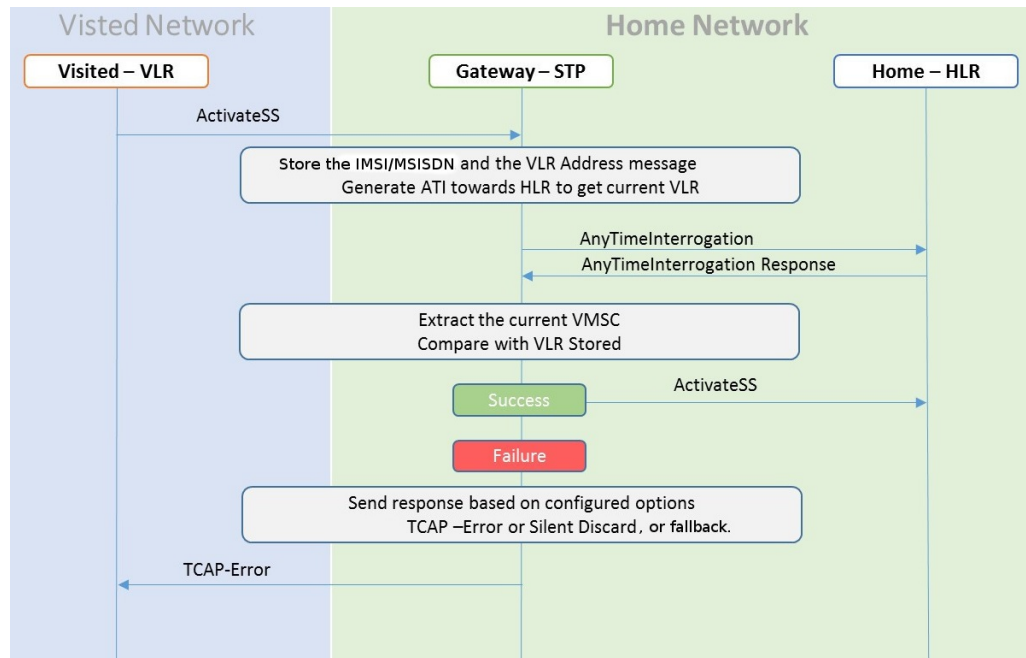
Figure 2-1 Call Flow for VLR Validation
