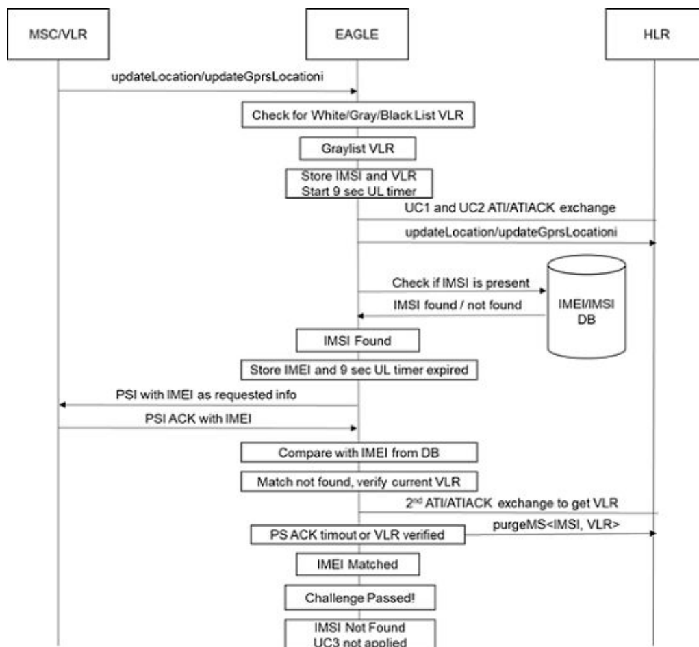
Figure 2-7 Graylisted VLR Challenge
