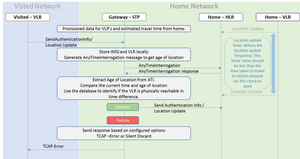
Figure 2-2 Call Flow for Velocity Check Using ATI
