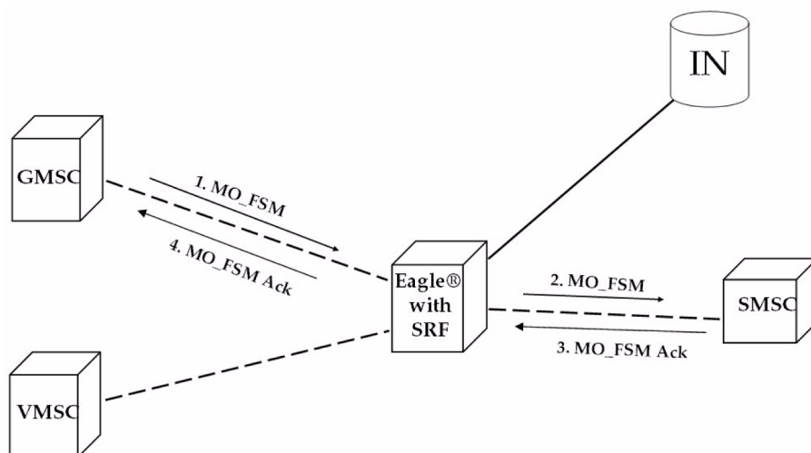
Figure 2-5 Successful Delivery of MO_FSM from Contract Subscriber
