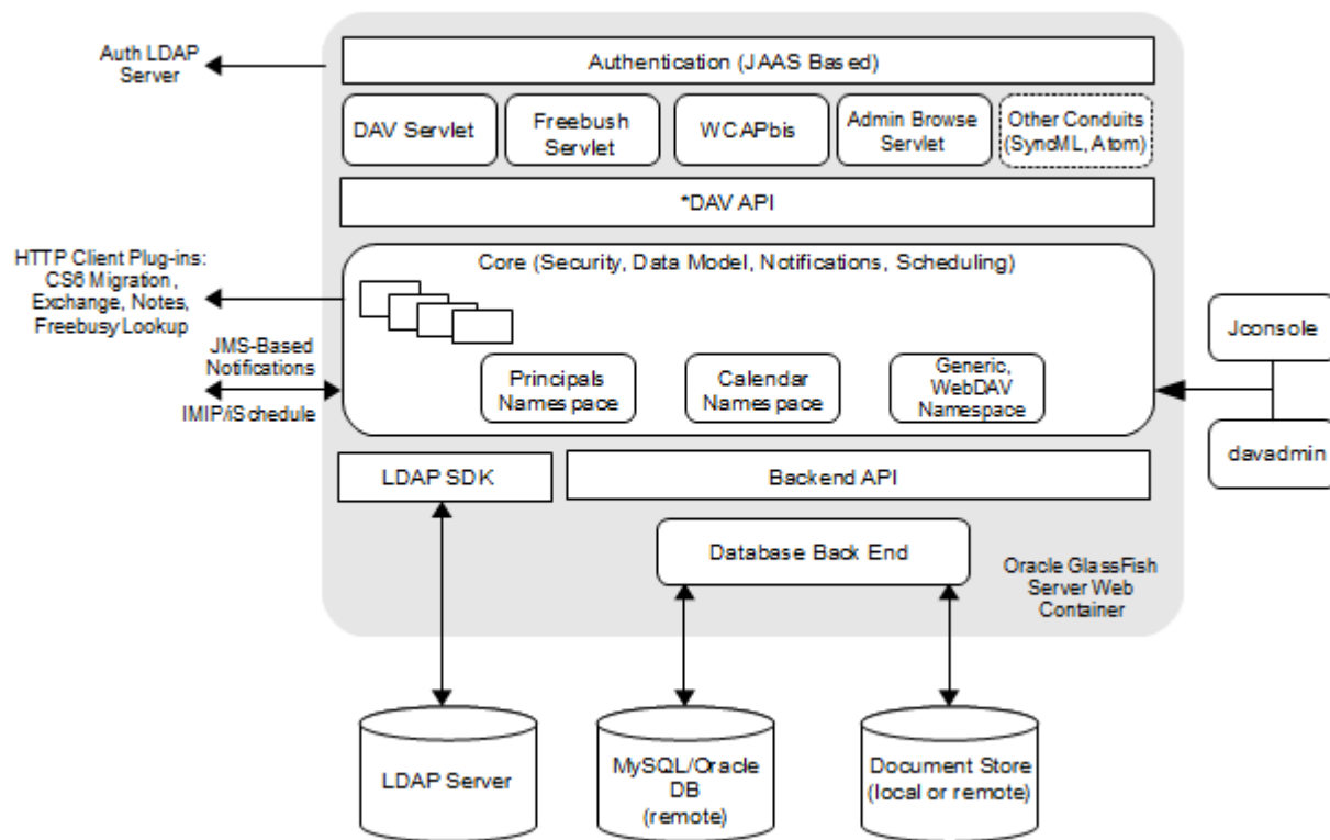
Figure 1-1 Calendar Server Software Architecture
