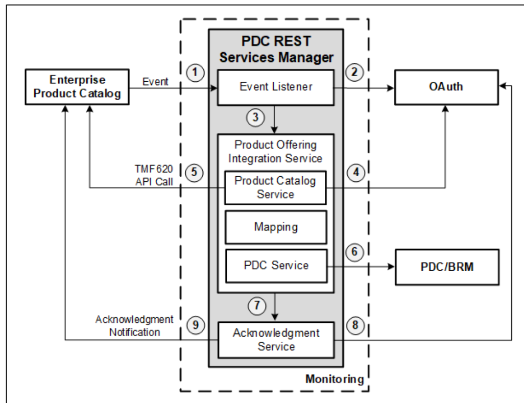
Figure 1-1 PDC REST Services Manager Architecture
