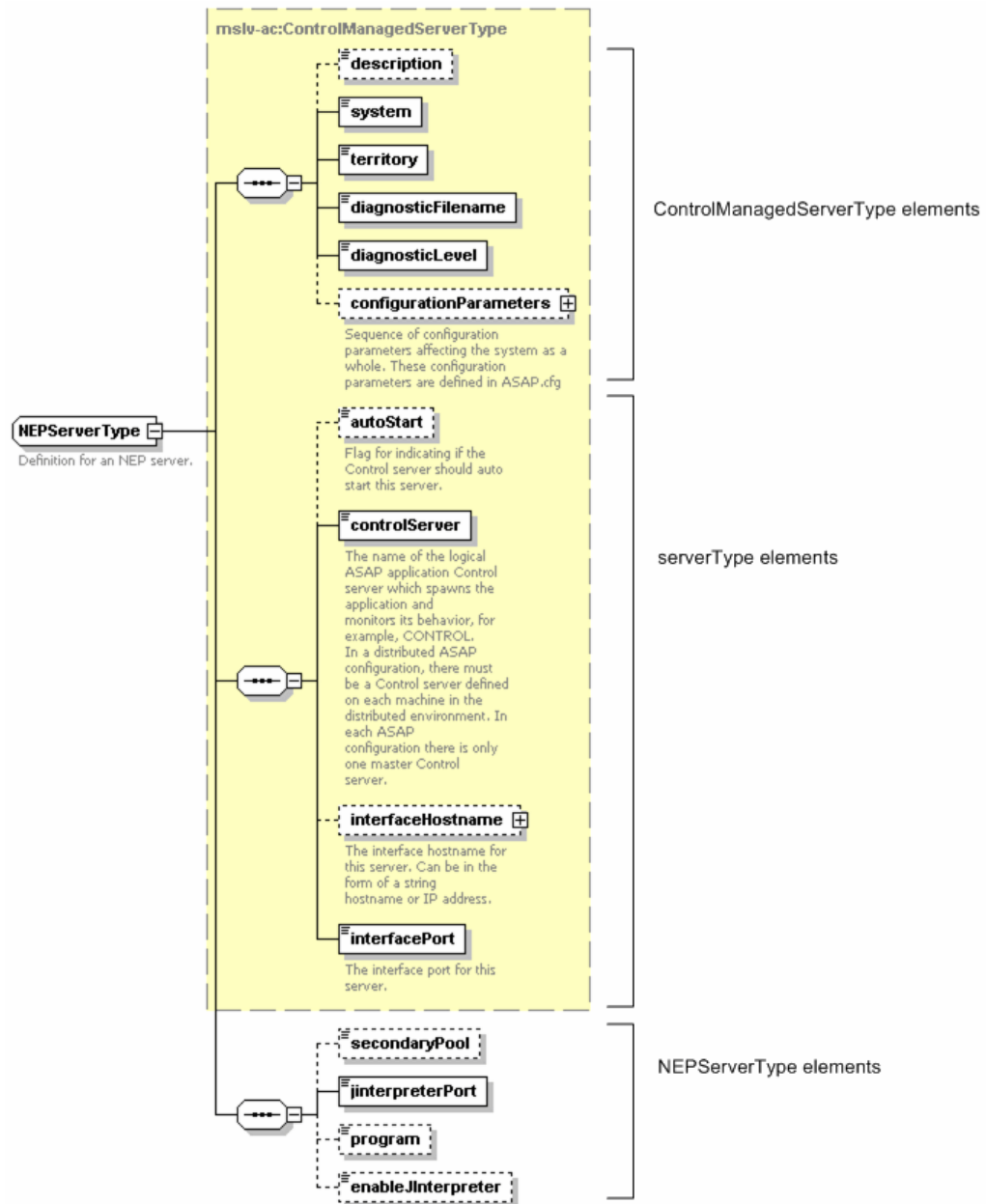
Figure 2-3 NEPServerType Schema
