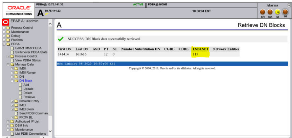
Figure 3-82 Retrieve a DN Block Screen
