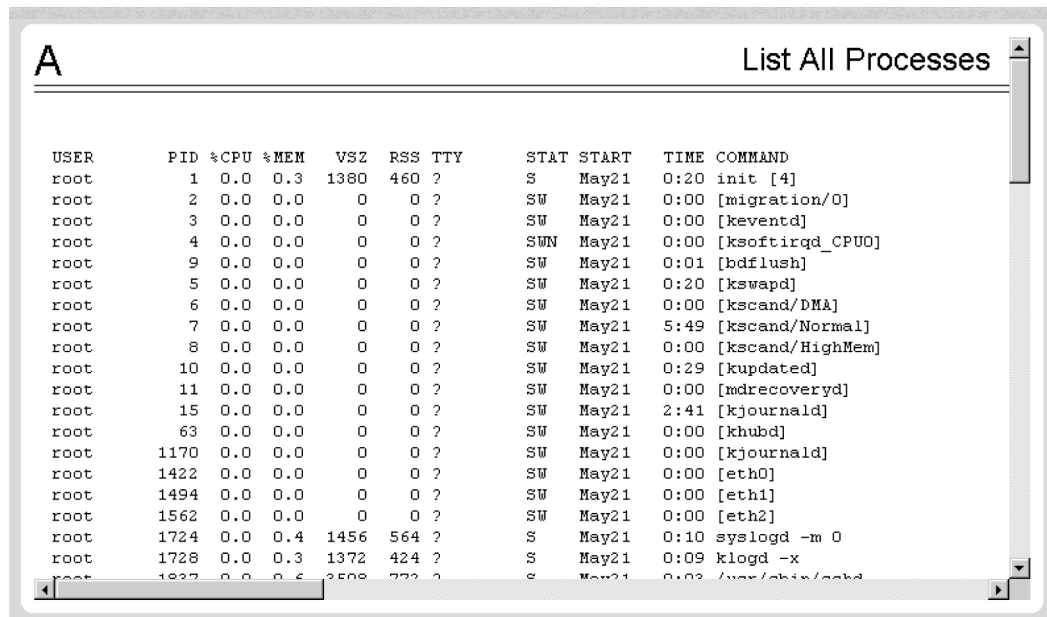
Figure 3-61 List All Processes Screen
