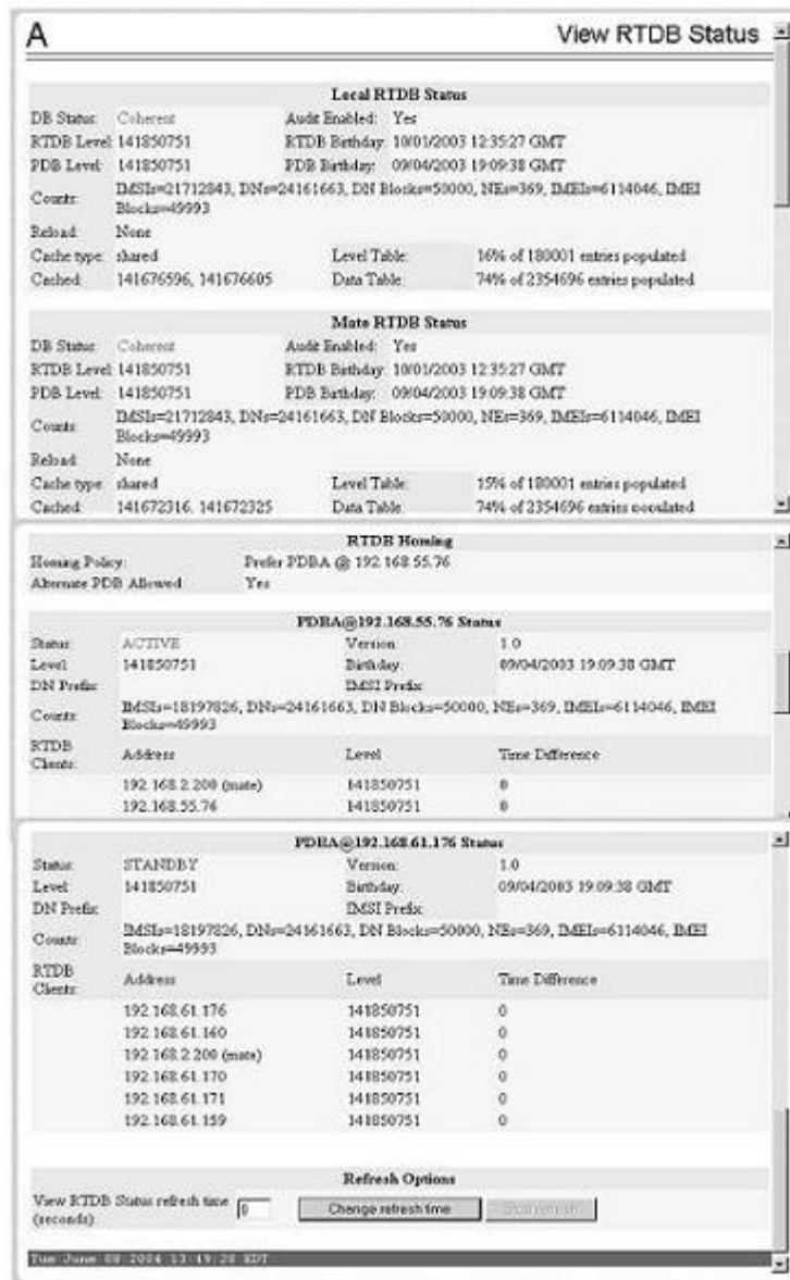
Figure 3-37 View RTDB Status Screen
