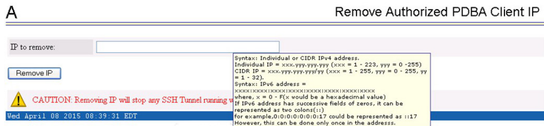
Figure 3-95 Remove Authorized PDBA Client IP
