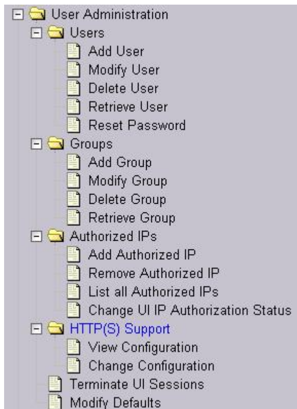
Figure 6-20 EPAP A User Administration Menu
