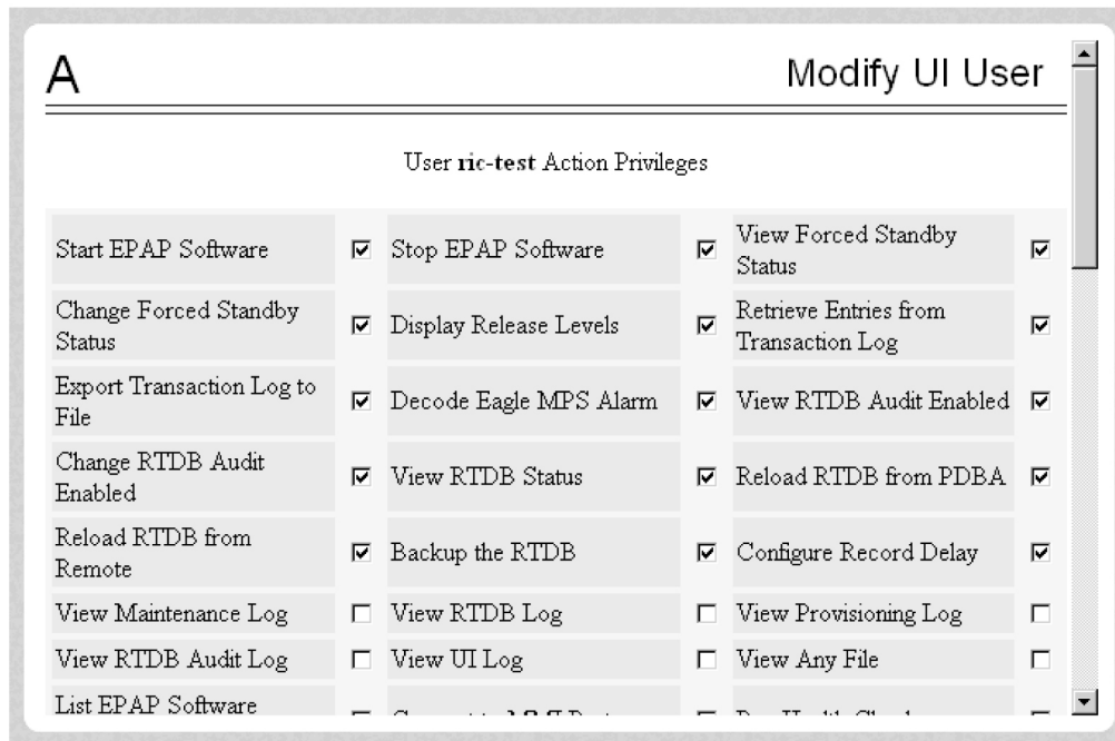
Figure 3-101 Modify UI User's Specific Actions
