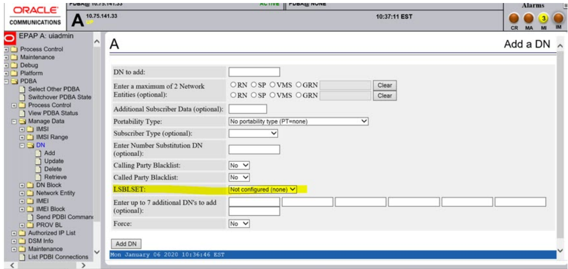
Figure 3-75 Add a DN Screen
