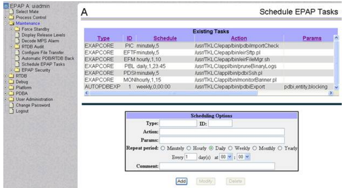
Figure 3-33 Schedule EPAP Tasks Screen
