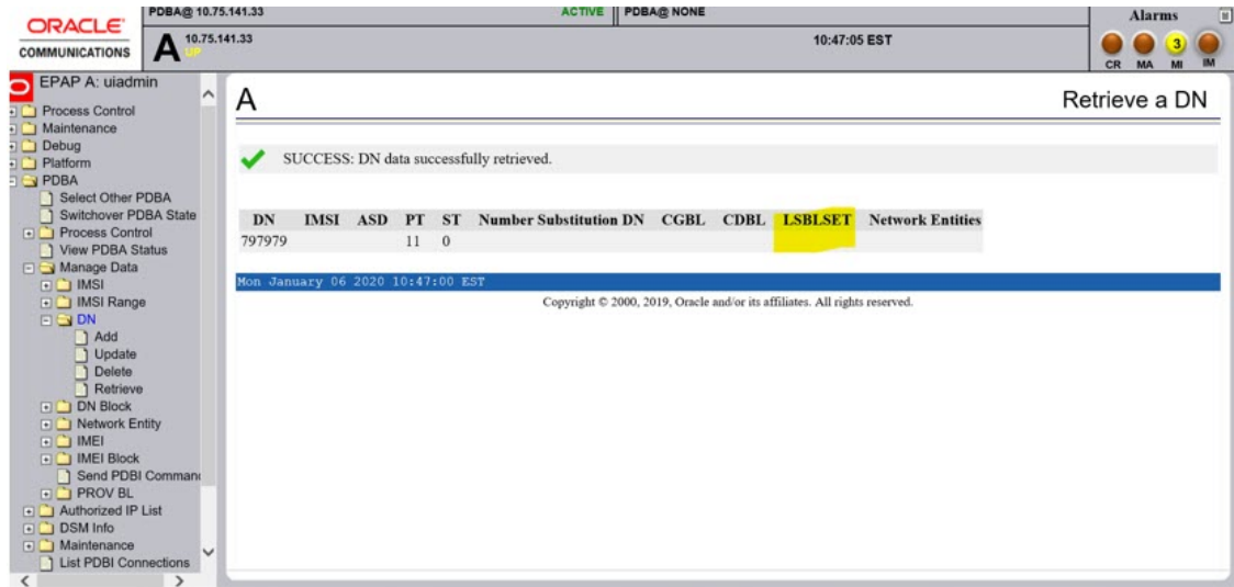
Figure 3-78 Retrieve a DN
