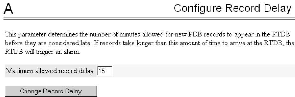
Figure 3-41 Configure Record Delay Screen
