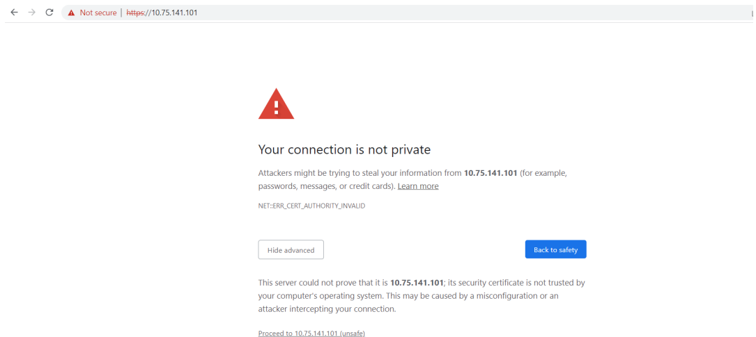
Figure 3-8 Security Certificate
