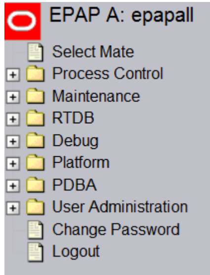
Figure 3-25 EPAP Menu
