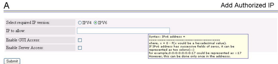
Figure 3-102 Add Authorized IP
