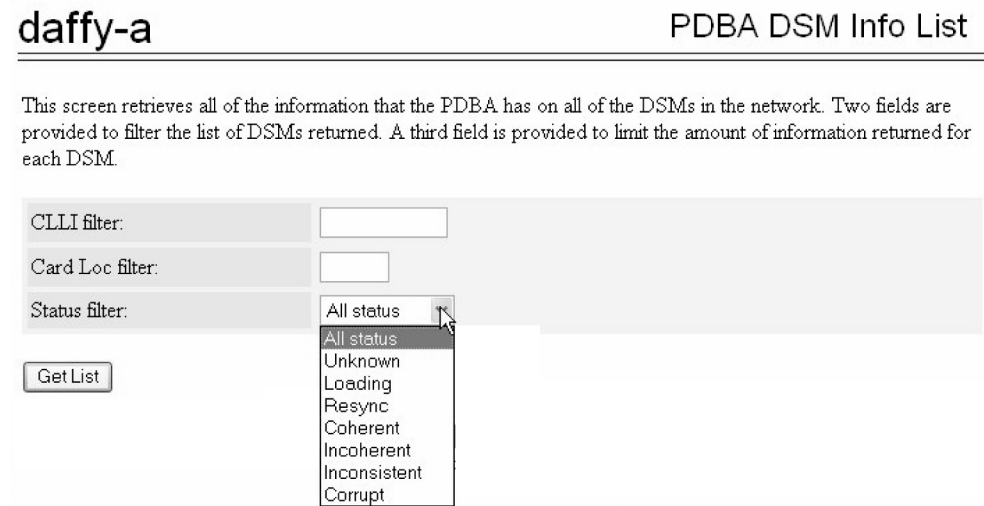
Figure 3-98 PDBA DSM Info List Screen (with Status filter pulldown)
