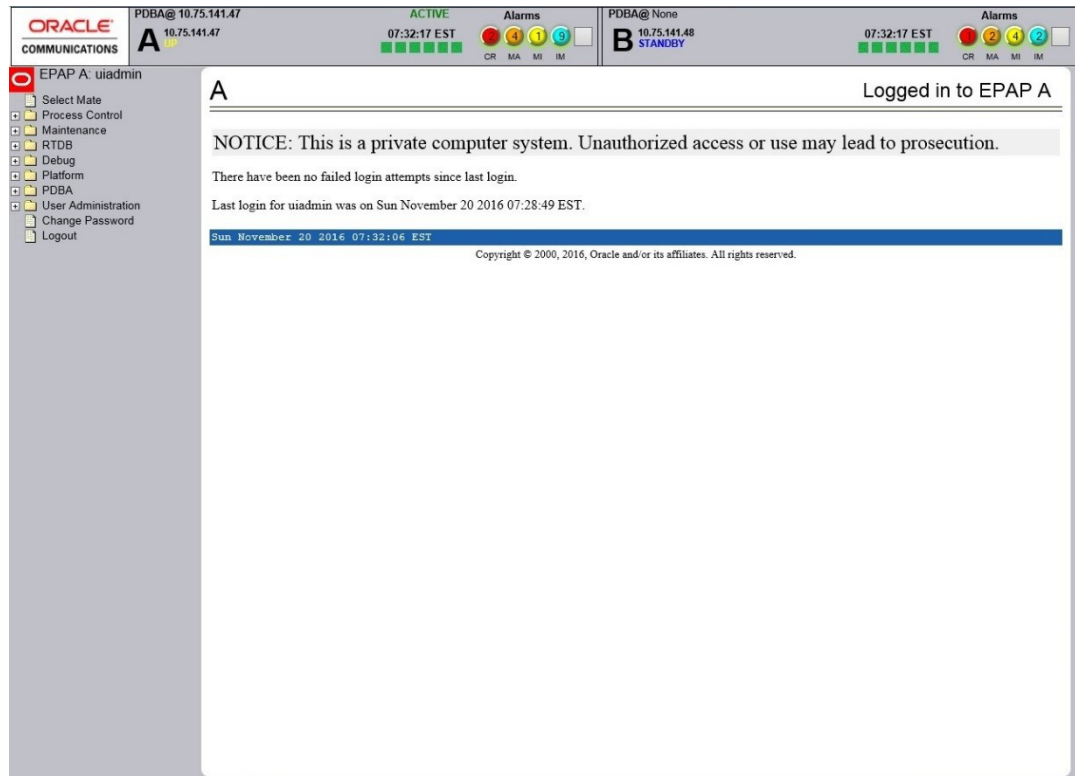
Figure 3-20 EPAP GUI
