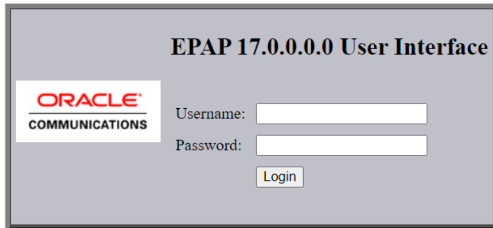
Figure 3-2 EPAP Login
