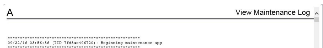
Figure 3-59 Log Viewer
