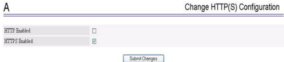
Figure 3-5 HTTPS Enabled
