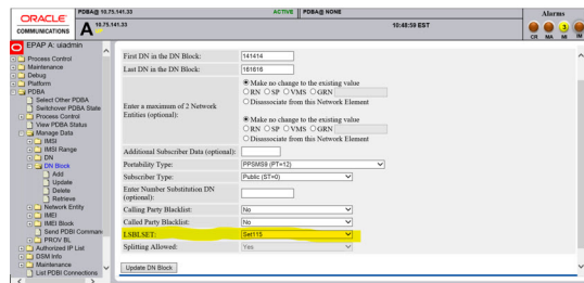
Figure 3-80 Update a DN Block Screen
