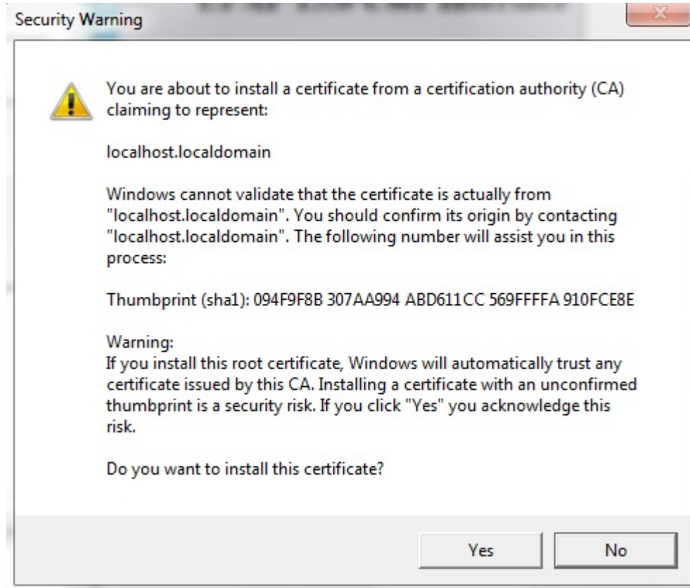
Figure 3-16 Security Warning
