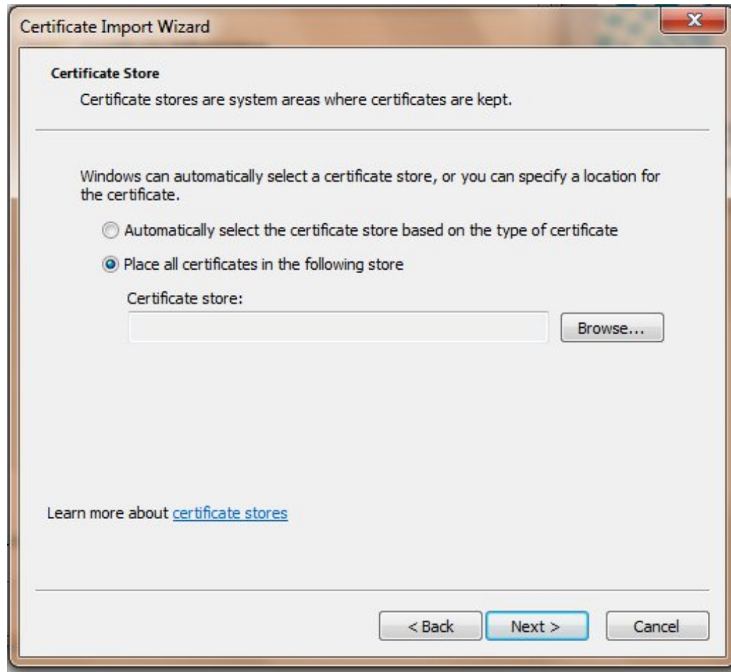
Figure 3-12 Certificate Store
