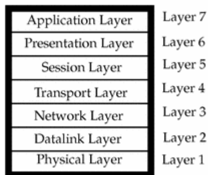
Figure 20-1 OSI Model
