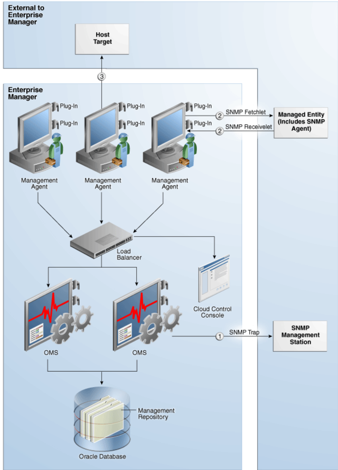
Figure 1 How Enterprise Manager Supports SNMP
