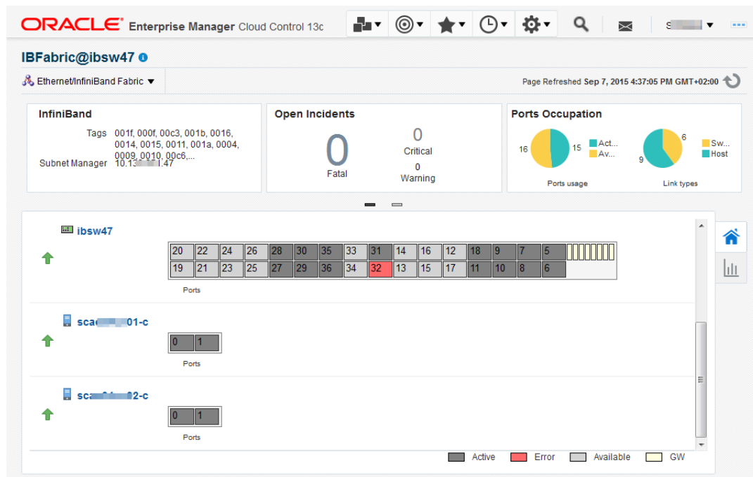
Figure 20-5 Fabric Landing Page
