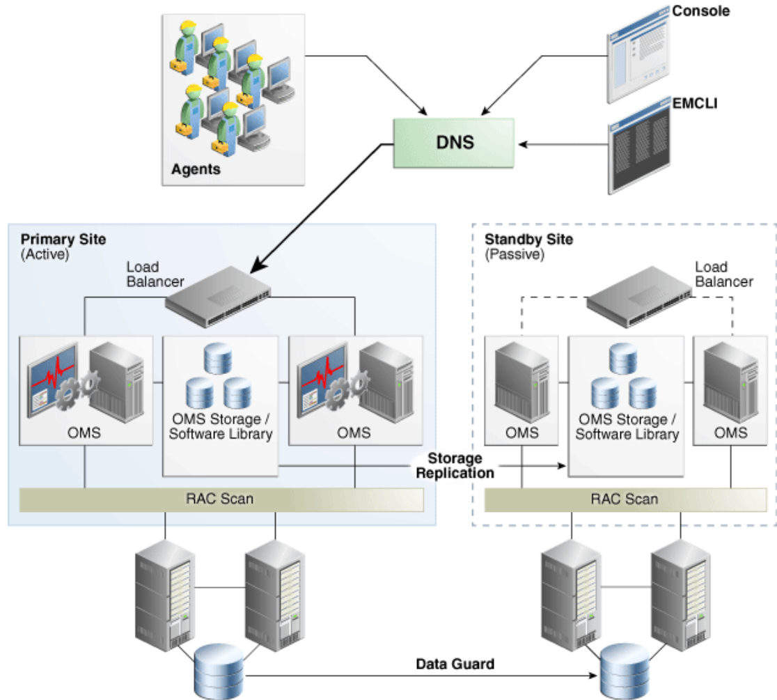
Figure 25-1 High Availability with Disaster Recovery Topology
