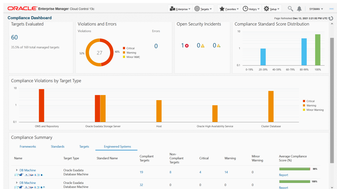
Figure 23-9 Compliance Dashboard with Engineered Systems Tab
