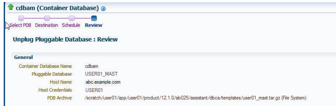
Figure 13-41 Unplugging a Pluggable Database: Review Page
