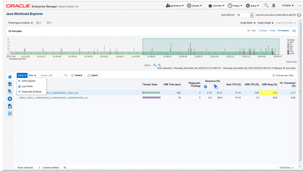
Figure 19-8 Overview Tab
