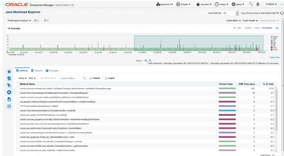
Figure 19-12 Code Tab
