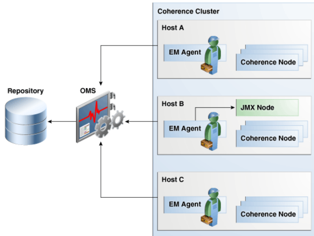
Figure 22-1 Coherence Cluster Configuration (Standalone Coherence Cluster)
