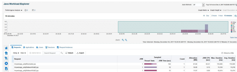
Figure 19-9 Request Tab
