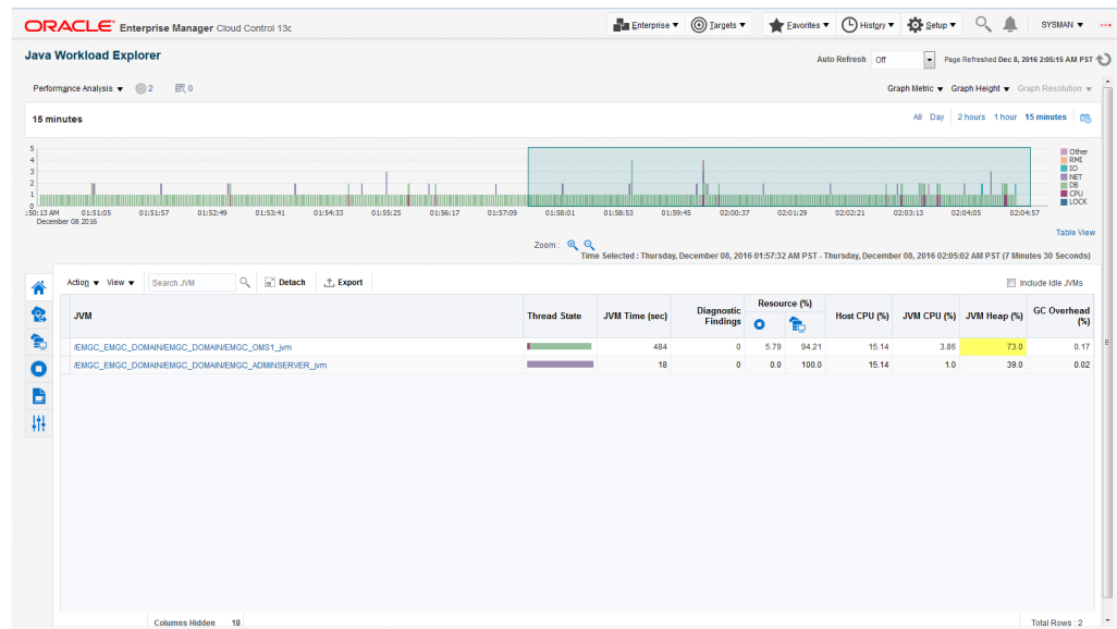
Figure 19-4 Performance Analysis
