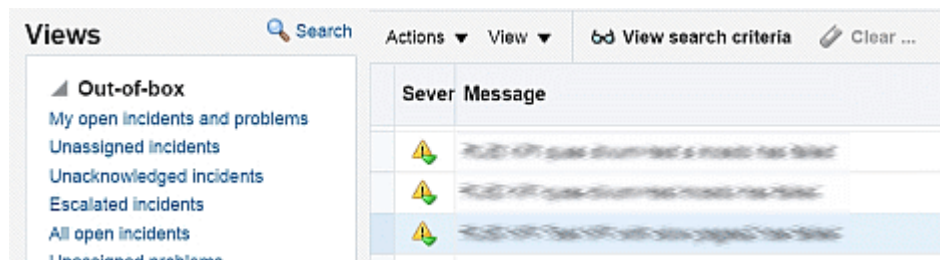
Figure 15-25 Incident Manager
