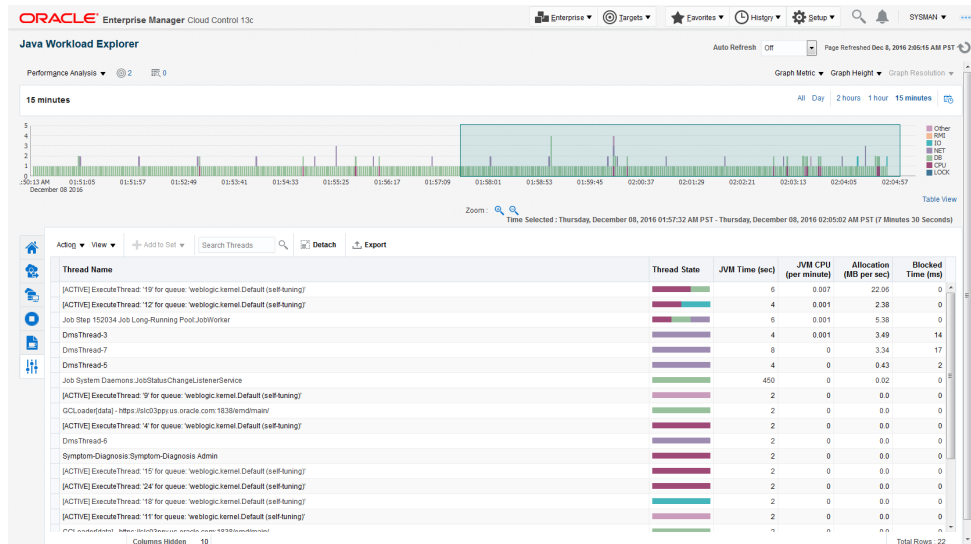
Figure 19-13 Threads Tab
