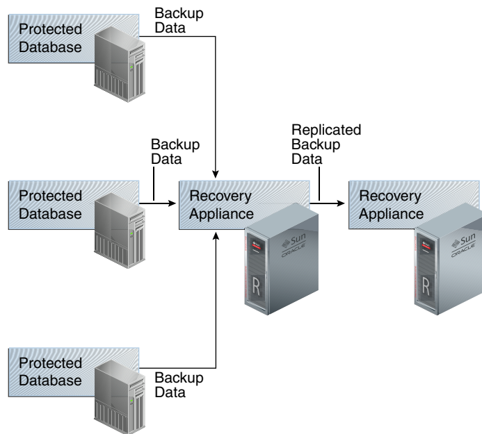
Figure 14-1 Simple Replication Topology
