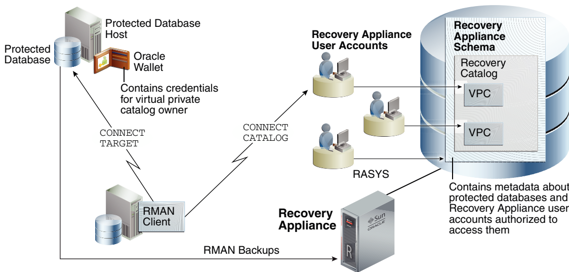
Figure 8-1 Protected Database Access
