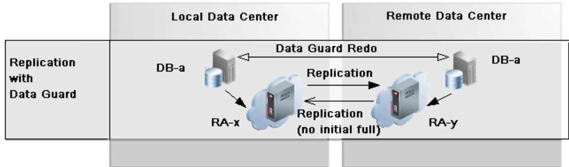
Figure 15-2 Backup Anywhere Mode for Data Guard
