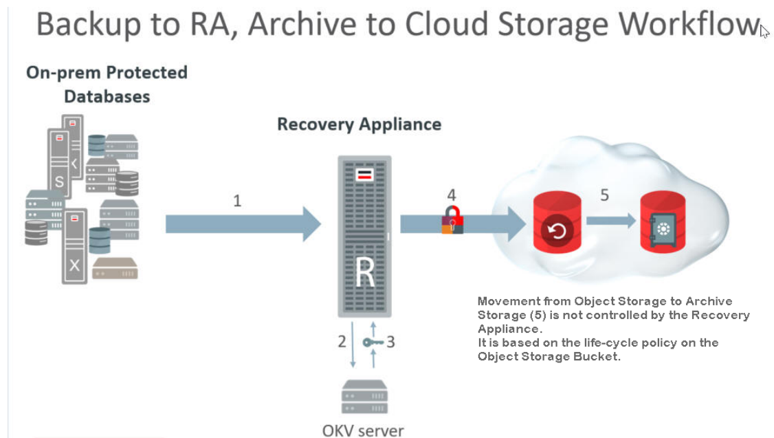
Figure 10-1 Flow for Backups to Cloud Storage
