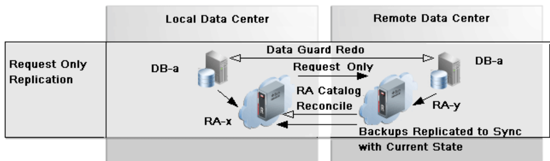
Figure 15-3 Replication Request Mode of Backup Anywhere
