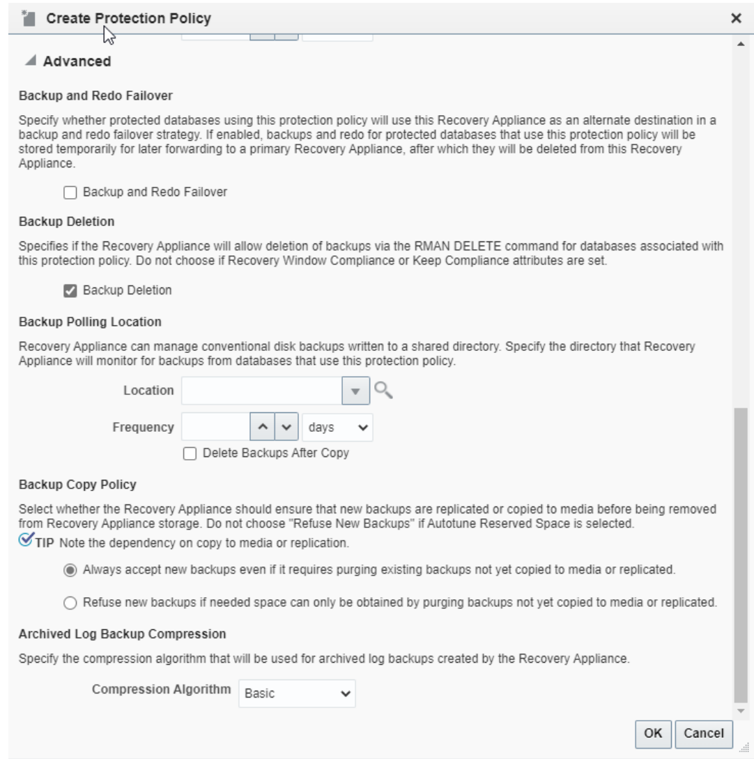
Figure 14-8 Protection Policy Advanced Parameters
