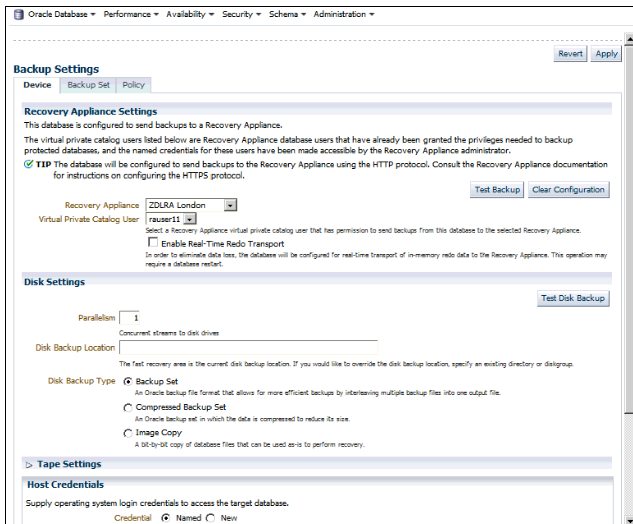
Figure 4-2 Backup Settings Page for Protected Databases
