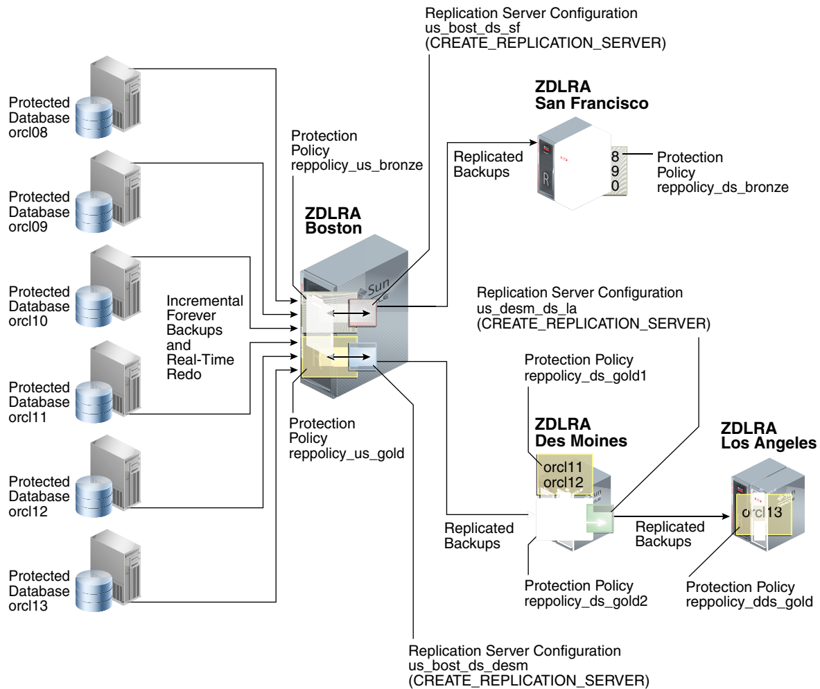
Figure 9-5 Cascaded Replication, with Different Protection Policies on Each Recovery Appliance
