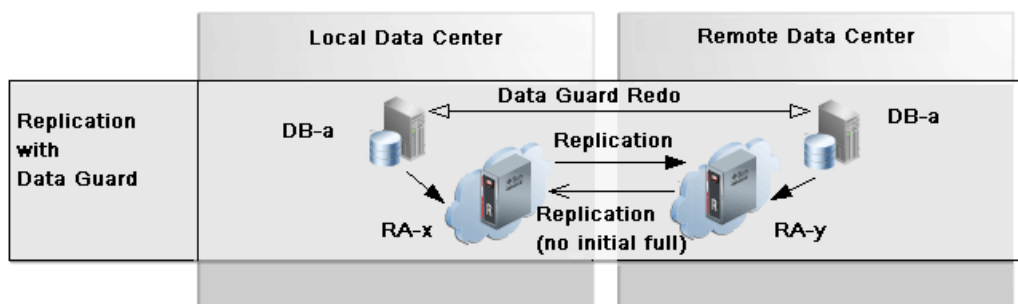
Figure 10-2 Backup Anywhere Mode for Data Guard
