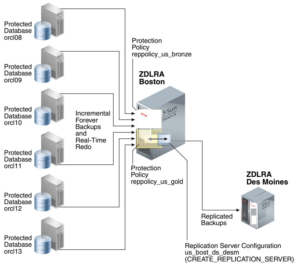
Figure 9-2 Databases Replicating to One Recovery Appliance
