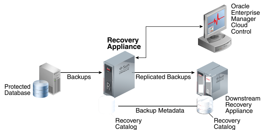
Figure 1-6 One-Way Replication
