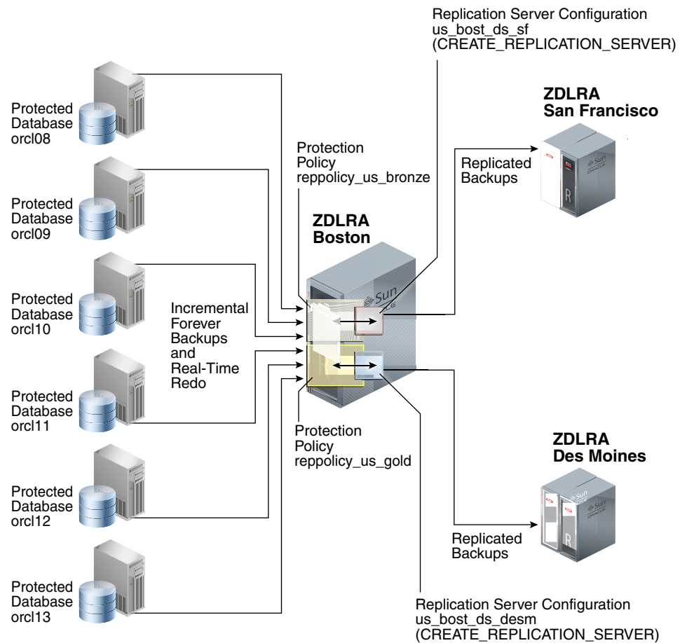
Figure 9-3 Databases Replicated to Multiple Recovery Appliances
