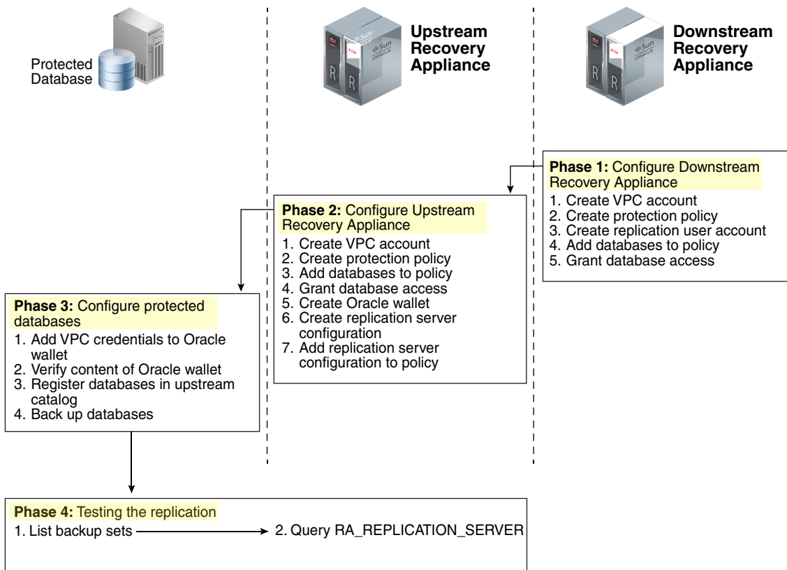
Figure 9-14 Overview of Manual Configuration for Replication
