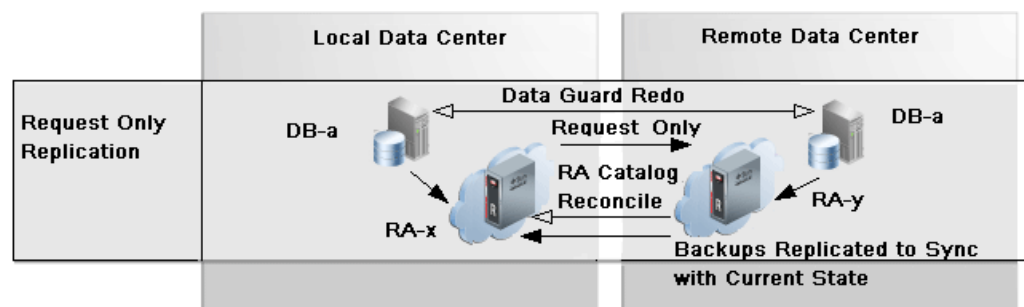
Figure 10-3 Replication Request Mode of Backup Anywhere
