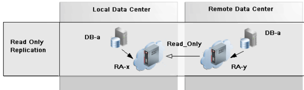
Figure 10-4 Read-Only Mode of Backup Anywhere
