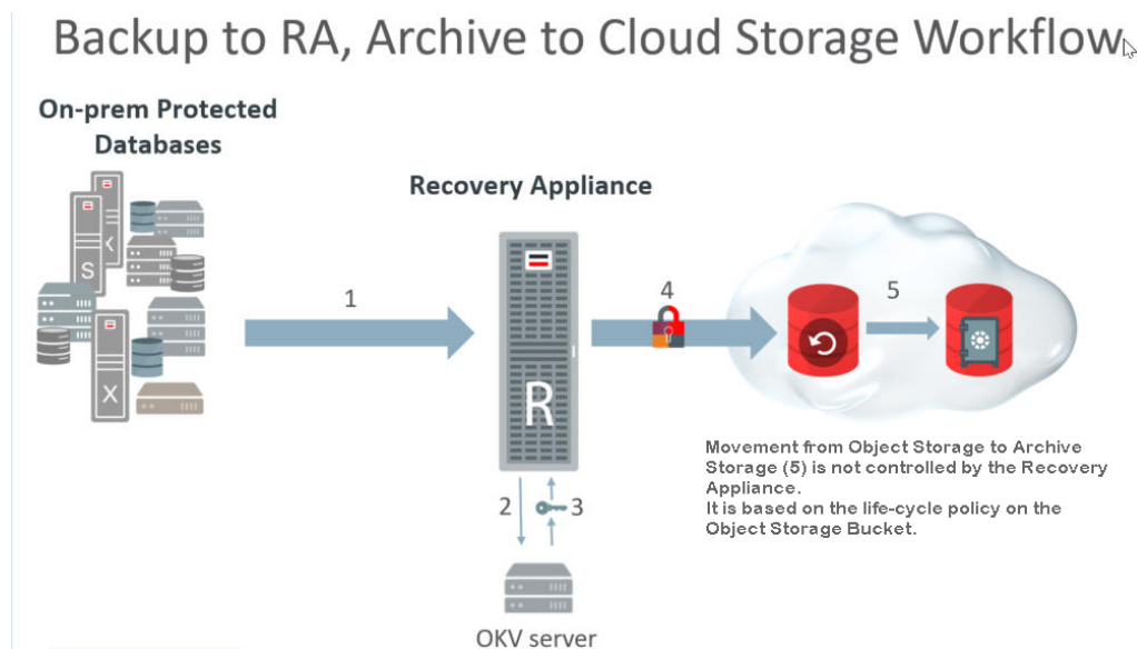
Figure 8-1 Flow for Backups to Cloud Storage
