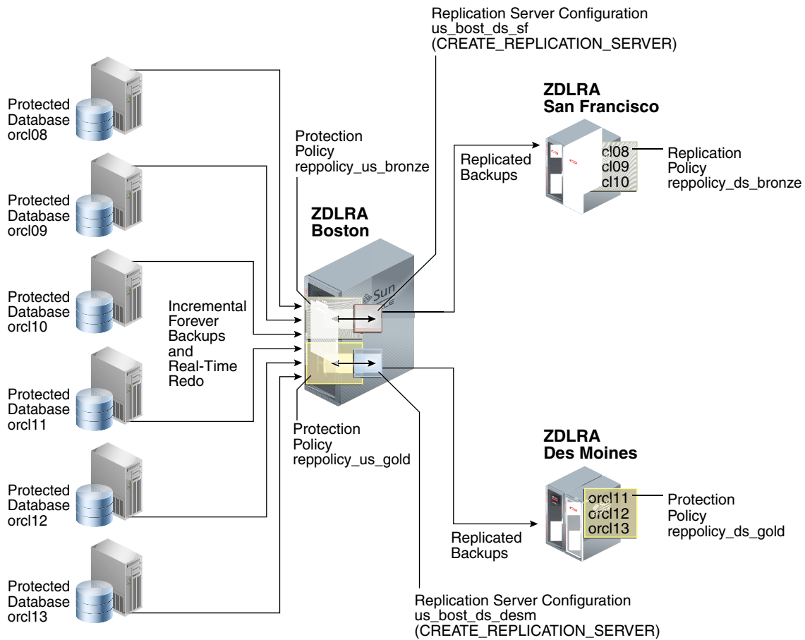
Figure 9-4 Different Protection Policies on Each Recovery Appliance
