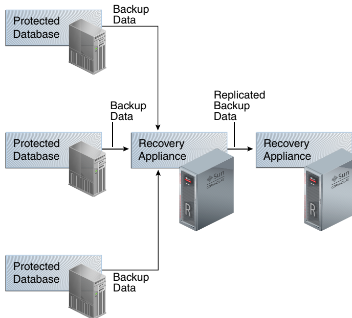
Figure 9-1 Simple Replication Topology
