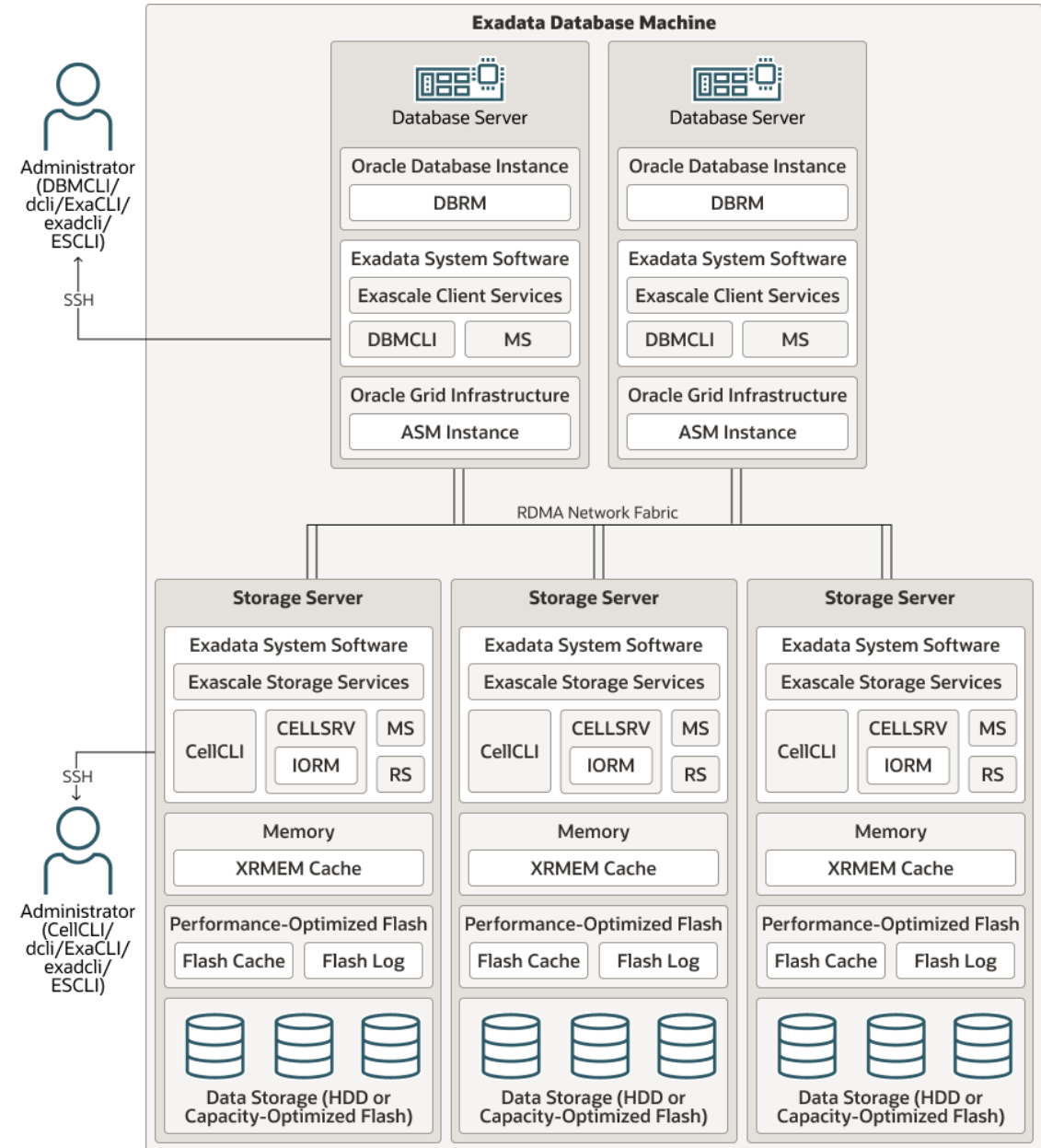
Figure 1-3 Software Components in Oracle Exadata
