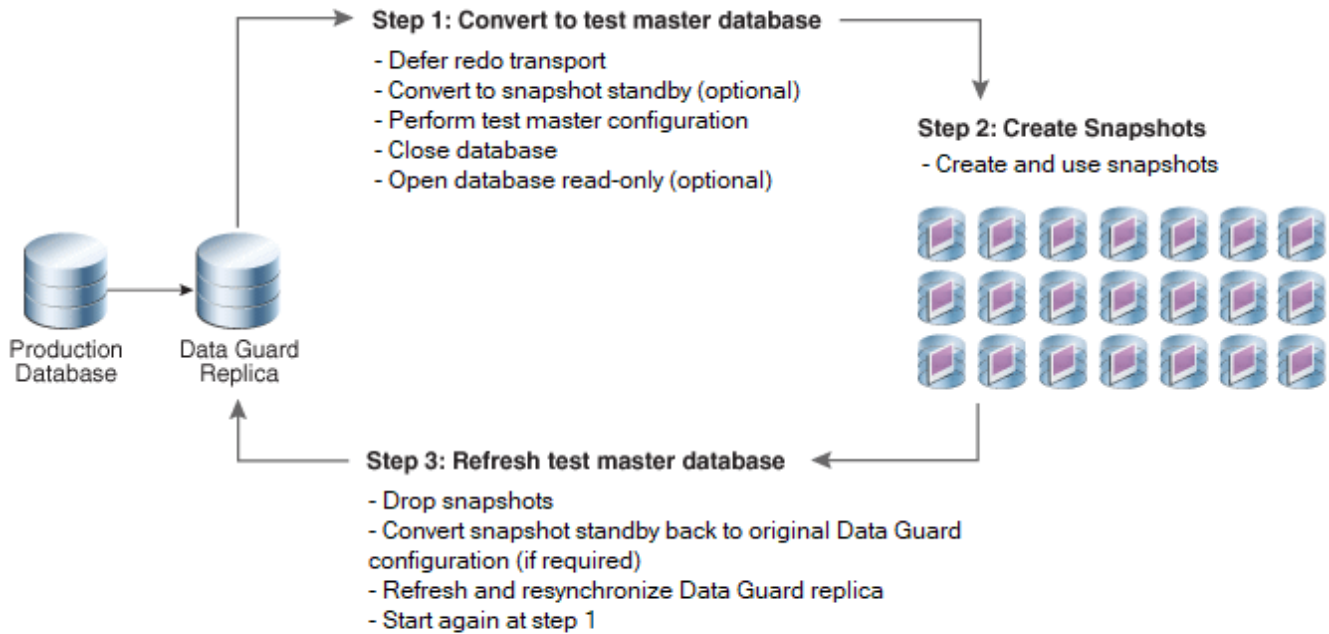
Figure 9-13 Lifecycle of Test Master and Snapshot Databases
