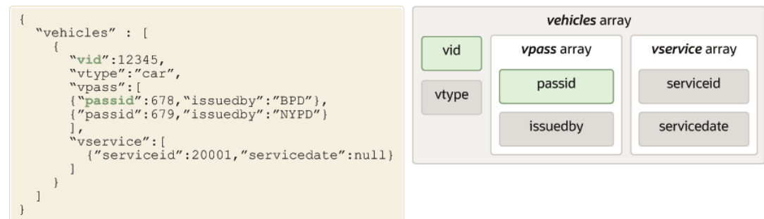
Figure 8-3 Composite Multikey Index
