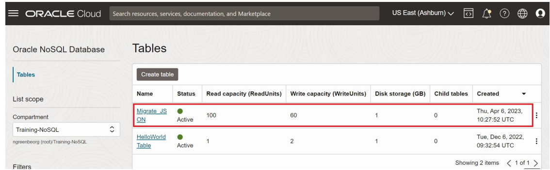
Figure 5-1 Oracle NoSQL Database Cloud Service Console Tables
