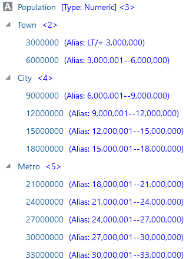
Figure 14-7 Numeric Attribute Dimension with Different-Sized Ranges
