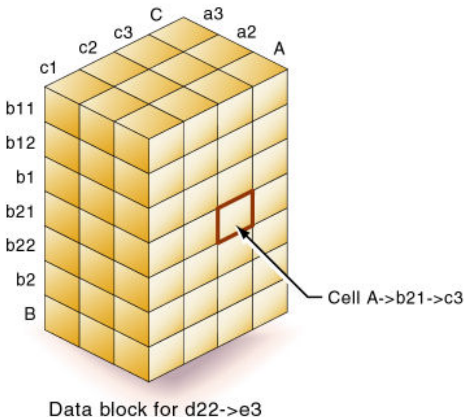
Figure 2-20 Data Block Representing Dense Dimensions for d22 \rightarrow e3
