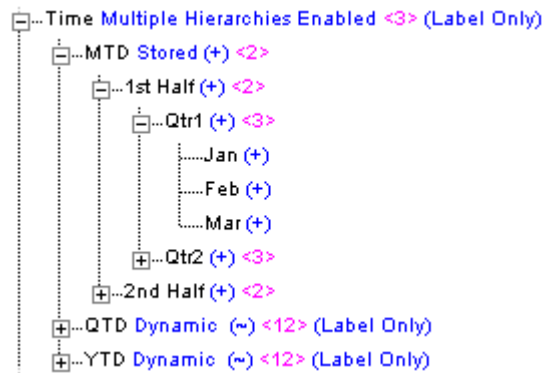
Figure 36-1 Outline Showing Multiple Hierarchies and Members on the Time Dimension
