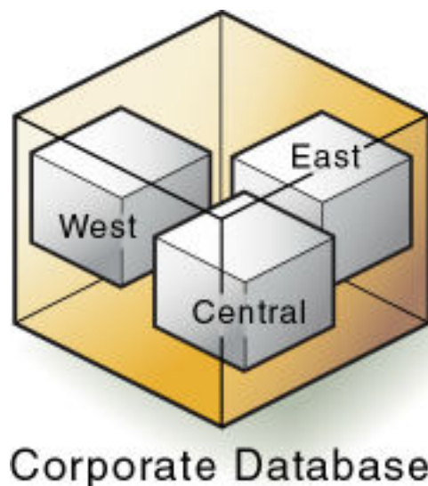
Figure 23-1 Calculating Partitions
