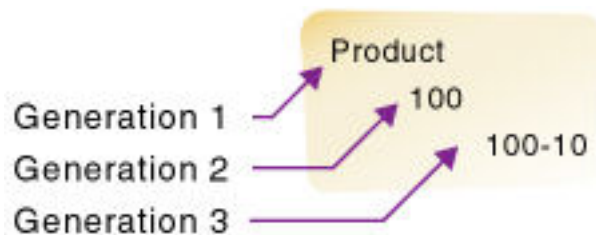
Figure 14-1 Generations
