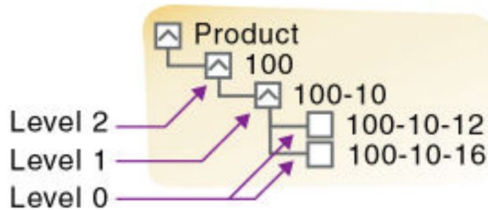
Figure 2-3 Levels
