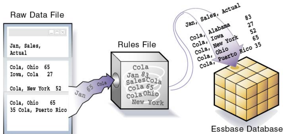
Figure 11-3 Loading Data Through Load Rules
