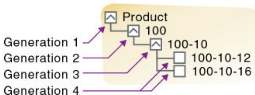
Figure 2-2 Generations
