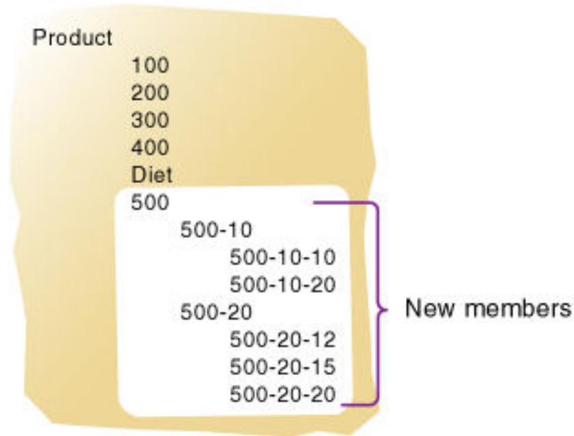
Figure 14-2 Generation References
