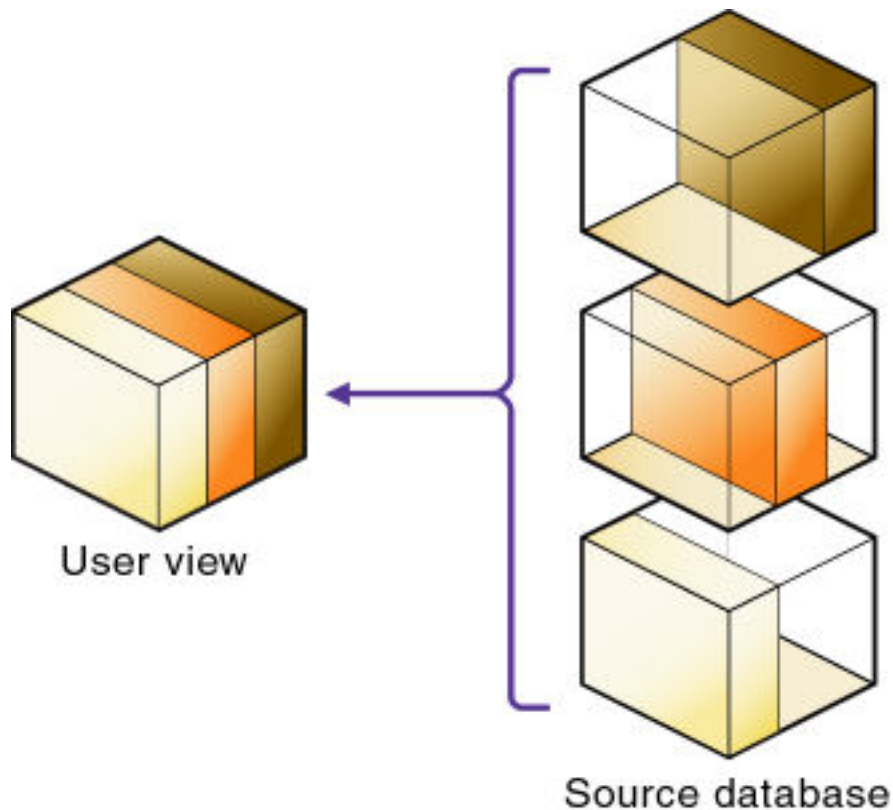
Figure 9-5 Transparent Partitions
