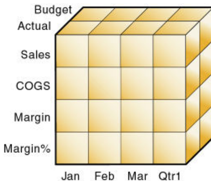
Figure 2-14 Three-Dimensional Database
