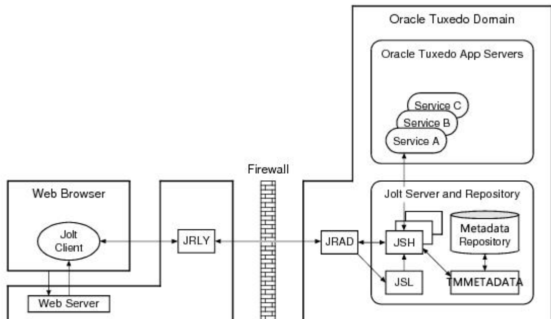
Figure 9-3 Oracle Jolt Internet Relay Connection Path
