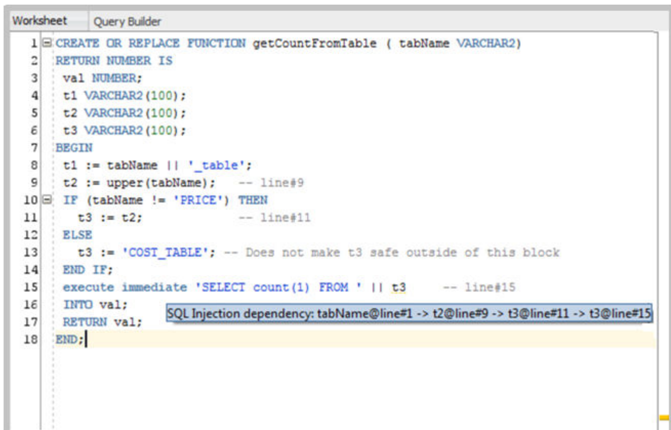
Figure 2-2 SQL Injection Vulnerability Warning in Code Editor
