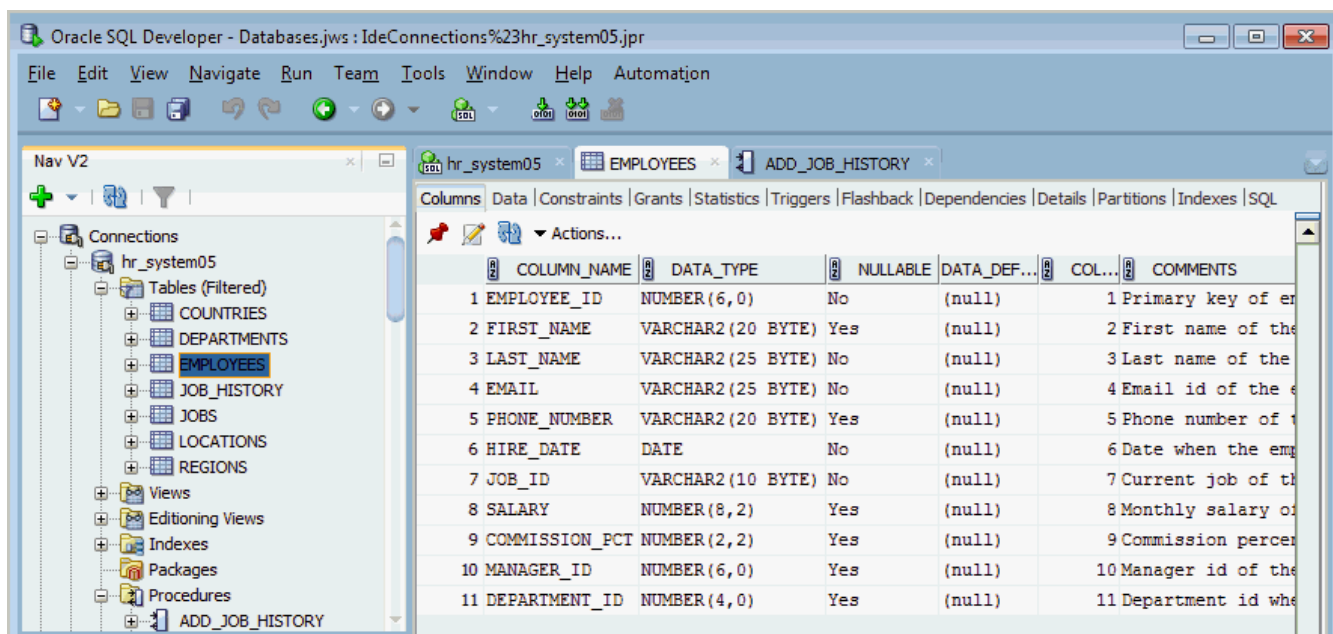
Figure 2-1 SQL Developer Main Window
