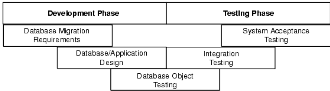
Figure 3-1 V-model with a Database Migration
