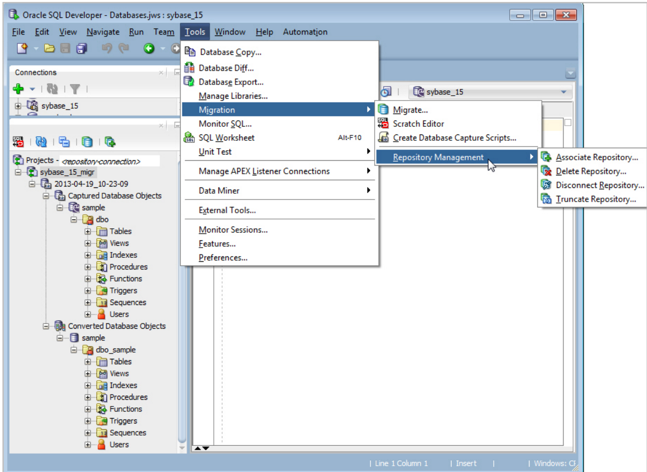
Figure 3-2 Main Window for a Database Migration
