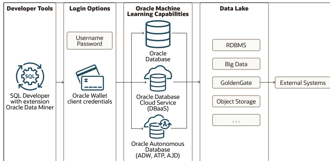
Figure 1-2 Oracle Data Miner Architecture
