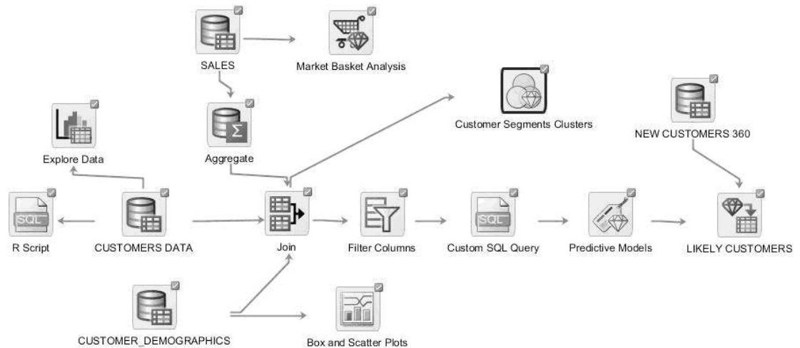
Figure 1-1 Sample Data Miner Workflow
