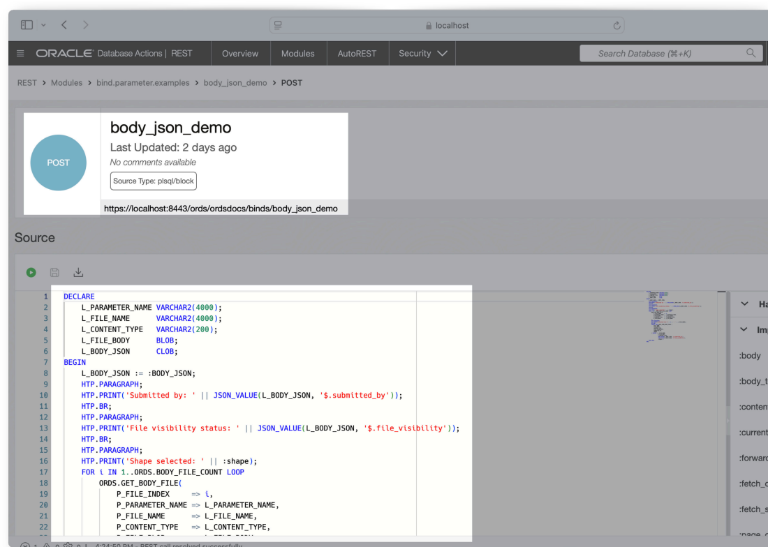
Figure 3-2 Creating an ORDS Endpoint
