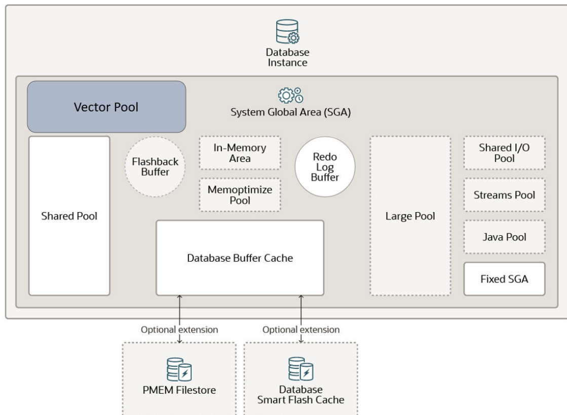
Figure 6-1 Vector Pool
