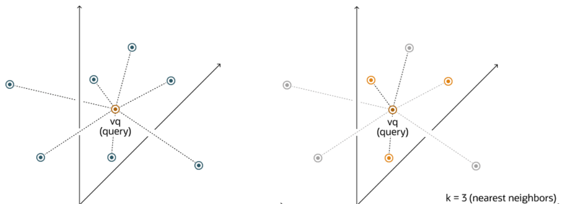
Figure 8-1 Exact Search
