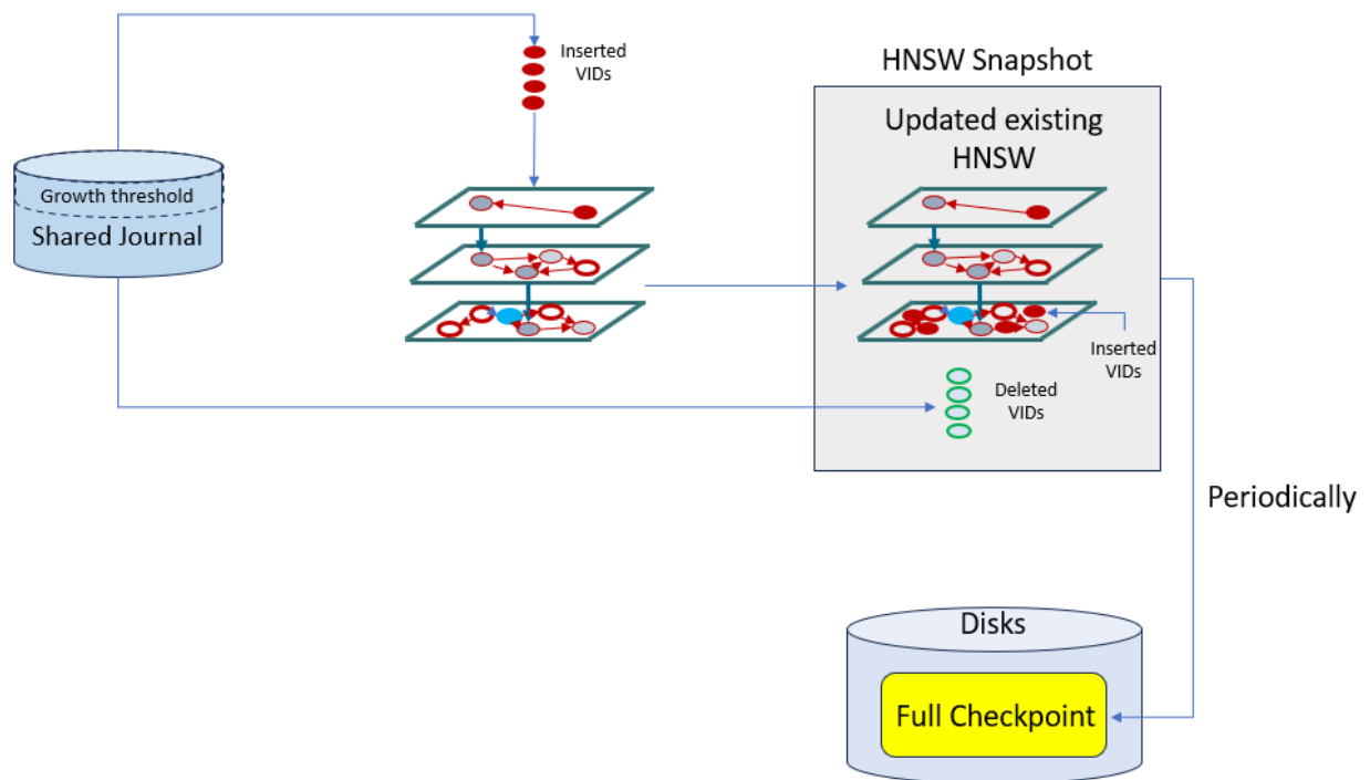
Figure 6-6 HNSW Snapshots
