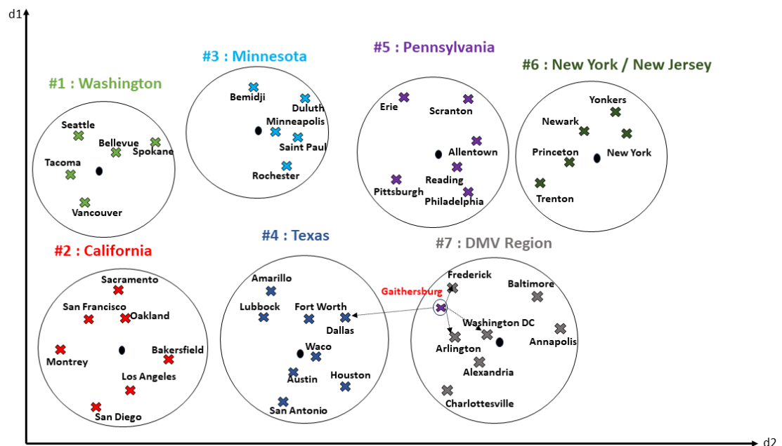
Figure 6-17 Similarity Search After Index Reorganization
