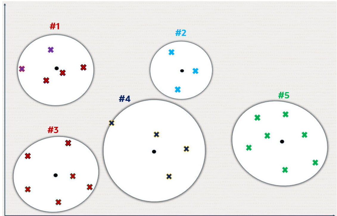
Figure 6-7 Inverted File Flat Index Using 2D
