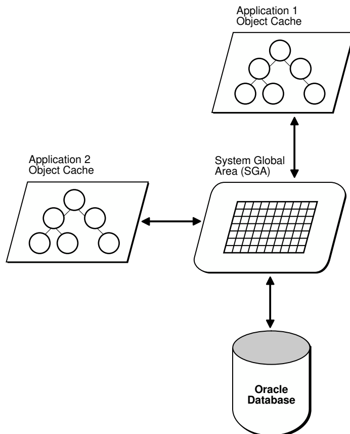
Figure 21-1 Object Cache
