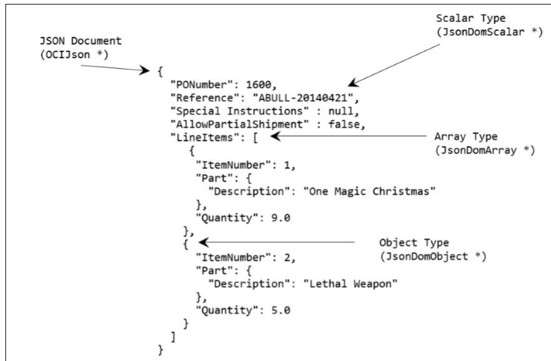
Figure 23-1 Sample JSON Document
