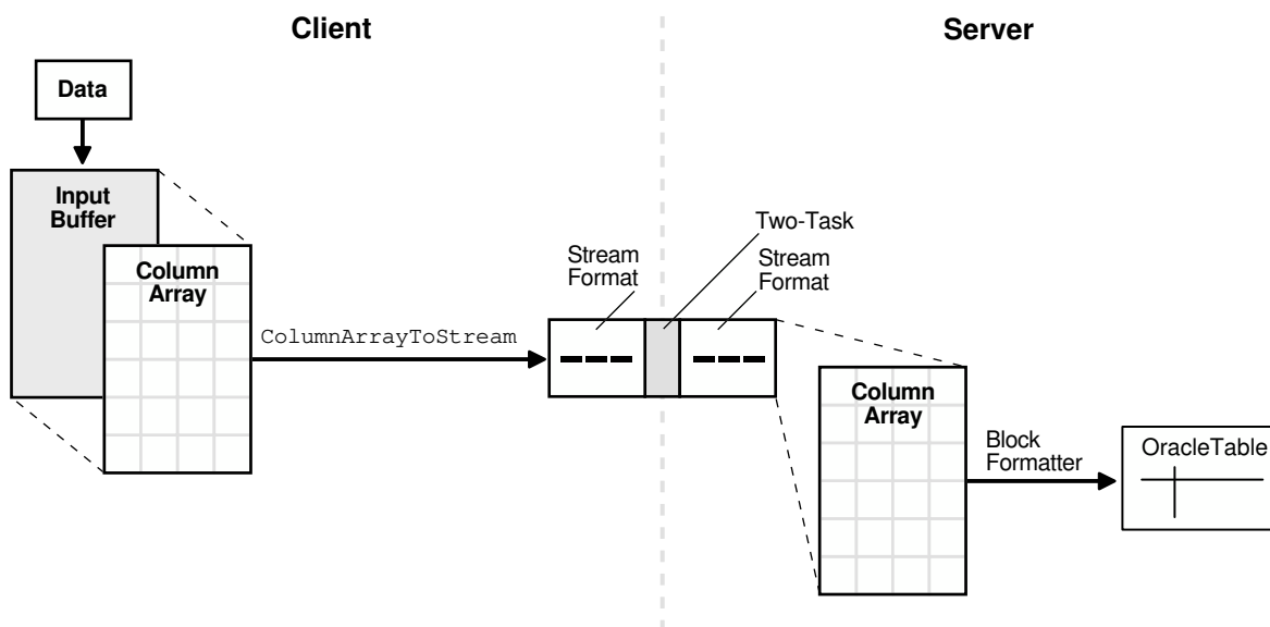
Figure 20-1 Direct Path Loading
