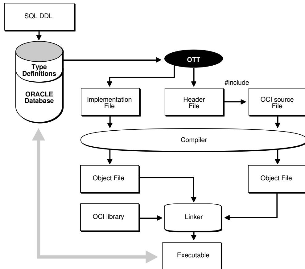
Figure 26-1 Using OTT with OCI
