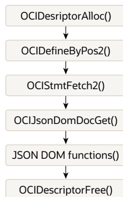
Figure 23-3 Calling Sequence for Reading JSON Data
