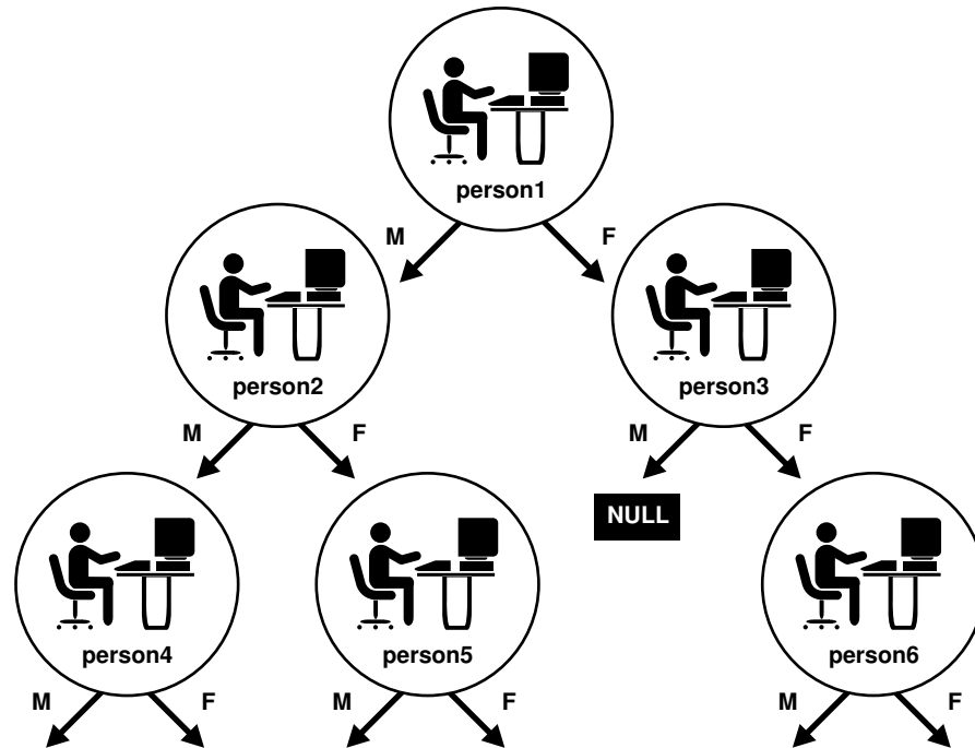
Figure 21-2 Object Graph of person_t Instances
