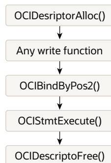
Figure 23-2 Calling Sequence for Writing JSON Data
