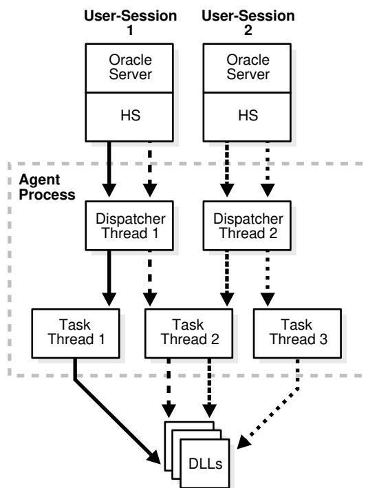
Figure F-1 Multithreaded extproc Agent Architecture
