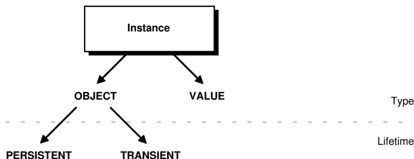
Figure 29-1 Classification of Instances by Type and Lifetime
