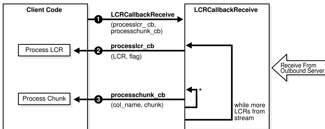
Figure 37-2 Execution Flow of the OCIXStreamOutLCRCallbackReceive() Function
