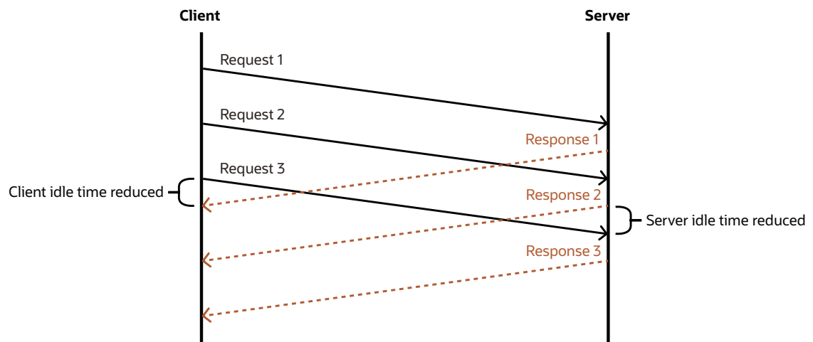
Figure 22-4 Pipelining Functionality
