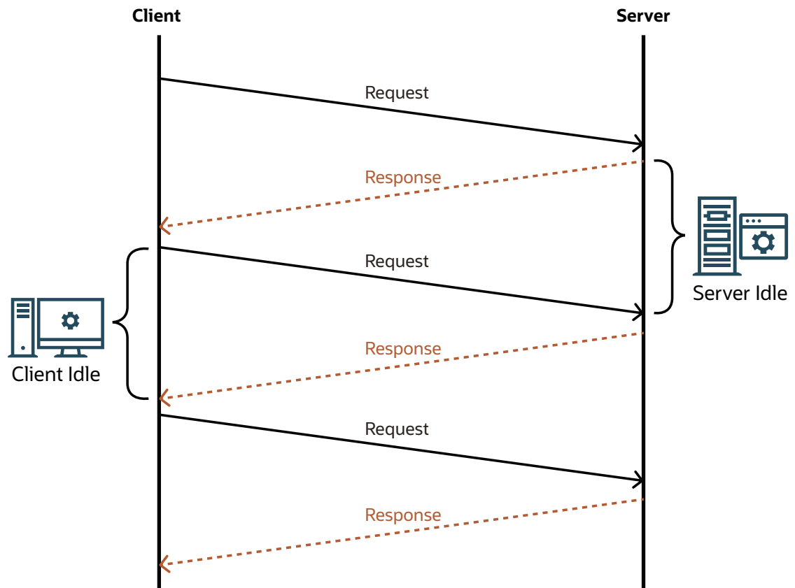
Figure 22-1 Blocking Functionality
