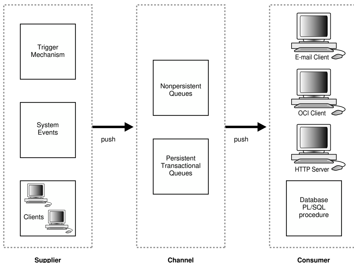
Figure 12-1 Publish-Subscribe Model
