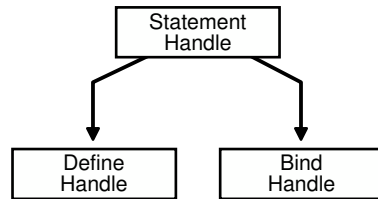
Figure 3-3 Statement Handles
