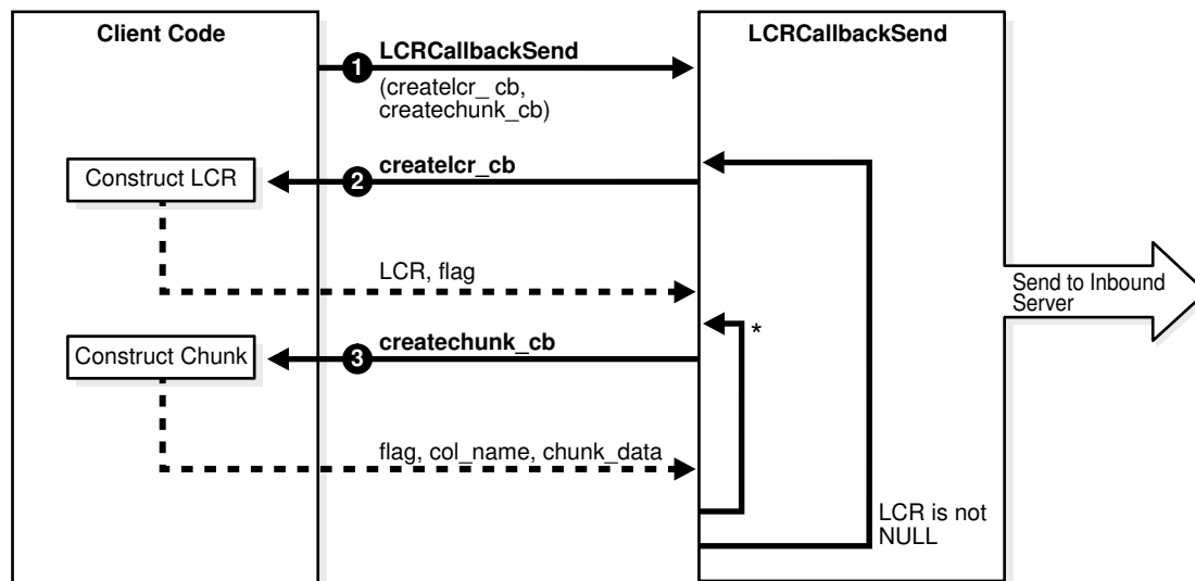
Figure 37-1 Execution Flow of the OCIXStreamInLCRCallbackSend() Function
