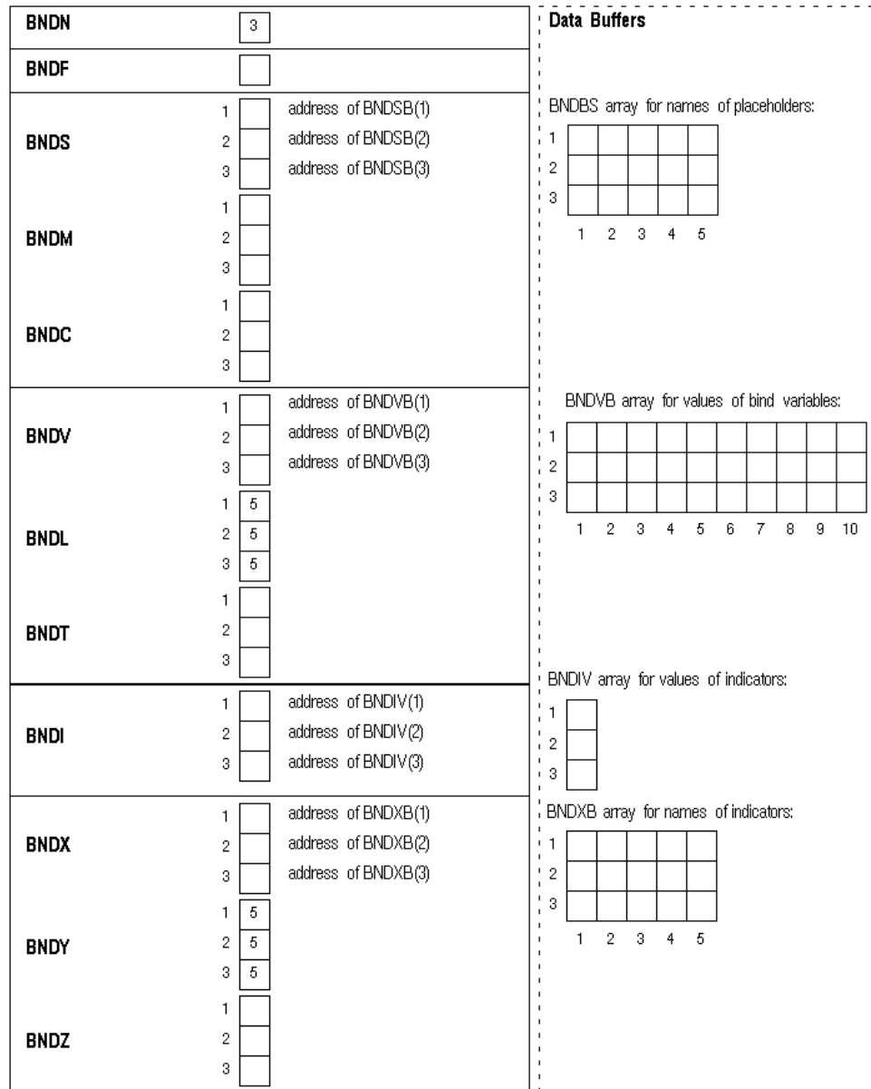
Figure 4-4 Initialized Bind Descriptor
