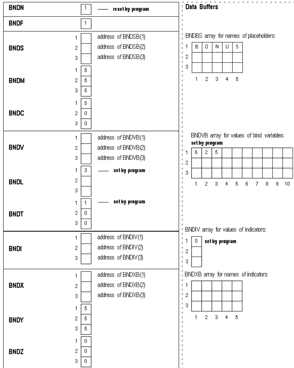
Figure 4-6 Bind Descriptor After Assigning Values
