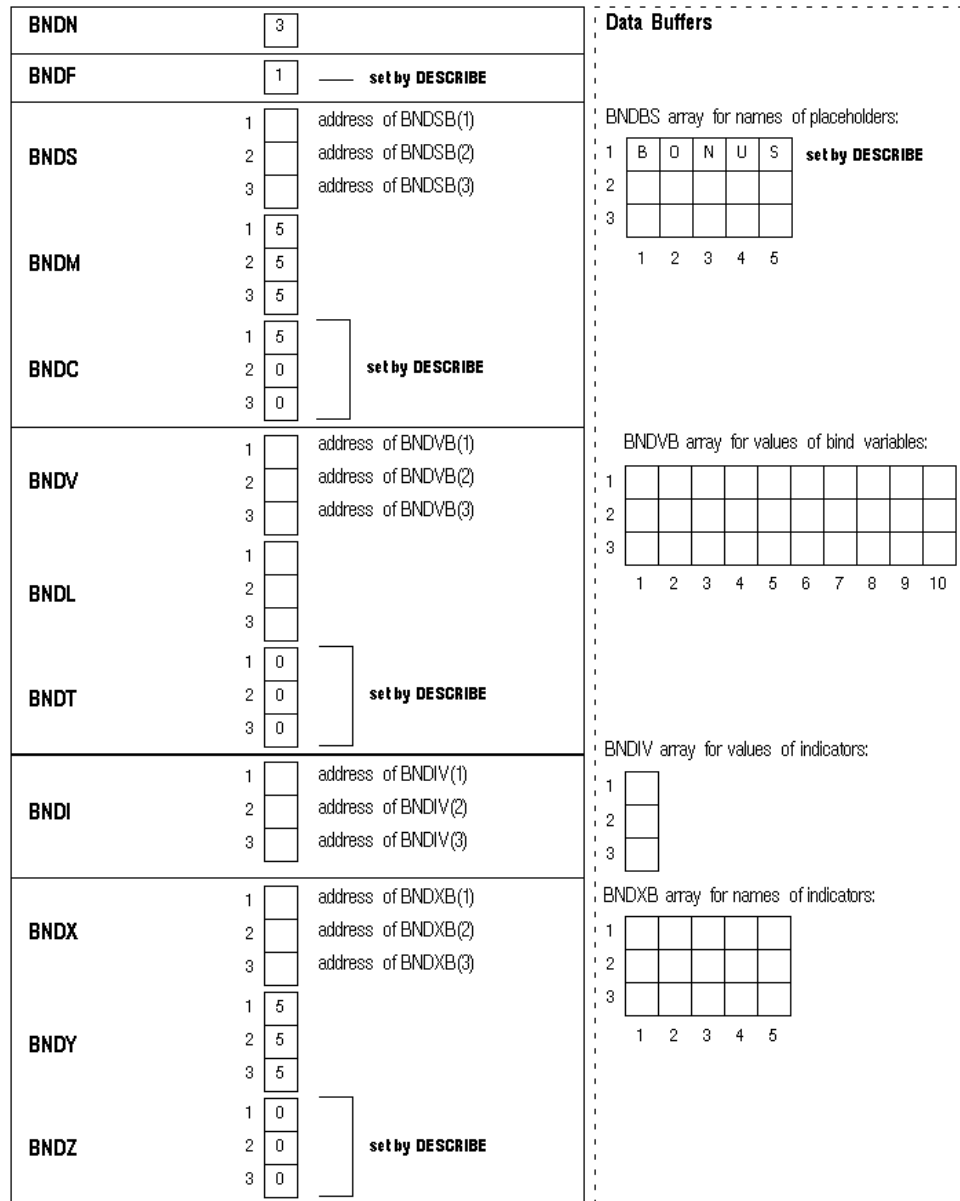
Figure 4-5 Bind Descriptor after the DESCRIBE
