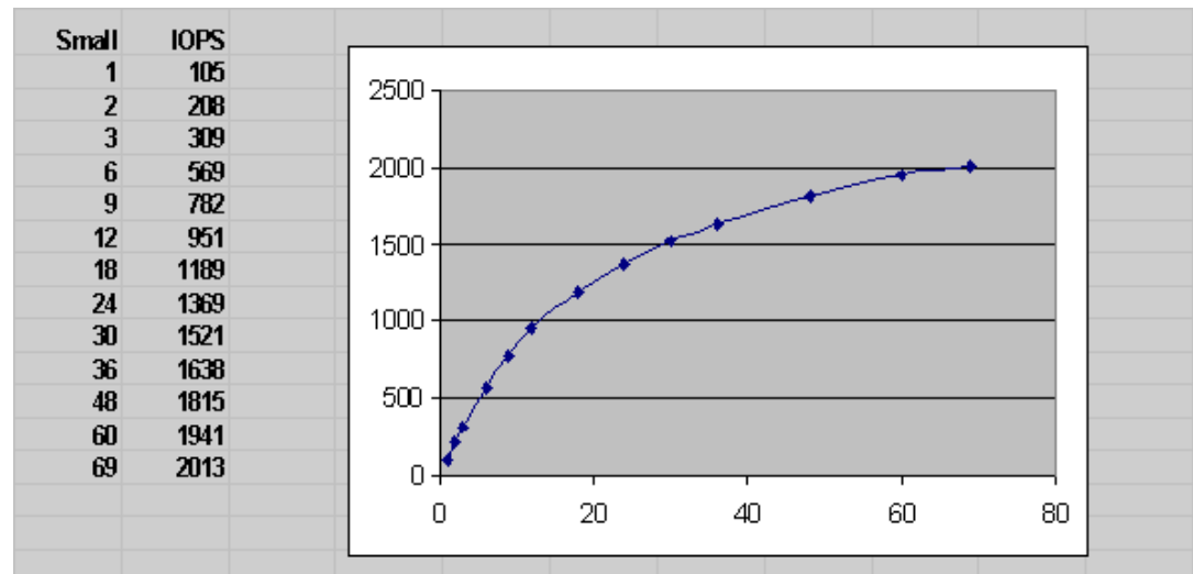
Figure 18-3 I/O Throughput at Different Small I/O Load Levels
