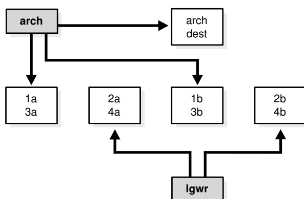
Figure 18-1 Distributing Redo Members Across Disks
