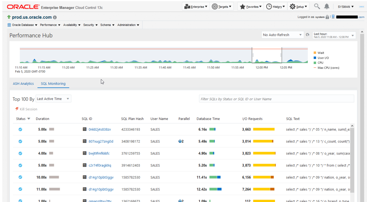
Figure 5-1 Monitored SQL Executions Page
