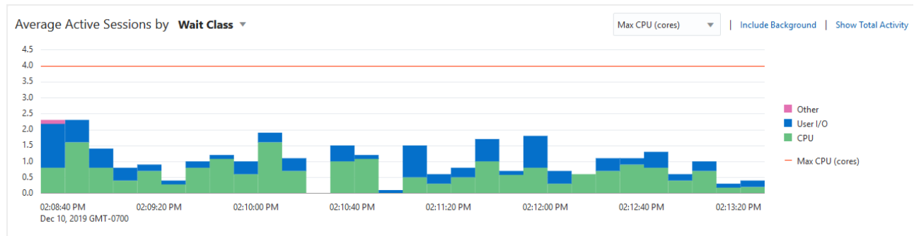
Figure 4-1 Average Active Sessions by Wait Class
