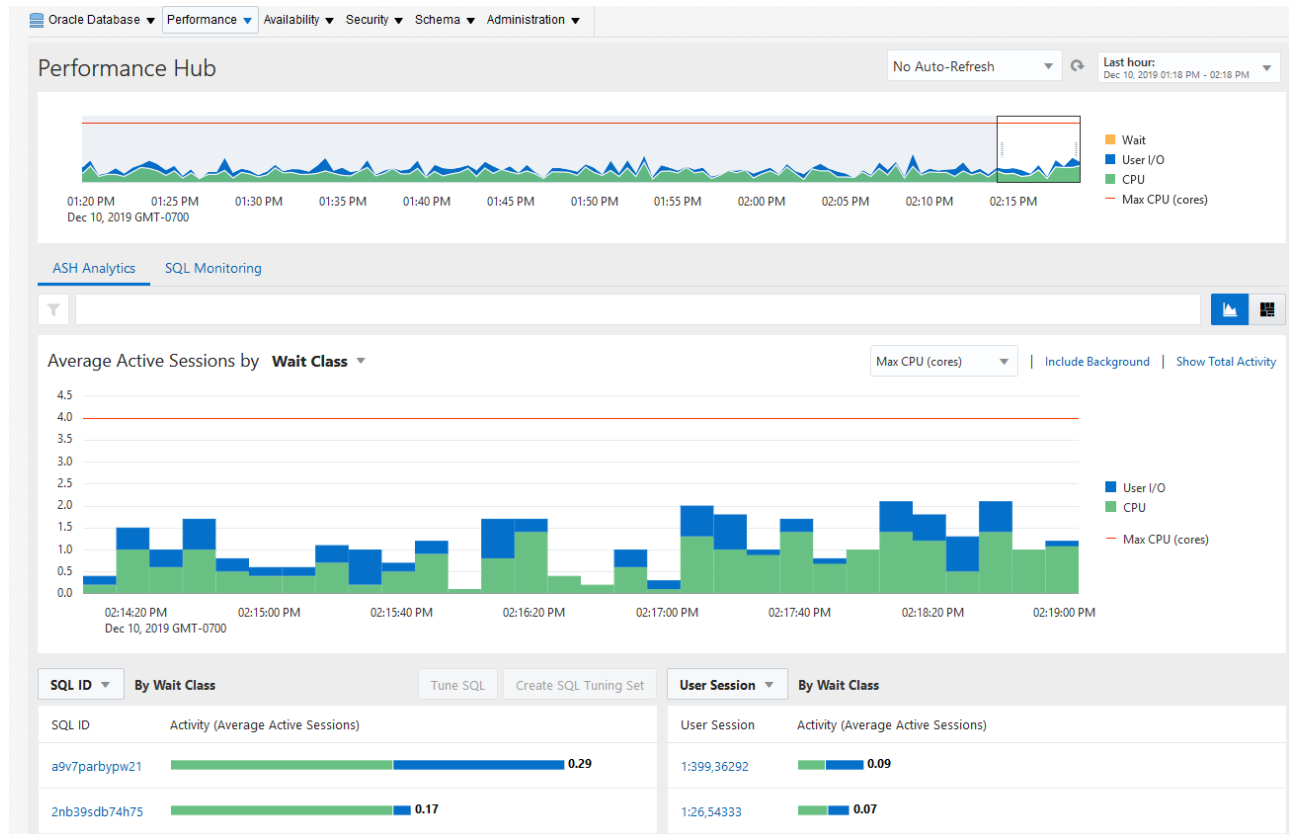
Figure 4-10 ASH Analytics Page
