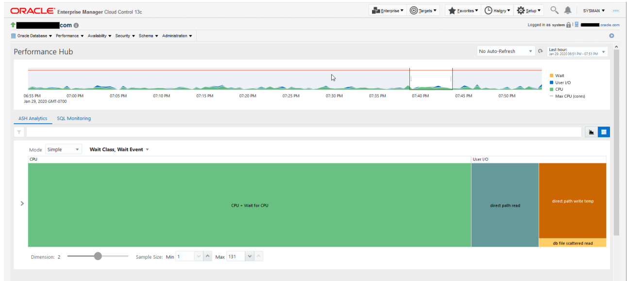
Figure 4-12 Load Map on the ASH Analytics Page
