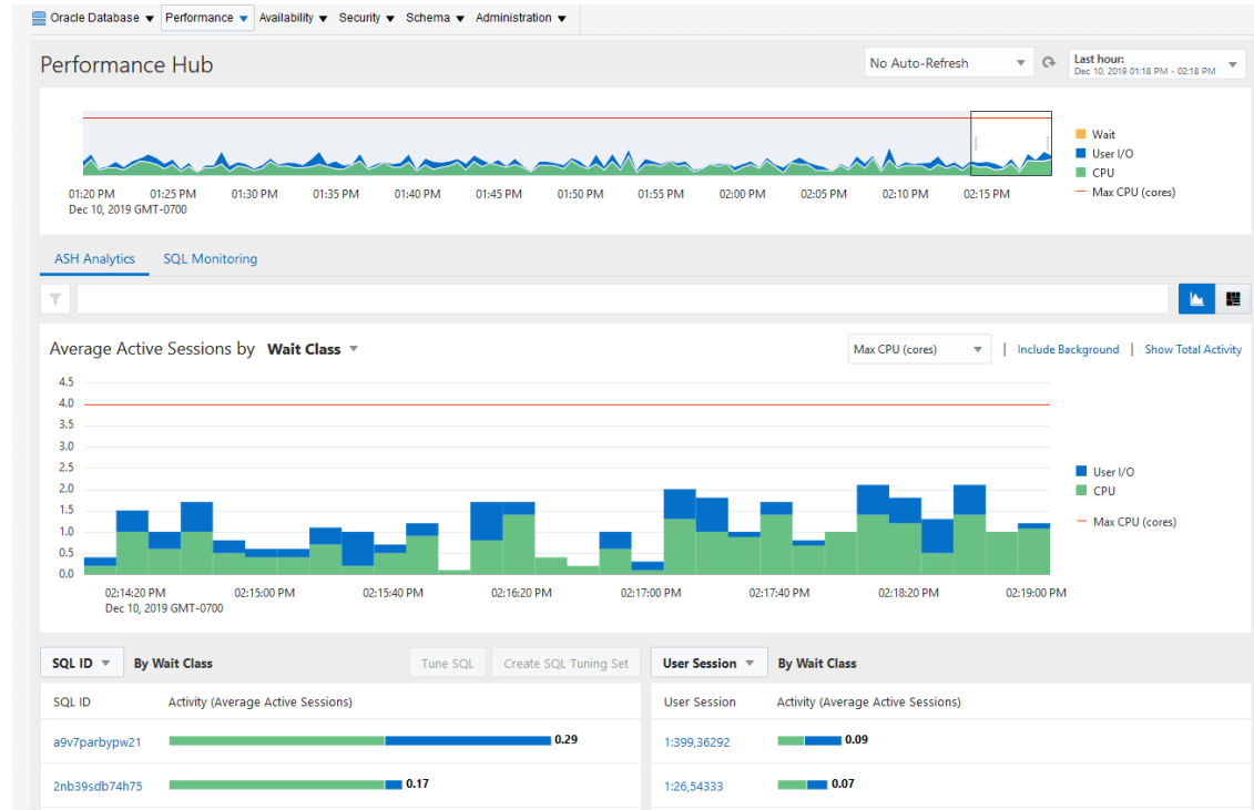
Figure 11-1 Top Activity Page
