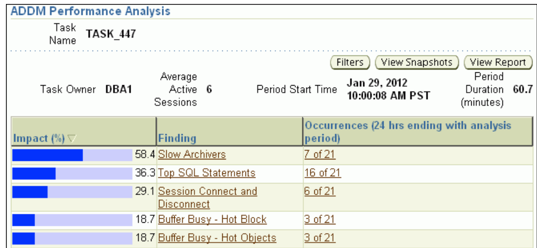
Figure 7-1 Analyzing Historical Database Performance
