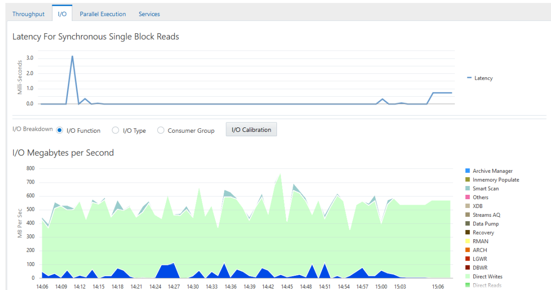
Figure 4-5 Performance Monitoring I/O by Type
