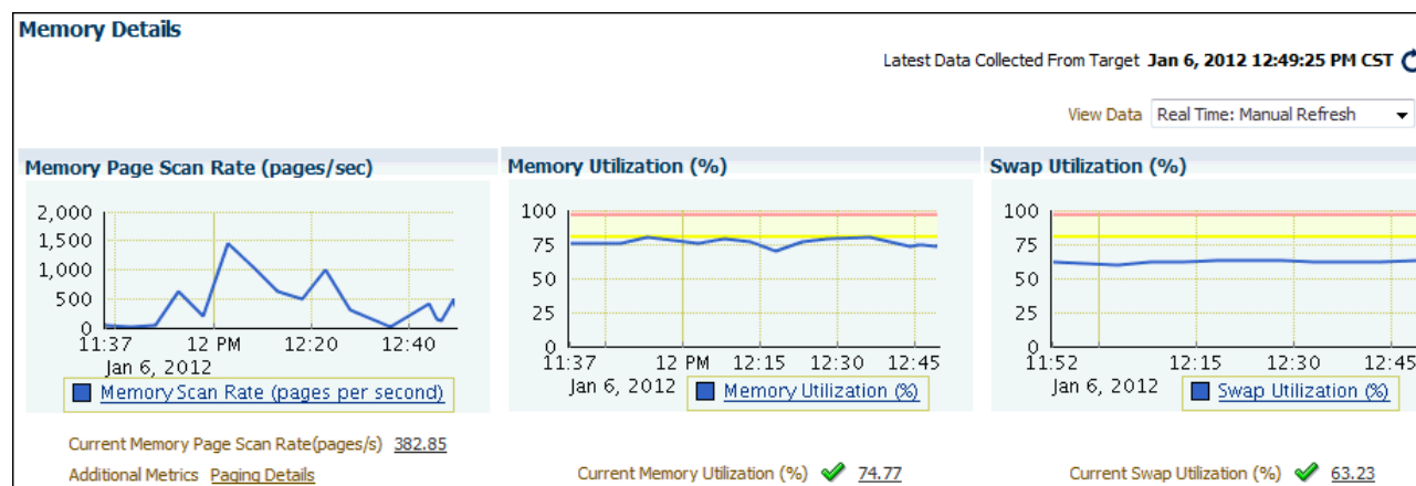
Figure 4-8 Memory Details Page
