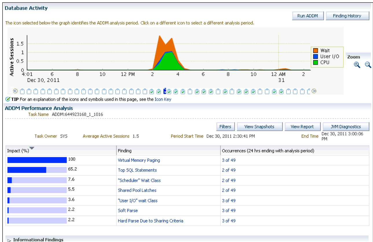
Figure 3-1 The Automatic Database Diagnostic Monitor Page
