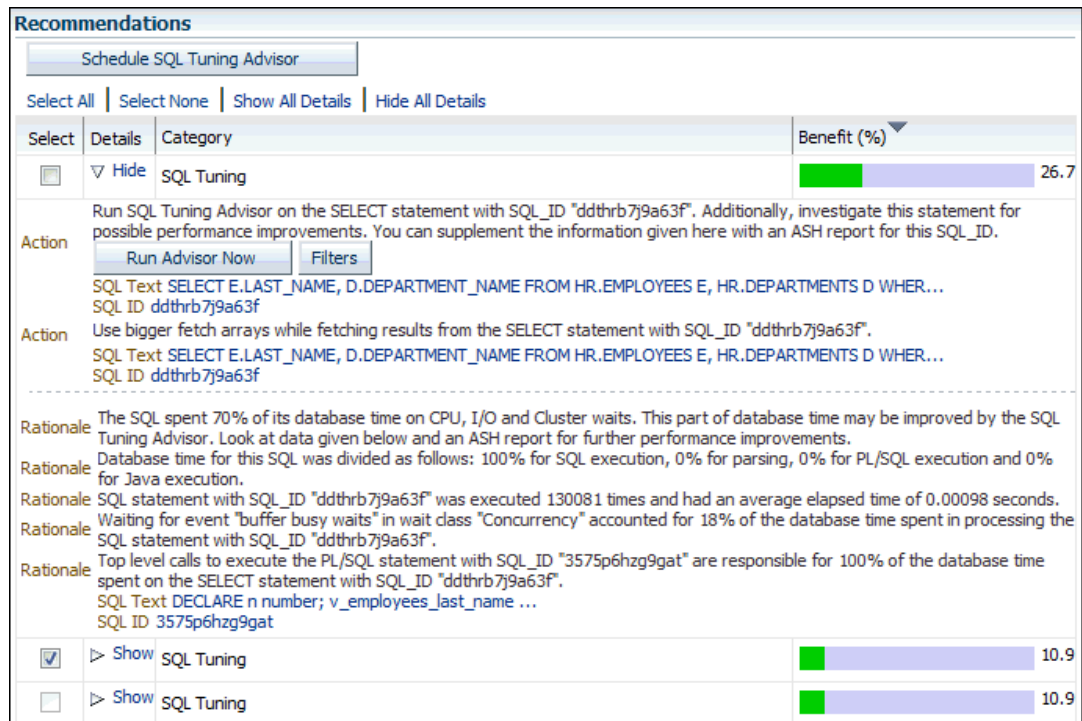
Figure 3-2 Recommendations on the Performance Finding Details Page
