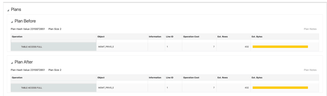
Figure 17-9 Plan Changes
