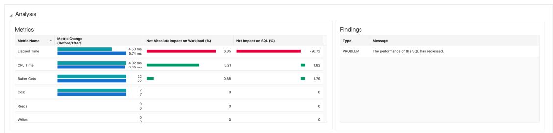
Figure 17-7 Analysis Metrics
