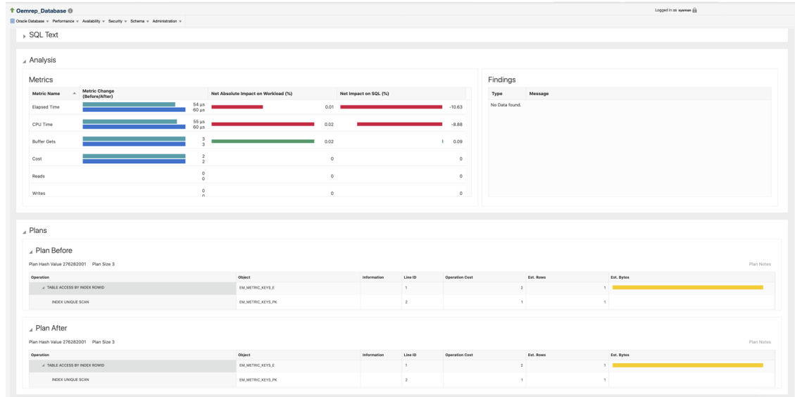
Figure 17-5 SQL Details
