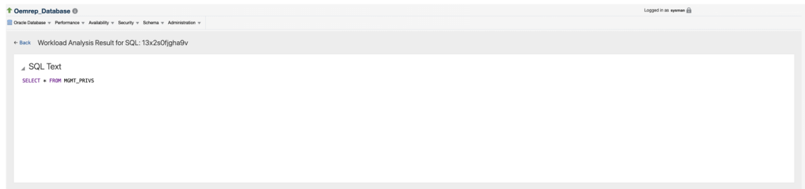
Figure 17-6 SQL Text
