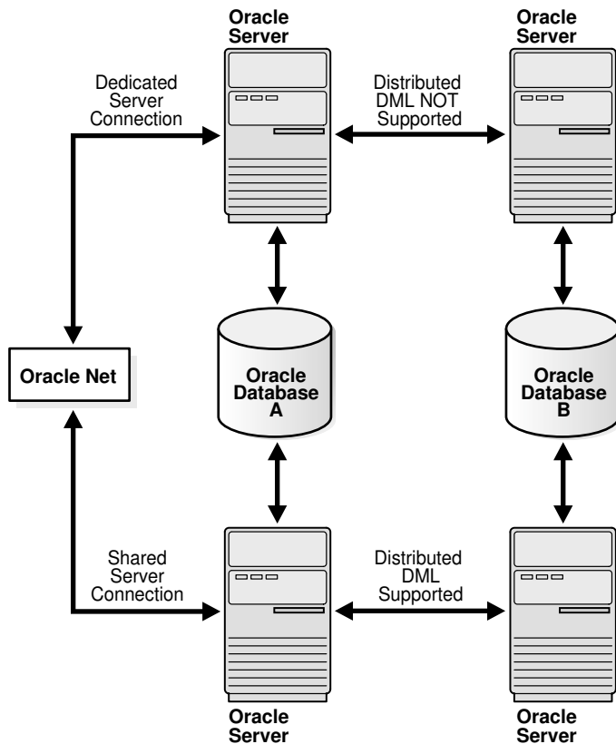
Figure 6-1 Distributed DML Statements from MTS Applications
