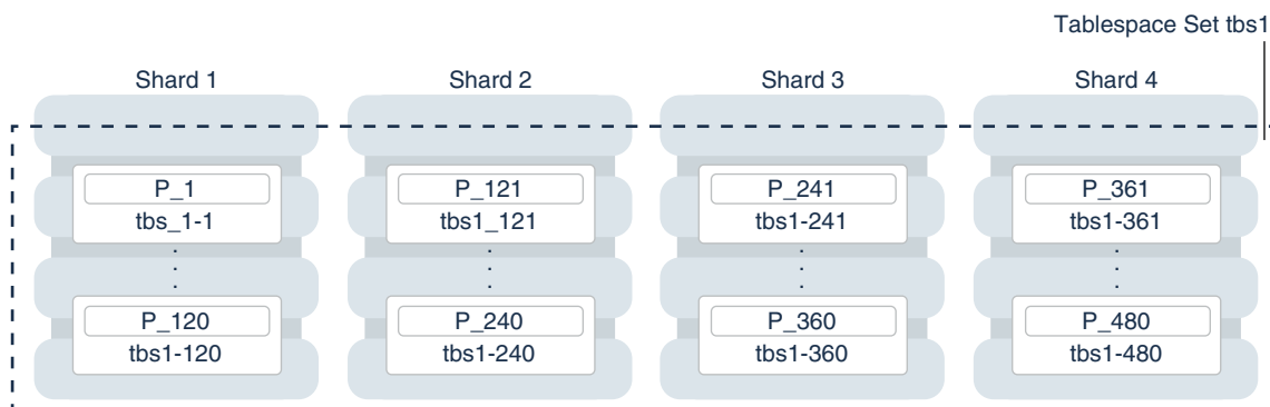
Figure 2-7 System-Managed Sharding
