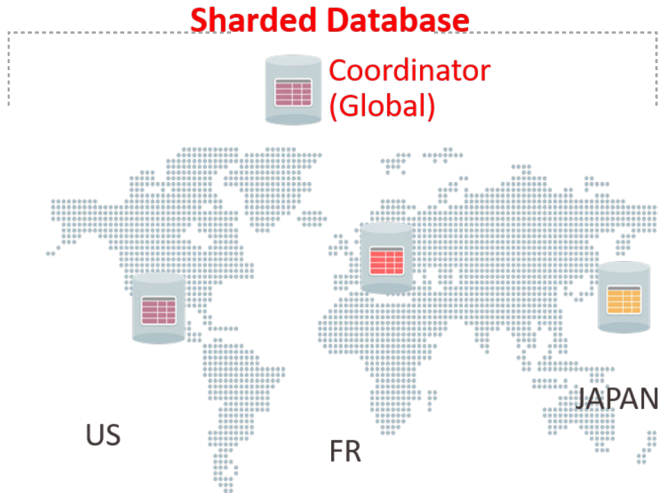
Figure 13-2 Sharded Database
