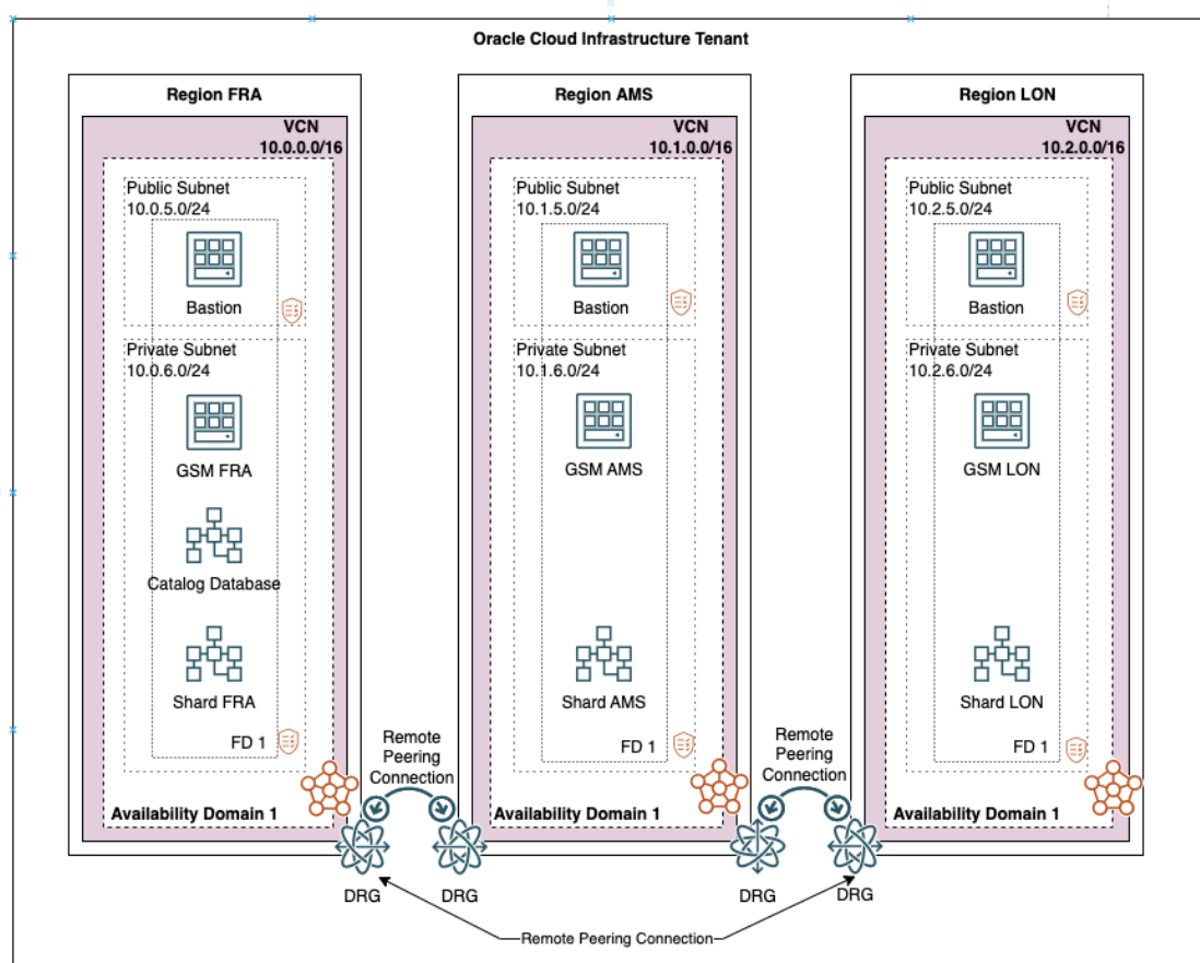
Figure 13-3 Deployment Topology of Data Sovereignty with Oracle Sharding
