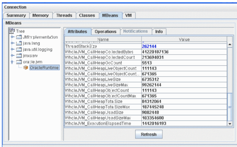
Figure 2-16 OracleRuntime MBean
