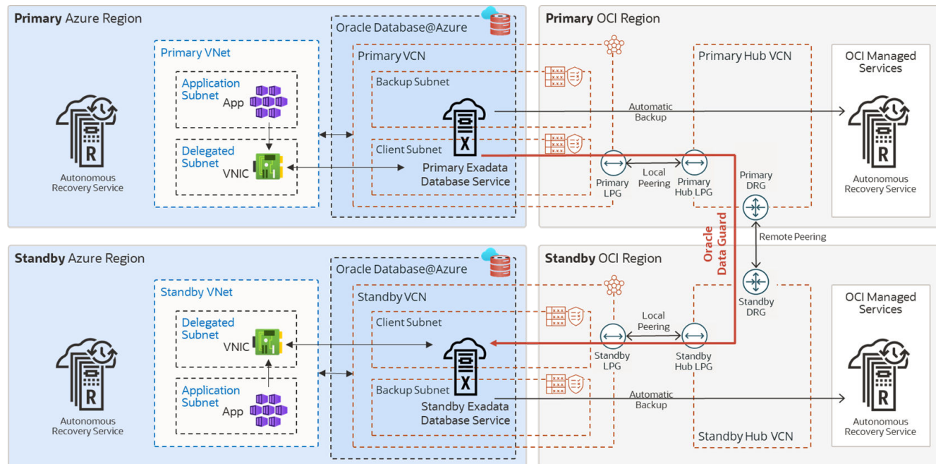
Figure 33-3 MAA Gold DR Architecture Across Two Azure Regions
