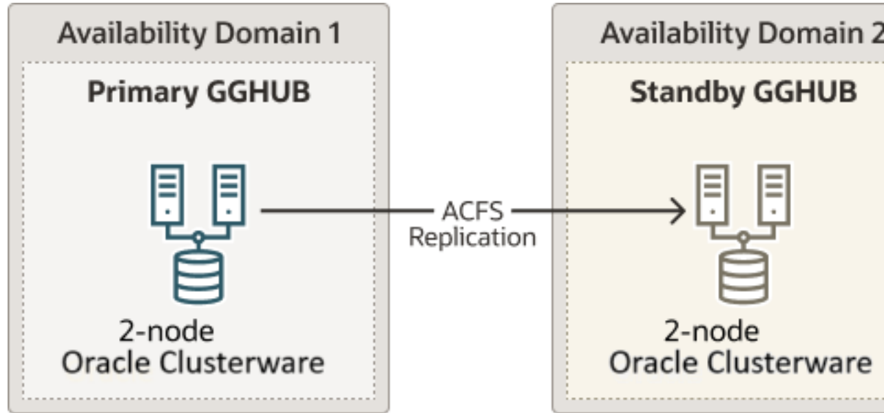
Figure 20-2 Oracle GoldenGate Maximum Availability Hub Hardware Architecture
