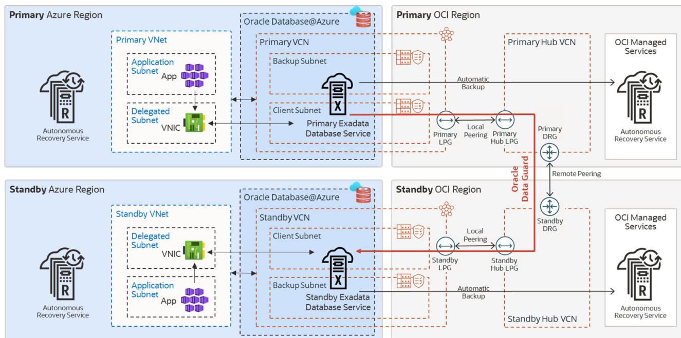
Figure 33-5 MAA Gold DR Architecture Across Two Azure Regions
