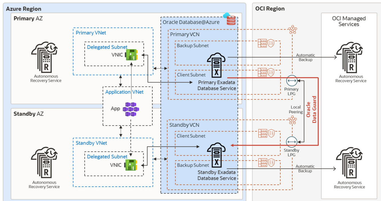
Figure 33-4 MAA Gold DR Architecture in the Same Azure Region
