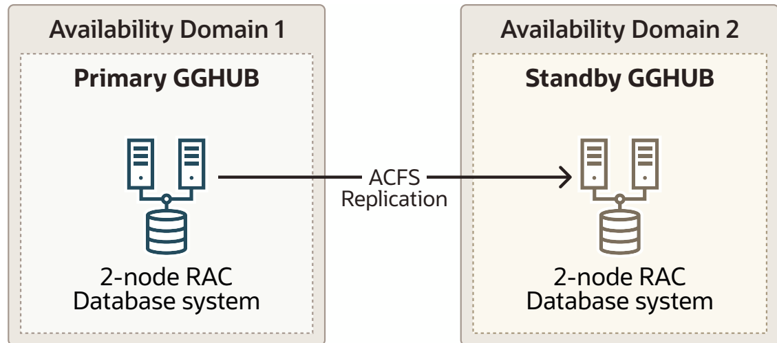
Figure 24-3 Oracle GoldenGate Hub Hardware Architecture
