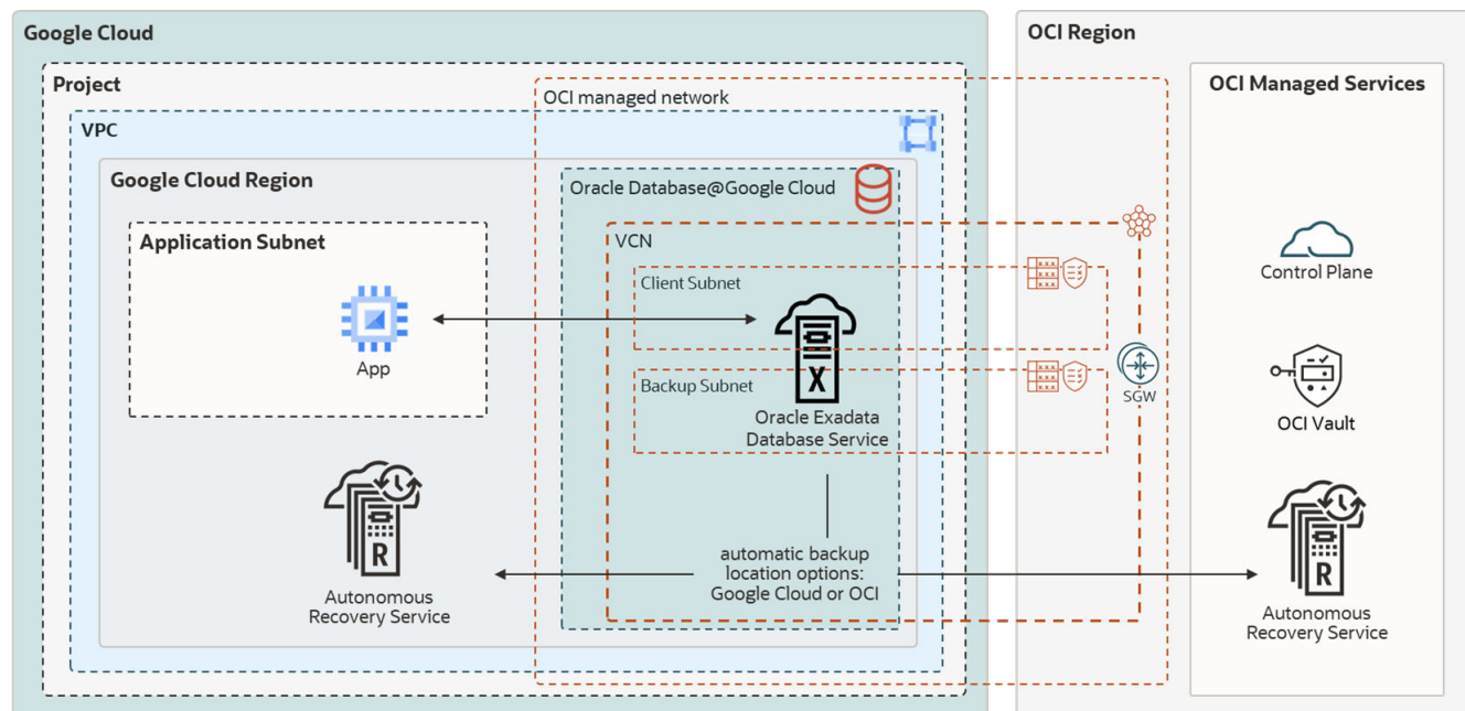
Figure 33-6 MAA Silver Architecture for Oracle Database@Google
