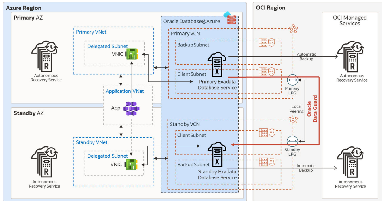
Figure 33-2 MAA Gold DR Architecture in the Same Azure Region
