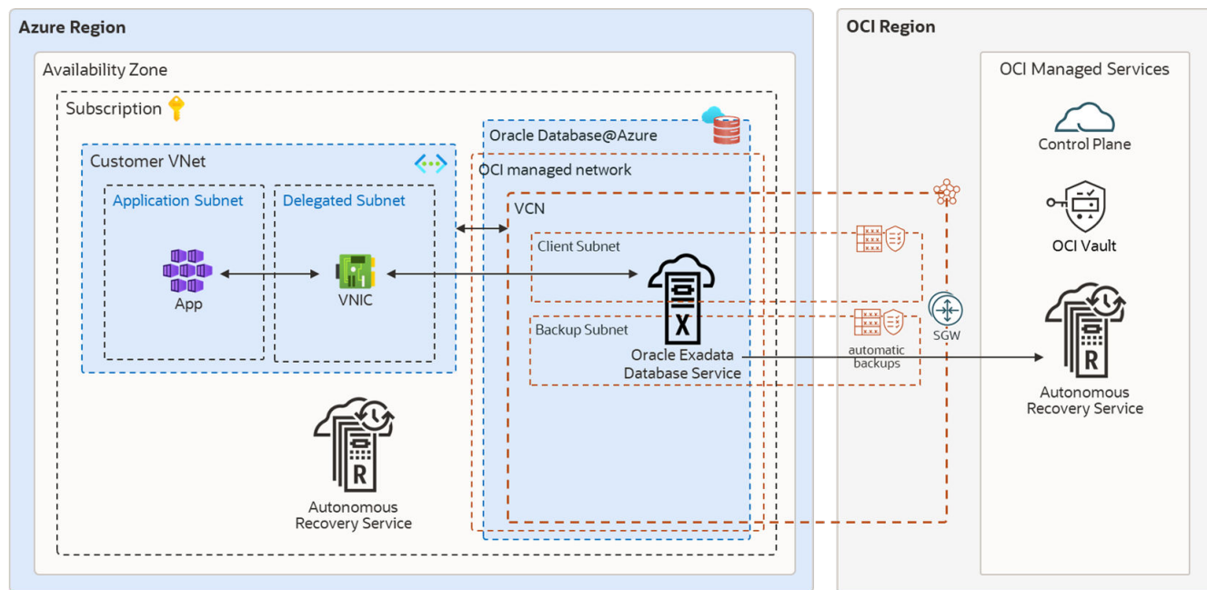
Figure 33-1 MAA Silver Architecture for Oracle Database@Azure
