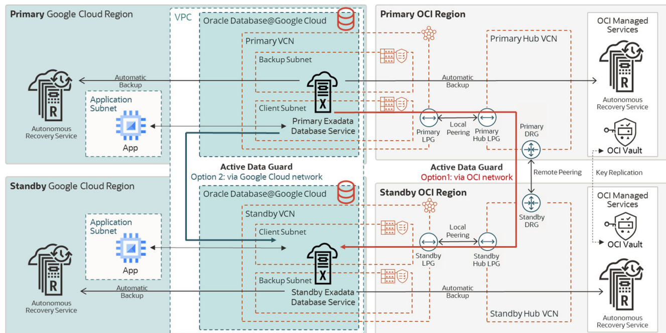
Figure 33-7 MAA Gold Architecture for Oracle Database@Google
