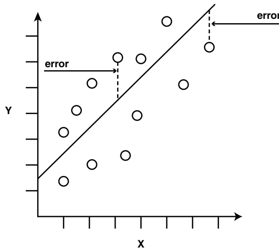
Figure 4-1 Linear Regression With a Single Predictor
