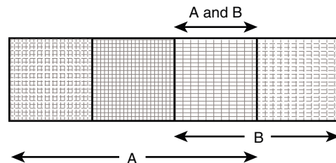
Figure 20-1 Conditional Probabilities in Bayes' Theorem
