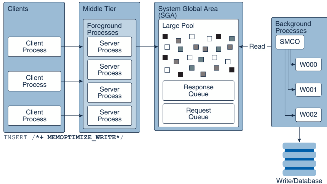
Figure 14-12 Deferred Insert Mechanism
