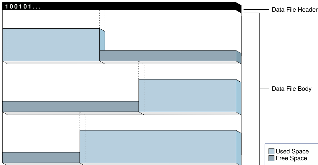
Figure 12-4 Bitmap-Managed Storage
