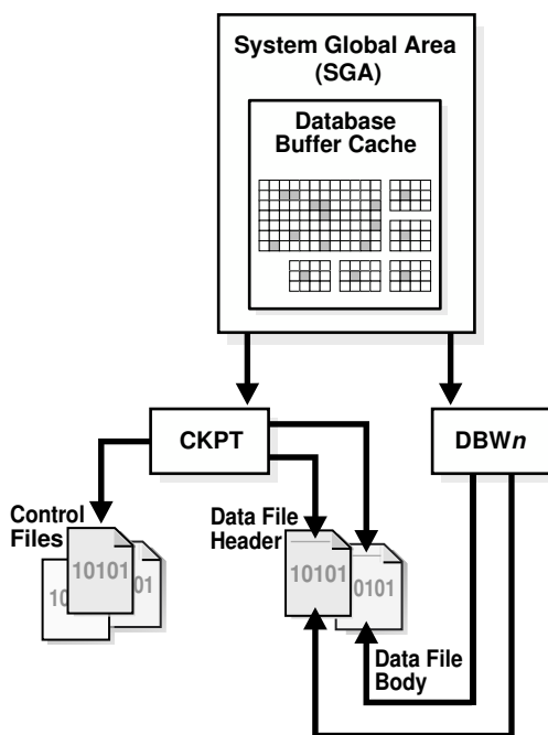
Figure 15-4 Checkpoint Process
