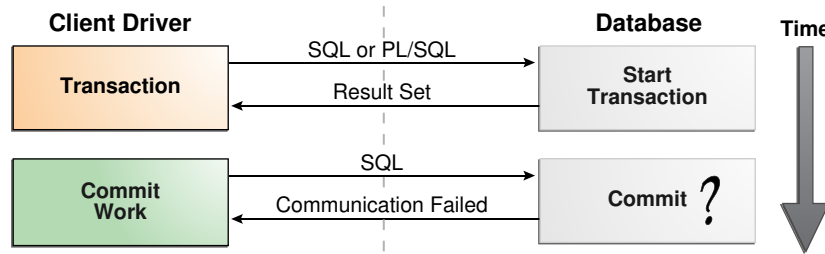
Figure 10-2 Lost Commit Message
