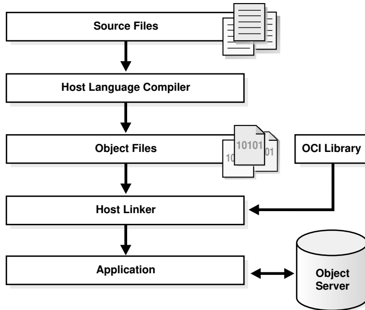
Figure 19-3 Development Process Using OCI or OCCl
