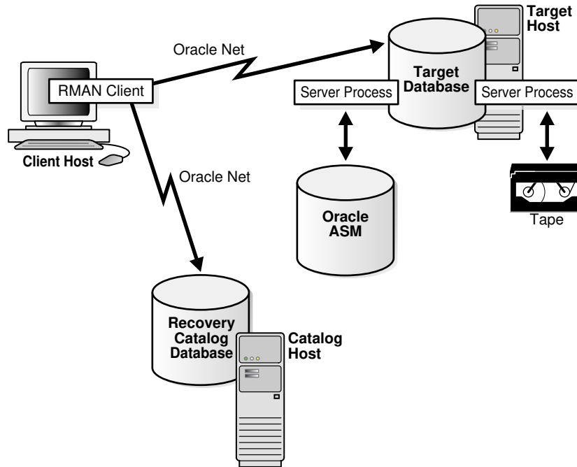
Figure 18-3 RMAN Architecture
