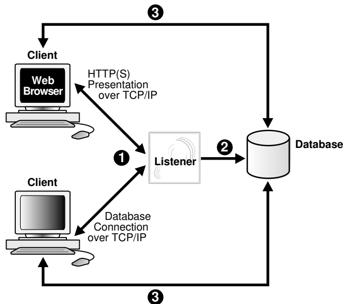
Figure 16-5 Listener Architecture
