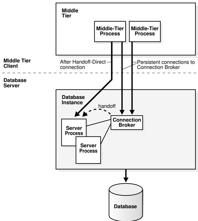
Figure 16-9 DRCP
