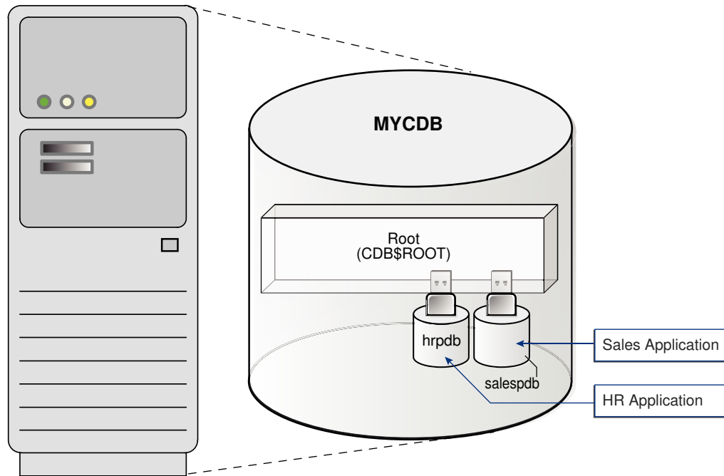
Figure 1-3 Consolidation of Non-CDBs into a CDB
