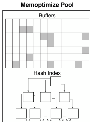
Figure 14-13 Memoptimize Pool
