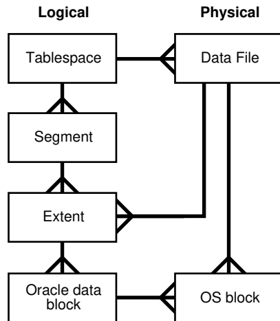
Figure 12-1 Logical and Physical Storage
