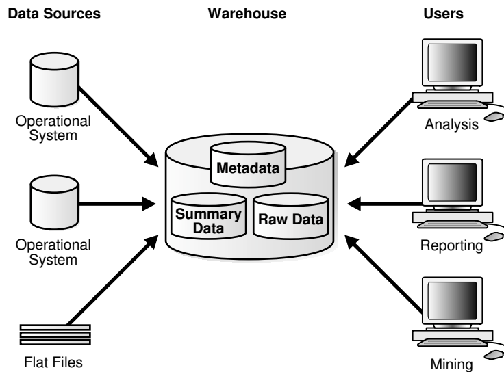
Figure 17-3 Architecture of a Data Warehouse
