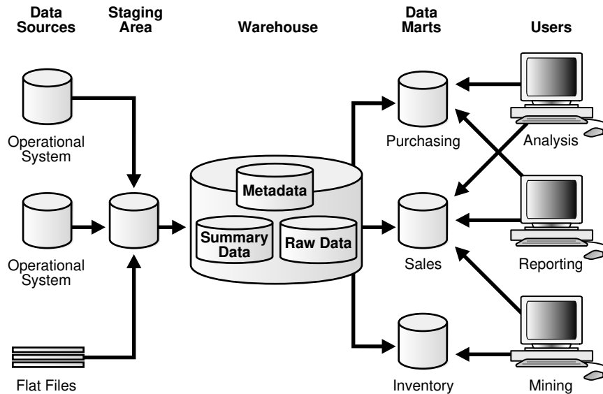
Figure 17-5 Architecture of a Data Warehouse with a Staging Area and Data Marts
