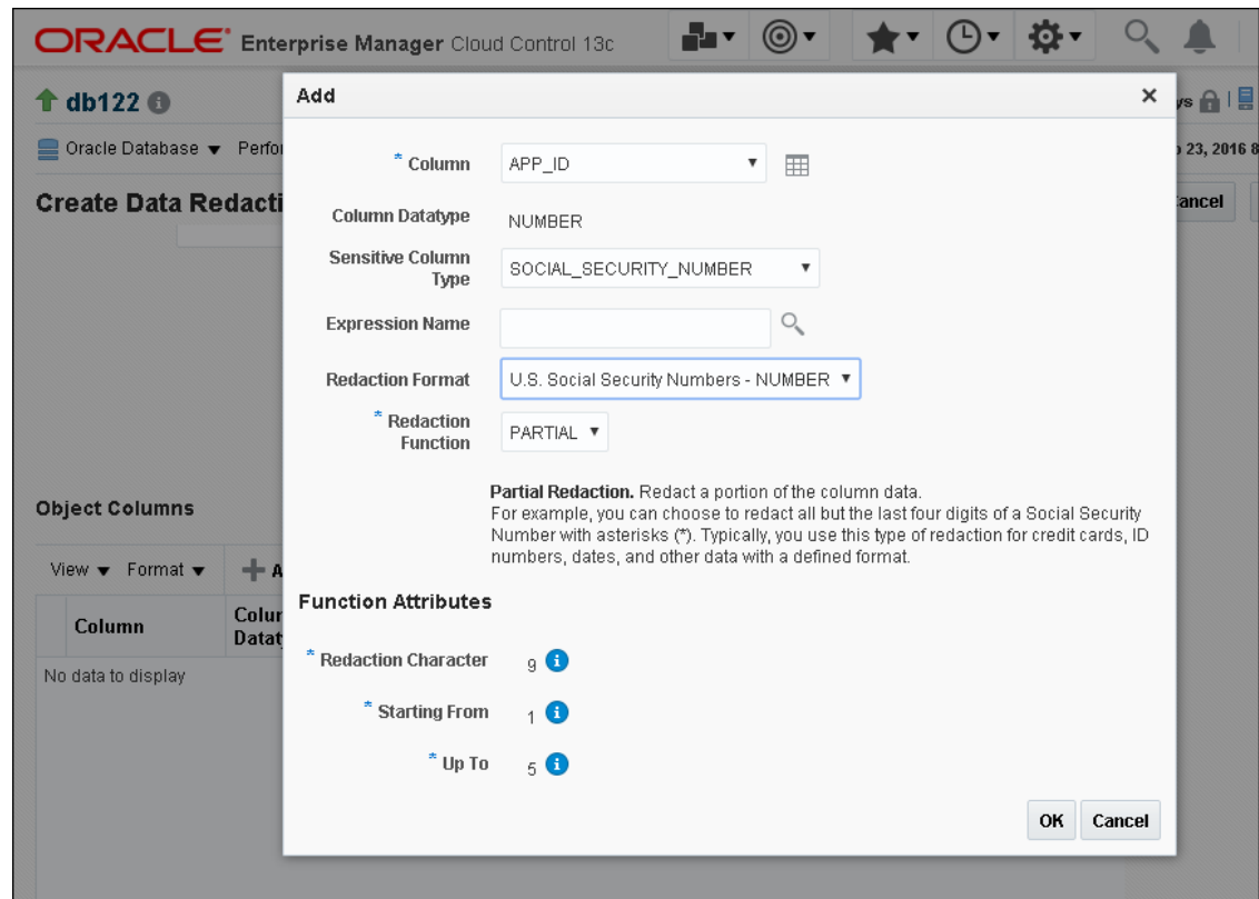
Figure 15-1 Oracle Data Redaction Formats Filtered on the Basis of Sensitive Column Types
