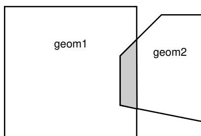
Figure 26-3 SDO_GEOM.SDO_INTERSECTION
