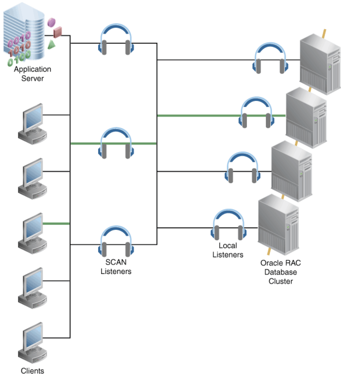
Figure 31-1 Connection Load Balancing Using the SCAN
