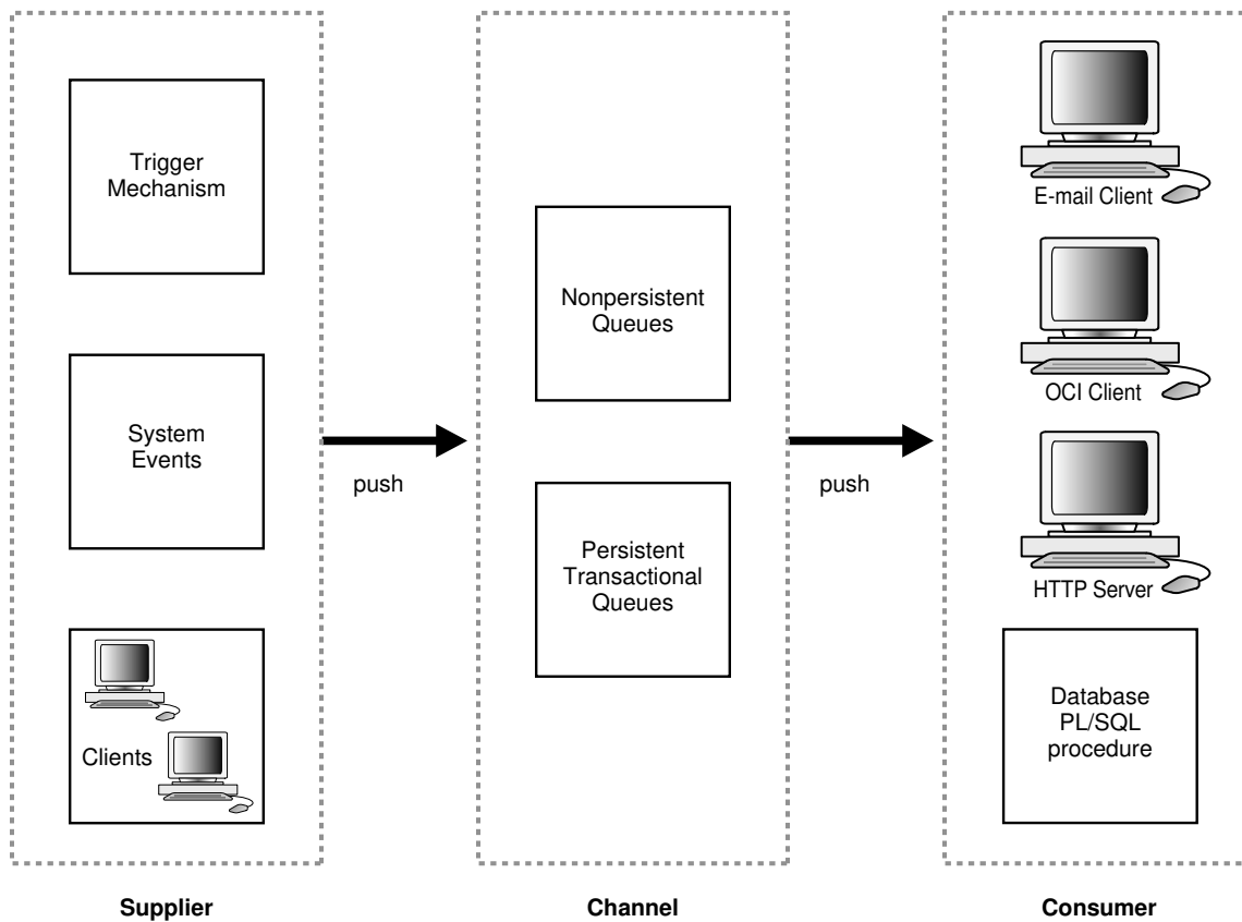
Figure 10-2 Publish-Subscribe Model
