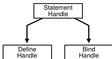
Figure 3-3 Statement Handles
