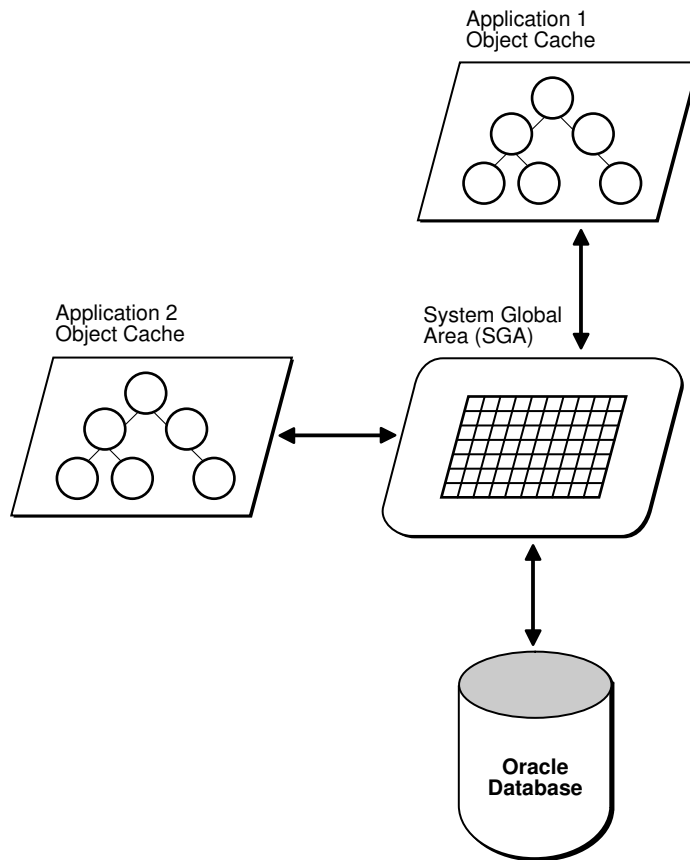
Figure 15-1 Object Cache
