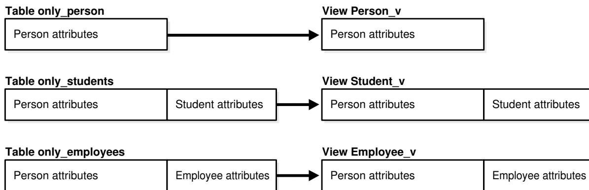
Figure 6-3 Horizontal Storage Model for Object View Hierarchy
