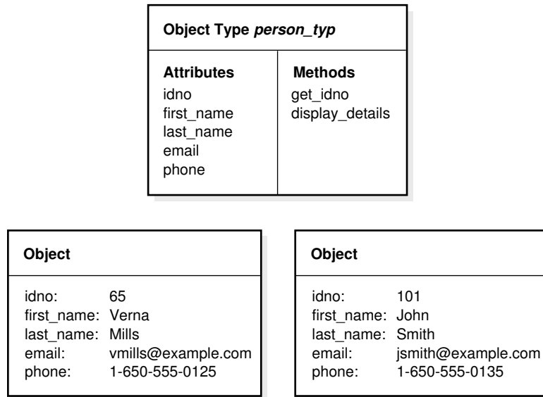
Figure 1-1 Object Type and Object Instances
