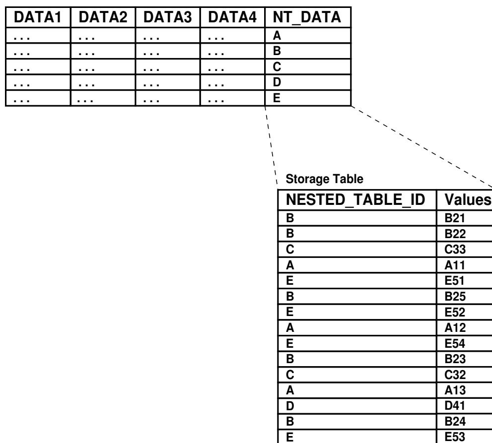
Figure 9-2 Nested Table Storage
