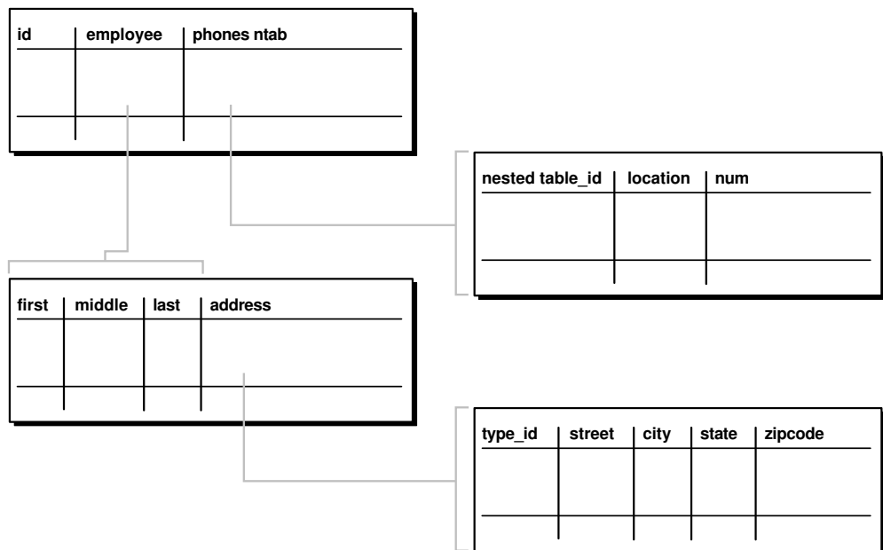
Figure 9-1 Representation of the people_reltab Relational Table
