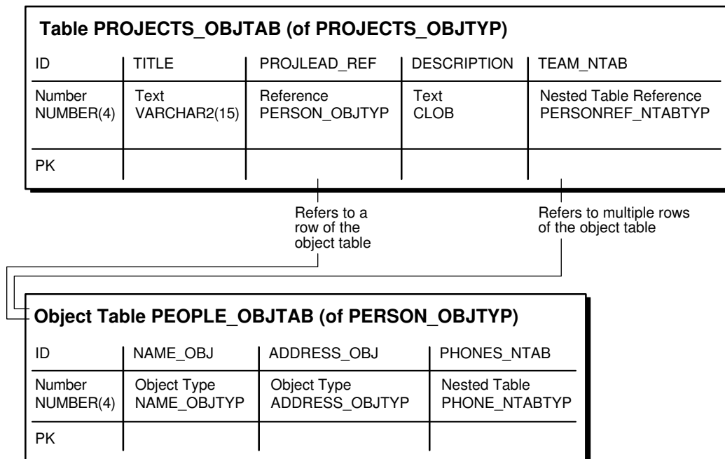
Figure 9-4 Object-Relational Representation of the projects_objtab Object Table
