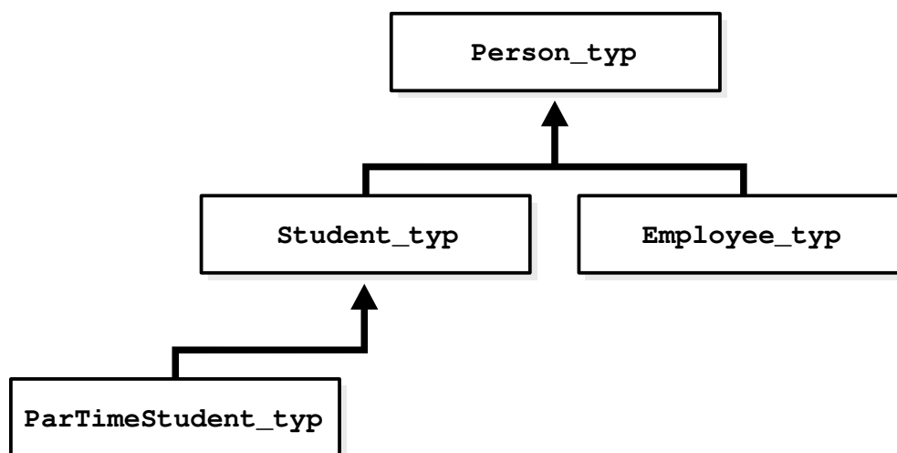
Figure 6-1 Object Type Hierarchy
