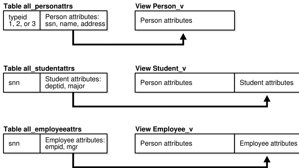
Figure 6-4 Vertical Storage Model for Object View Hierarchy
