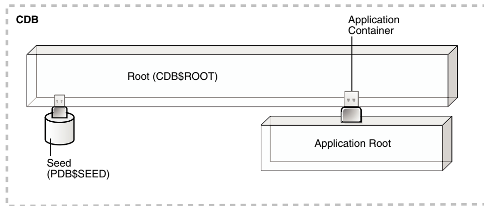
Figure 36-4 An Application Container
