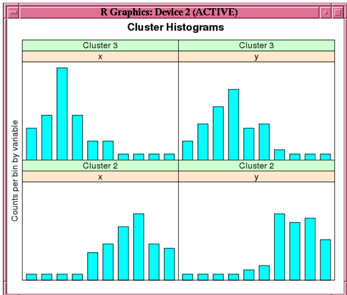
Figure 7-2 Cluster Histograms for the km.mod1 Model
