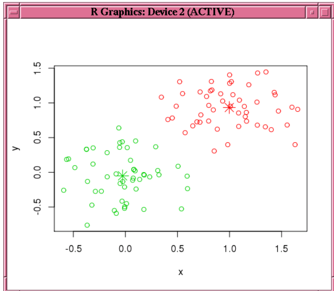
Figure 7-3 Results of the points Function for the km.mod1 Model
