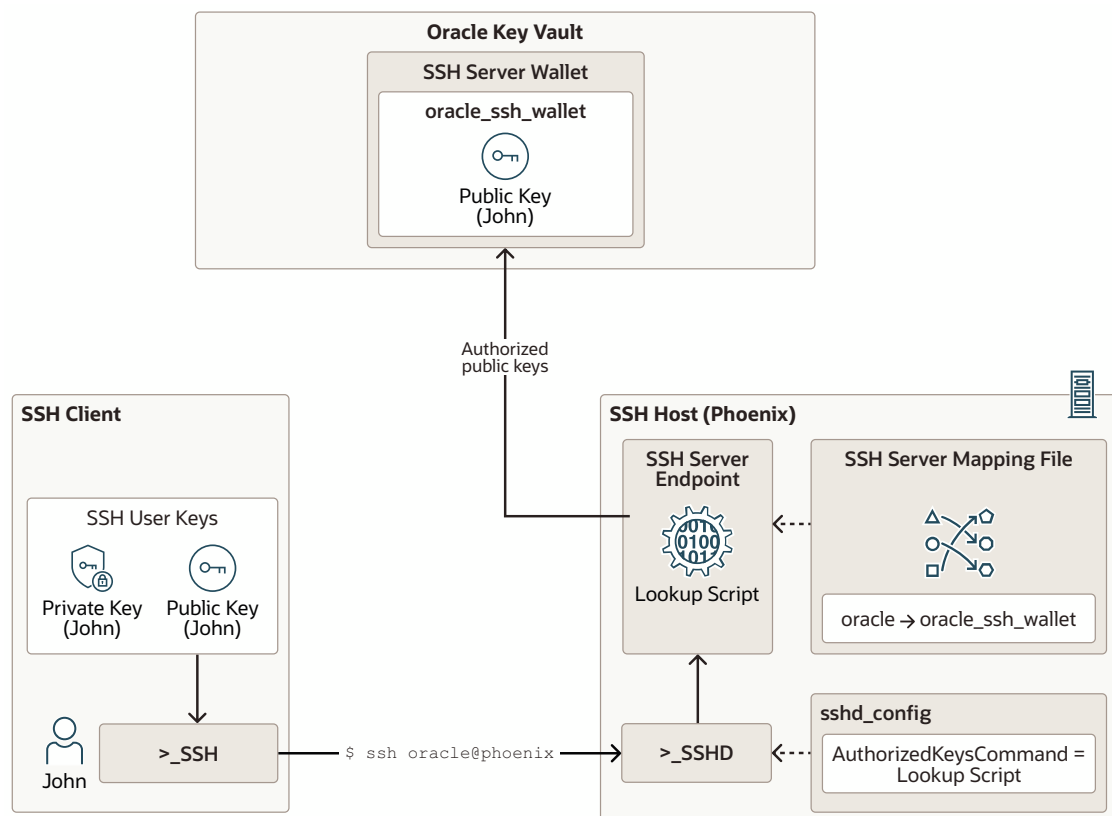
Figure 15-5 Centralized-SSH-Server-Access
