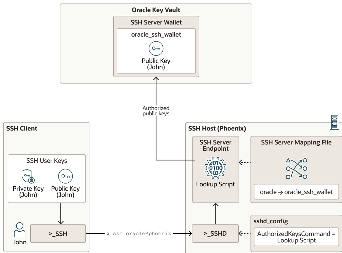
Figure 15-5 Centralized-SSH-Server-Access
