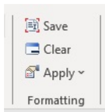
Figure 22-17 Formatting Options
