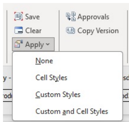
Figure 22-18 Apply Options
