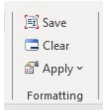
Figure 27-1 Formatting Options
