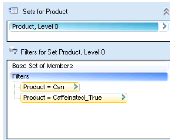
Figure 19-1 Union of Sets
