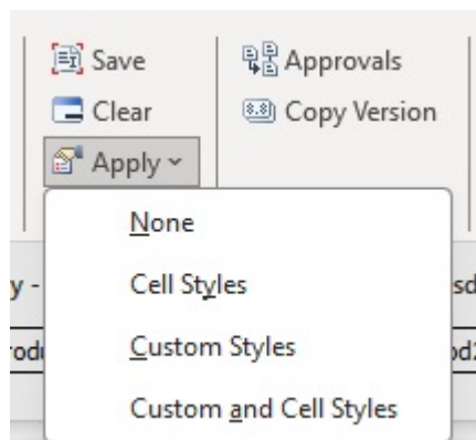
Figure 22-19 Apply Options
