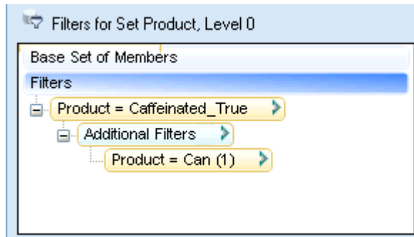
Figure 19-2 Intersection of Sets
