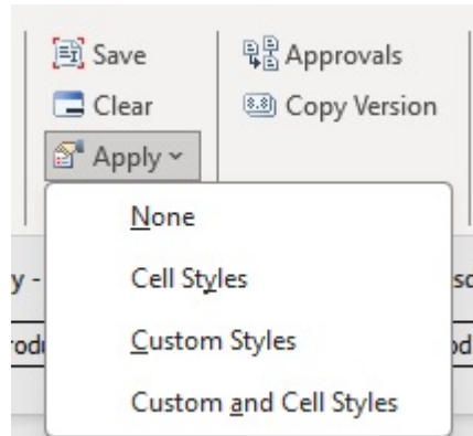
Figure 27-2 Apply Options
