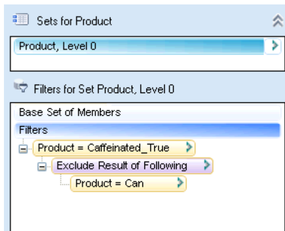
Figure 19-3 Complement of Sets
