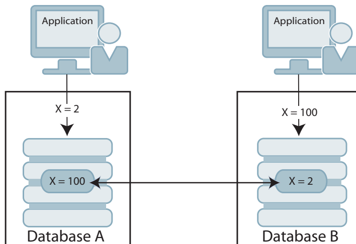
Figure 12–1 Update conflict
