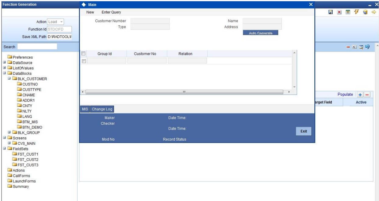
Fig 6.2.3: 12.0 Kernel version
