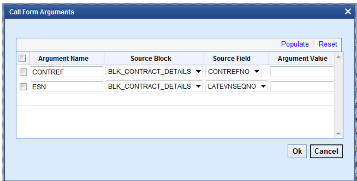
Fig 12.3 Passing Screen Arguments to Call Form Screen
