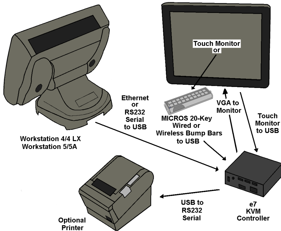
Figure 23-1 e7 Kitchen Video Monitor System
