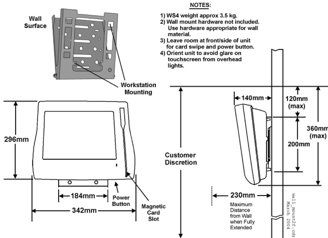
Figure 32-38 Workstation 4/4 LX Dimensions on Wall Mount Bracket
