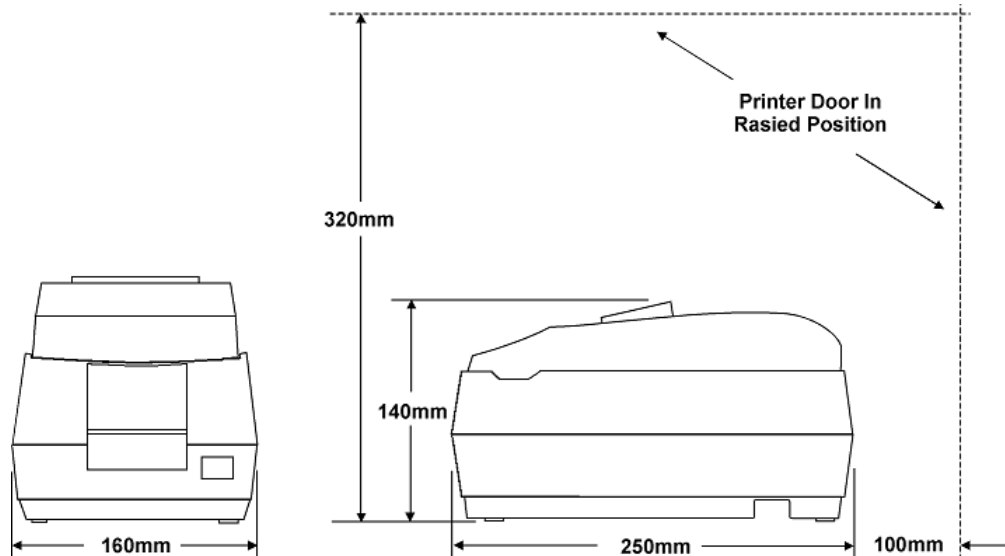
Figure 32-49 U200D Roll Printer Dimensions
