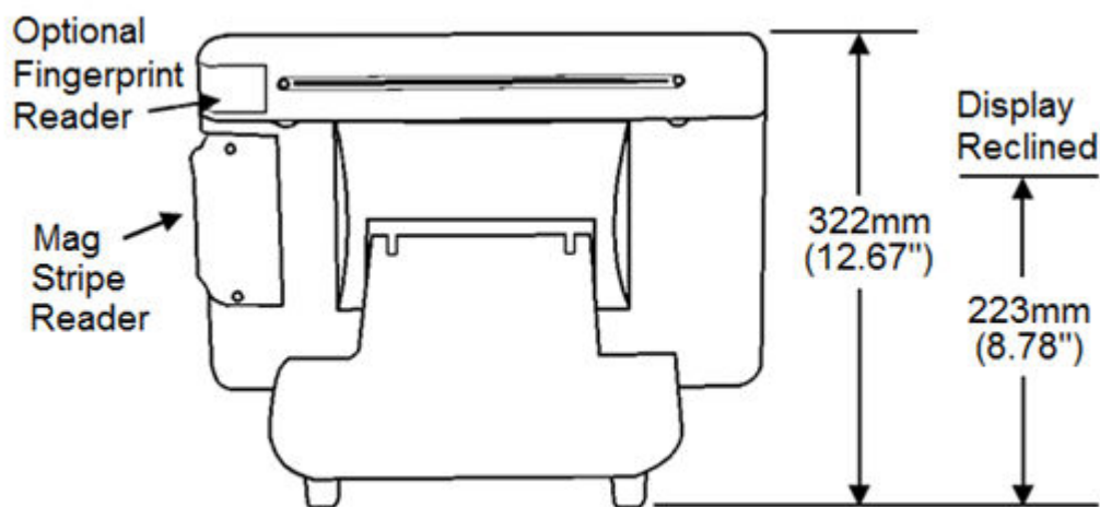
Figure 32-9 Workstation 6 Series Back Dimensions
