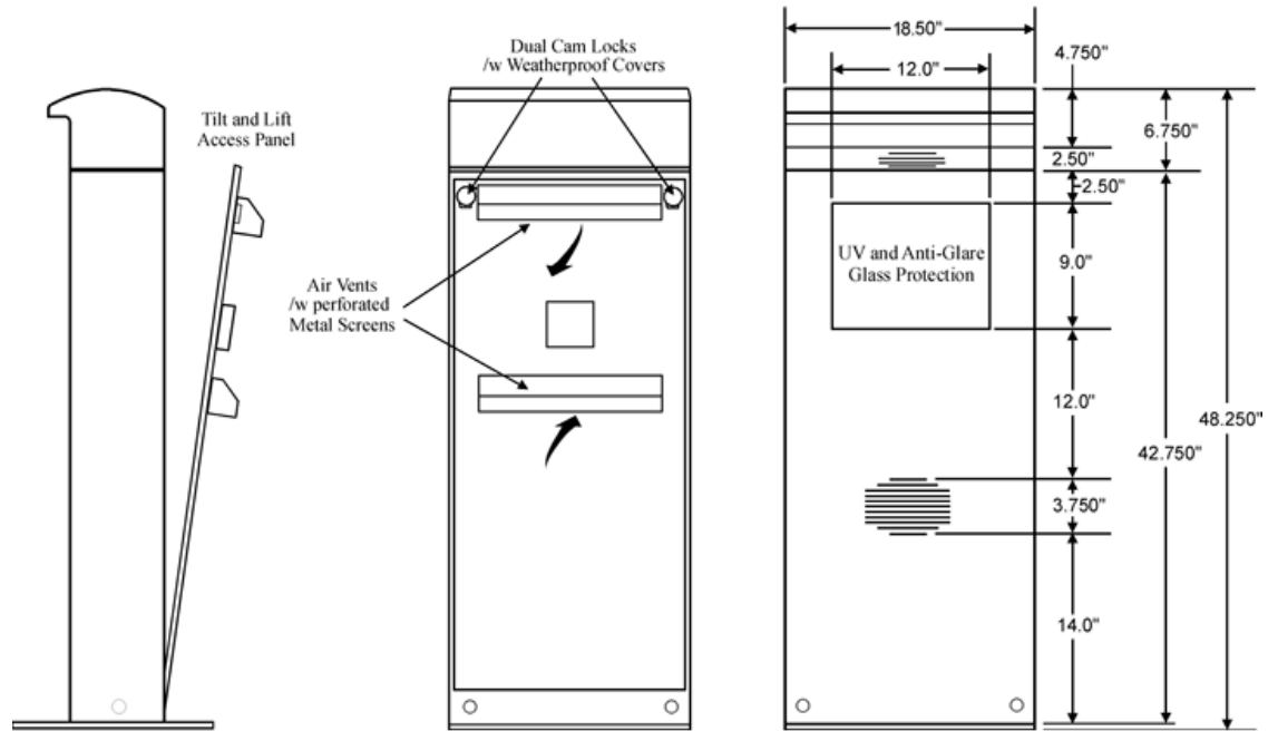
Figure 32-44 Order Confirmation System Remote Display Pedestal - Detail 2 Dimensions
