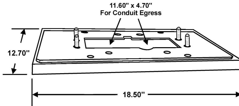
Figure 18-2 Pedestal Slab Example
