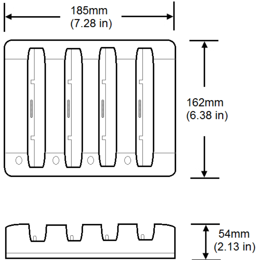
Figure 32-7 Tablet 700 Series 4-Bay Battery Charger Dimensions
