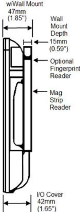
Figure 32-15 Workstation 6 Series Wall Mount Dimensions
