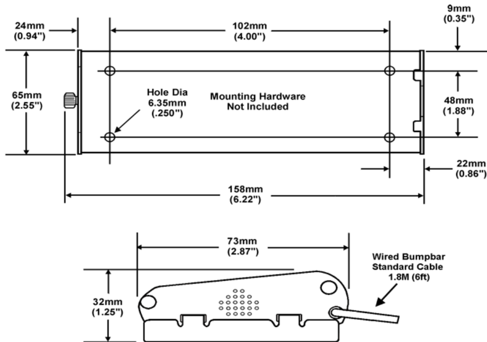
Figure 32-46 10-Key Bumpbar Mounting Bracket Dimensions
