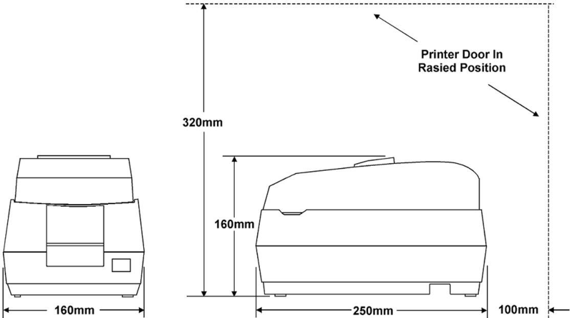
Figure 32-51 U200B Auto-Cut Roll Printer Dimensions
