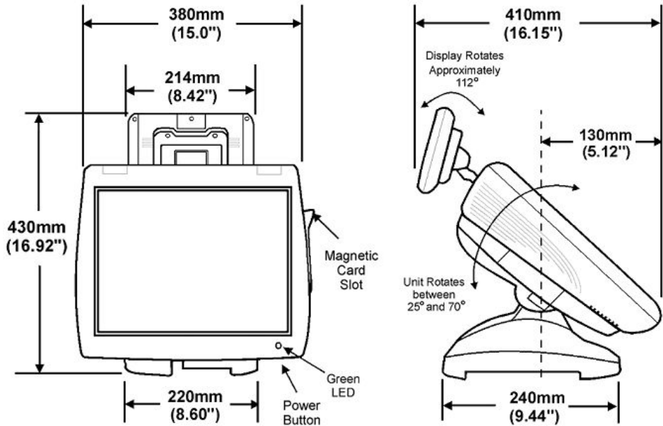
Figure 32-27 Workstation 5/5A - Low Profile Dimensions
