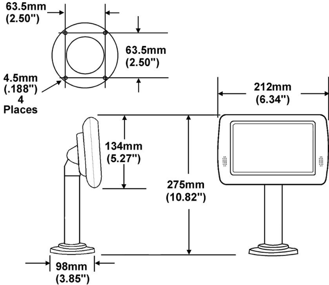
Figure 32-53 Pole Mount (6 inch) Protégé Customer Display Dimensions
