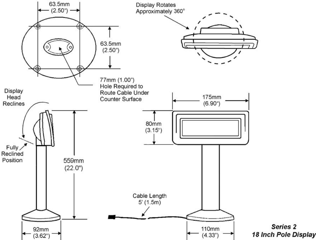
Figure 32-55 Series 2 Pole Customer Display Dimensions
