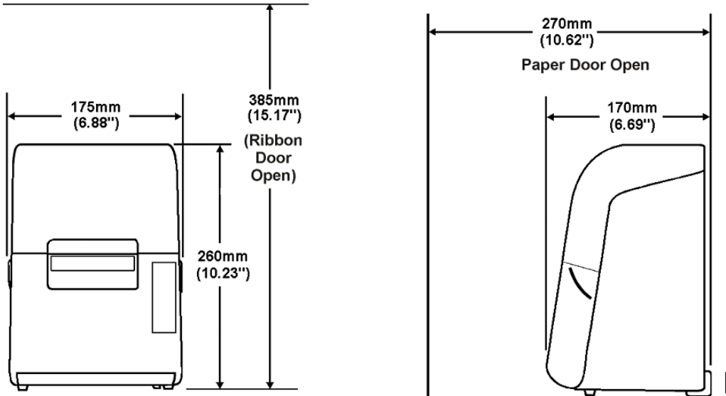
Figure 32-52 U230 Auto-Cut Roll Printer Dimensions
