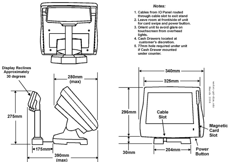
Figure 32-37 Workstation 4/4 LX Dimensions on Stand with VFD Customer Display
