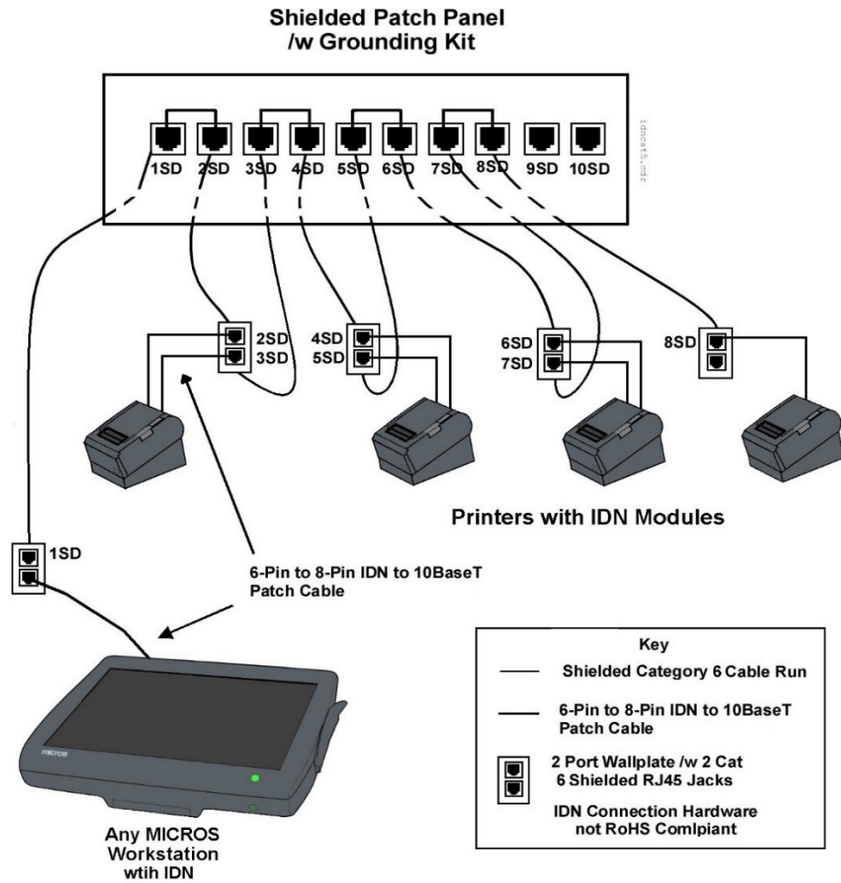
Figure 31-1 MICROS Workstation Driving IDN Printers over Shielded Cabling
