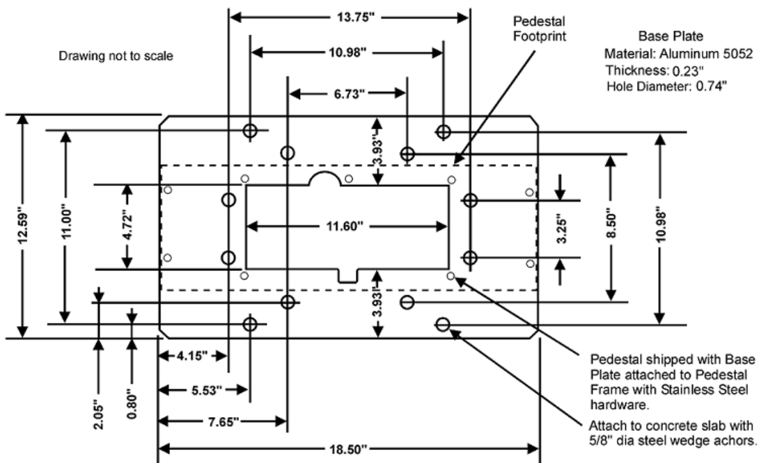
Figure 32-45 Order Confirmation System Remote Display Pedestal Baseplate Dimensions
