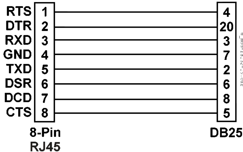
Figure 34-5 Modular RS232 Port to DB25 Male Connector
