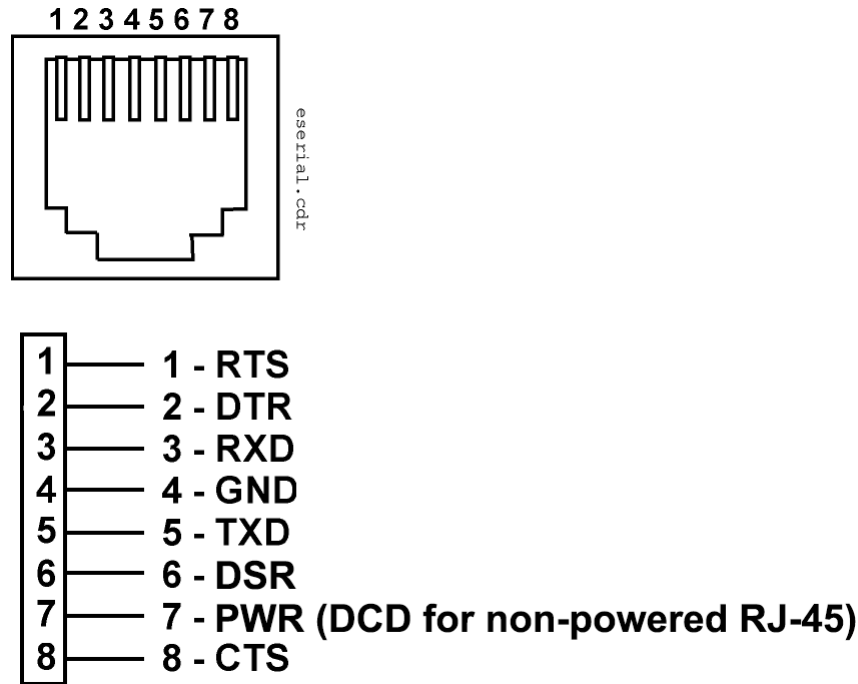
Figure 33-3 Modular COM Port with Handshaking
