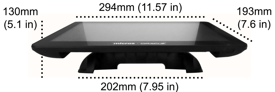
Figure 32-2 Dimensions of the Compact Workstation 310 with Basic Stand
