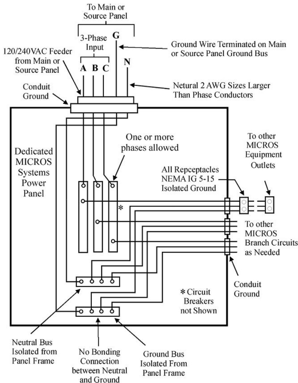
Figure 25-1 Preferred AC Power System Panel Wiring
