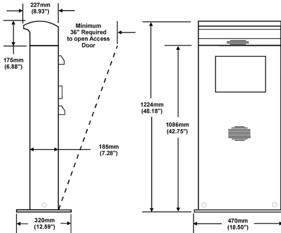
Figure 32-42 Order Confirmation System Remote Display Pedestal - Basic Dimensions
