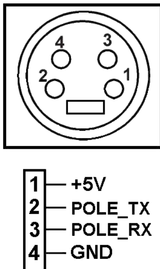
Figure 33-7 Remote Customer Display Connector Diagram
