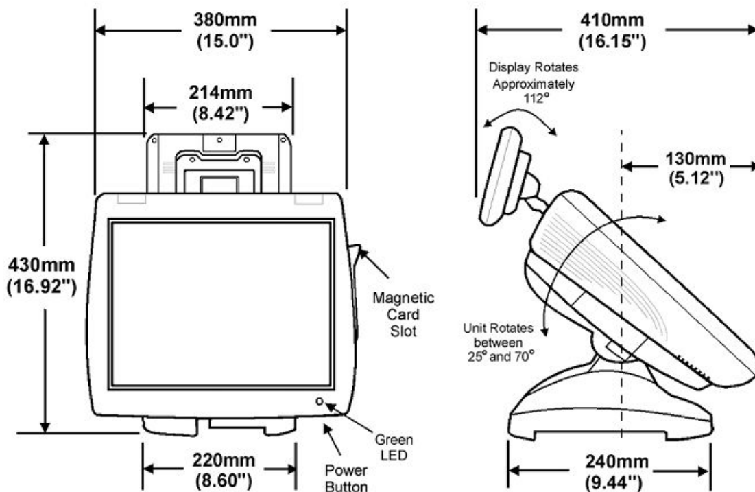
Figure 32-26 PC Workstation 2015 - Adjustable Stand Protégé Customer Display Dimensions
