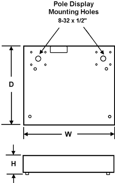
Figure 32-56 Cash Drawer Dimensions
