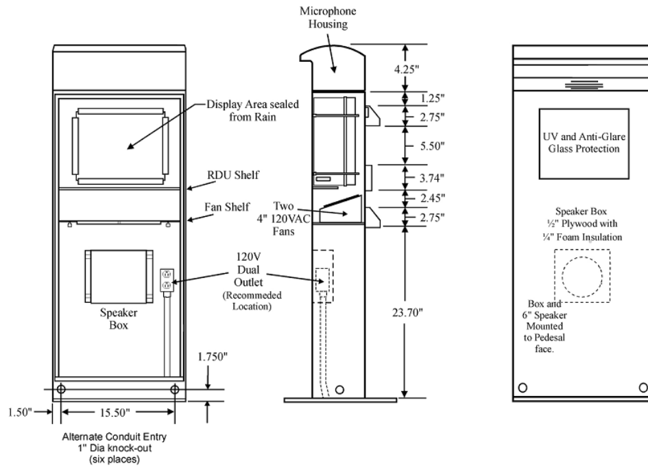
Figure 32-43 Order Confirmation System Remote Display Pedestal - Detail 1 Dimensions
