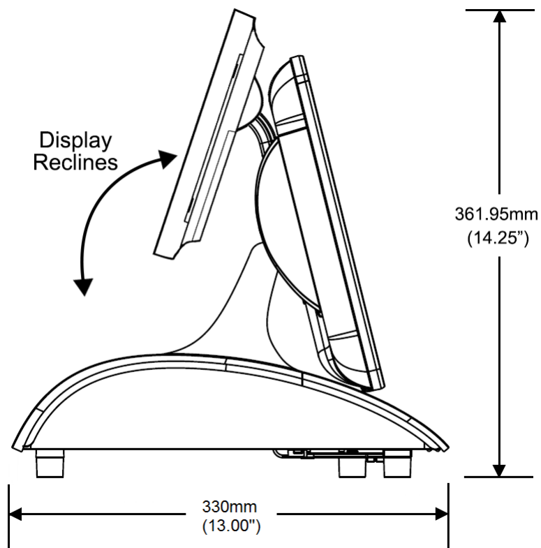
Figure 32-12 Dimensions (Side) of the 10-Inch Customer Display with High Mount
