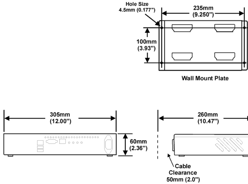
Figure 32-41 Order Confirmation Controller and Wall Bracket Dimensions
