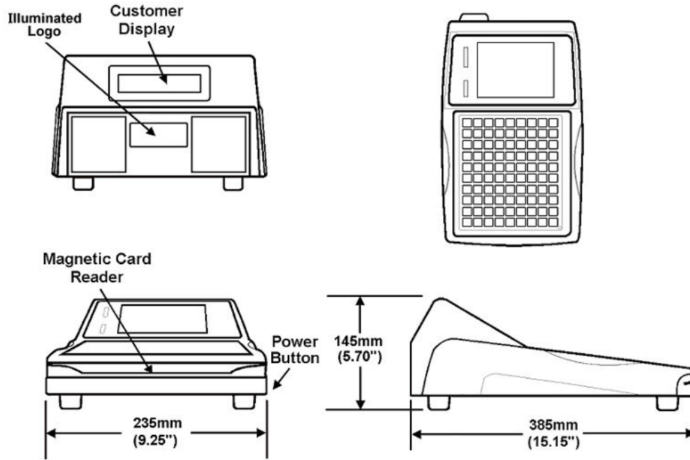
Figure 32-39 KW270 Low Profile Dimensions
