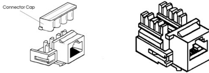
Figure 30-1 8-Pin Keystone (left) and 110 Connect (right) RJ45 Modular Jack
