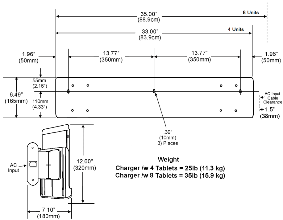
Figure 32-19 Tablet E-Series Multi-Unit Charger - Wall Mount Dimensions
