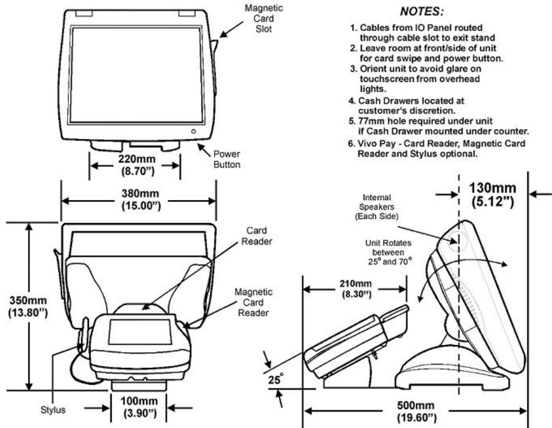
Figure 32-32 Workstation 5/5A Dimensions on Stand /w Vivo Payment Terminal
