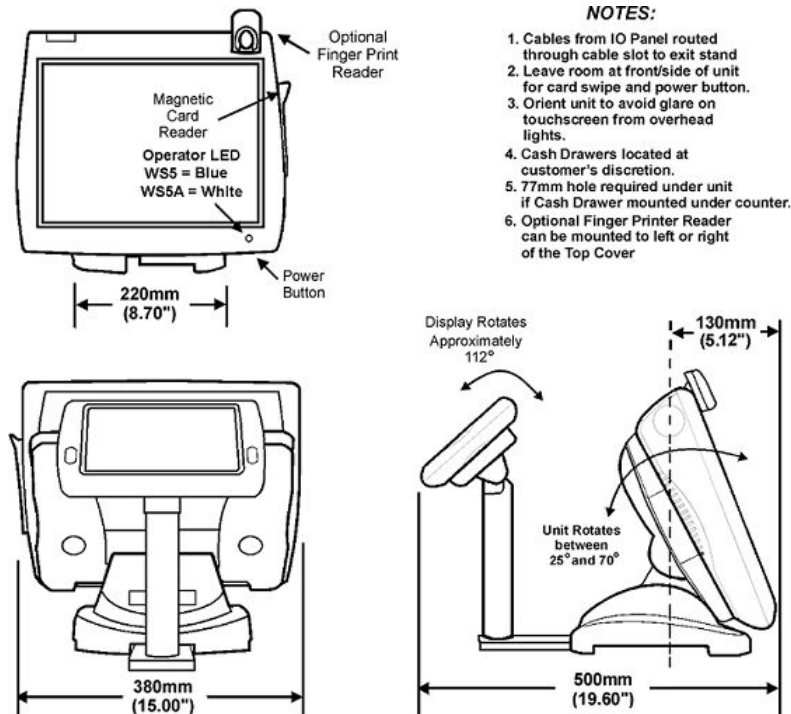
Figure 32-31 Workstation 5/5A Dimensions on Stand with Protégé Customer Display
