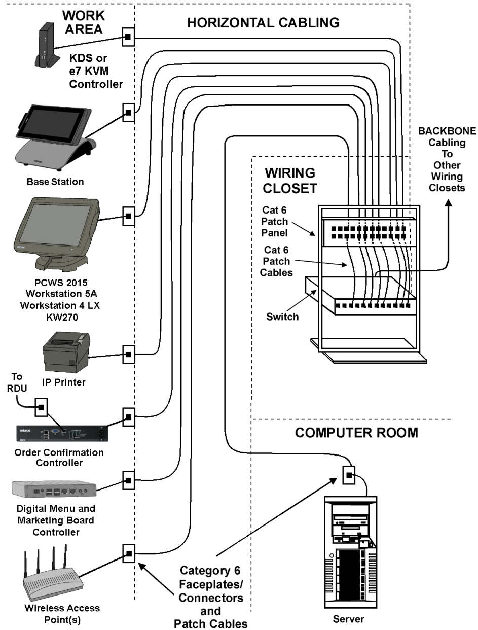
Figure 29-1 Example of MICROS Equipment in a Structured Cabling System
