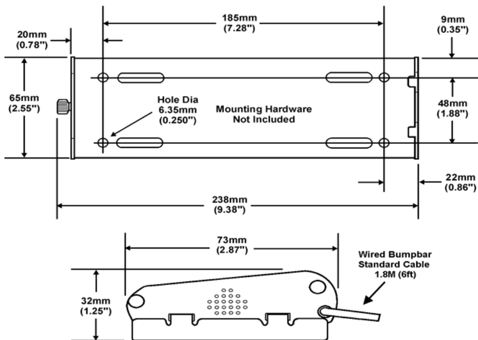
Figure 32-47 20-Key Bumpbar Mounting Bracket Dimensions
