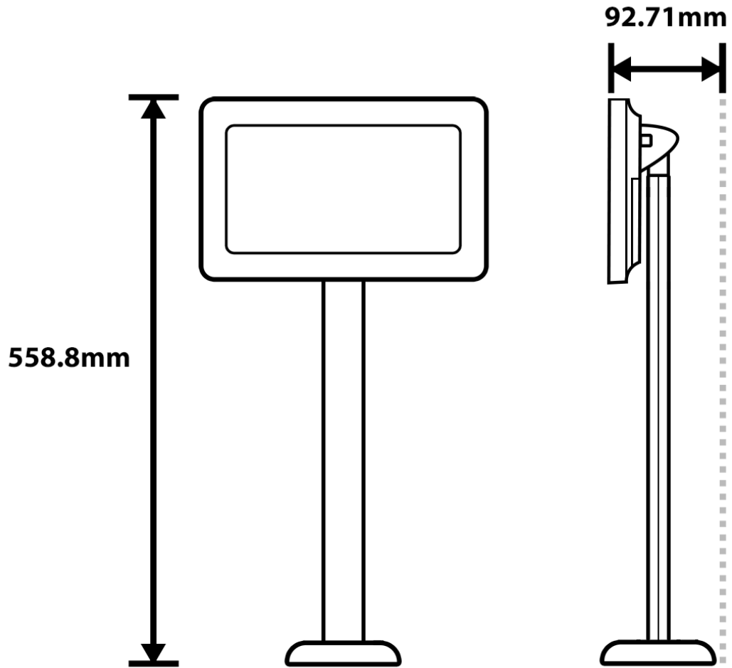
Figure 32-13 10-Inch Customer Display with Pole Mount Dimensions
