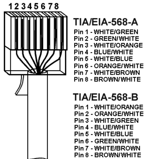
Figure 30-2 Cable Termination
