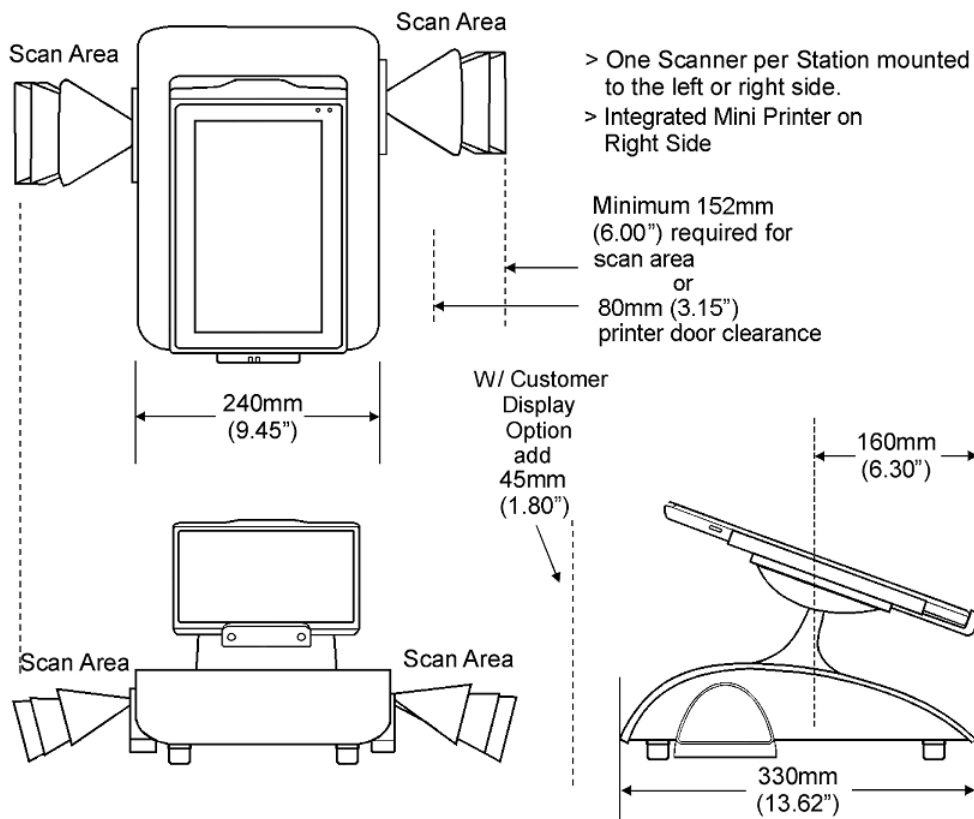
Figure 32-21 Tablet R-Series on Base Station Dimensions with Peripherals
