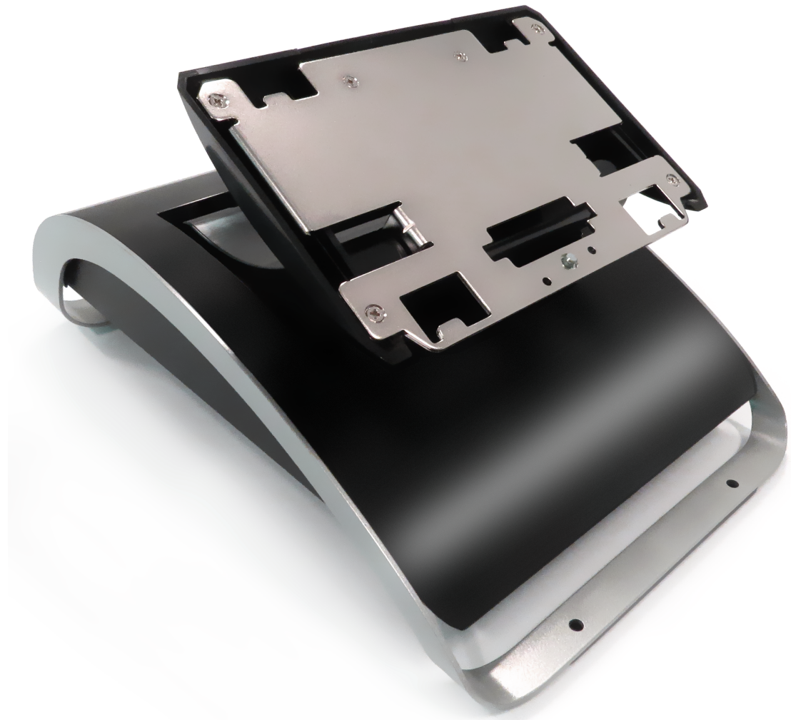
Figure 5-4 MICROS Flexible Stand
