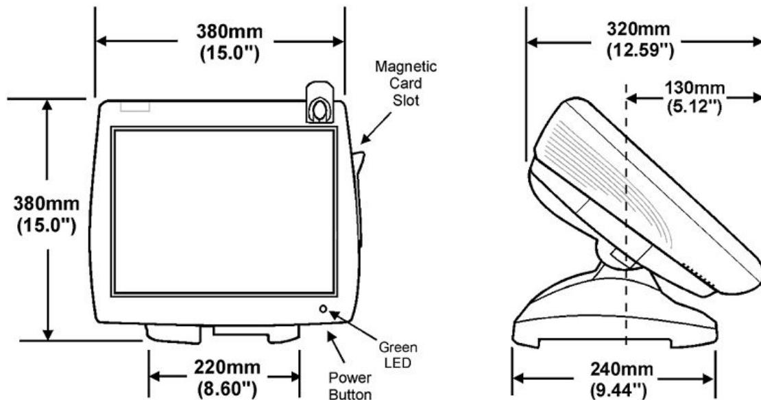
Figure 32-24 PC Workstation 2015 Adjustable Stand Dimensions
