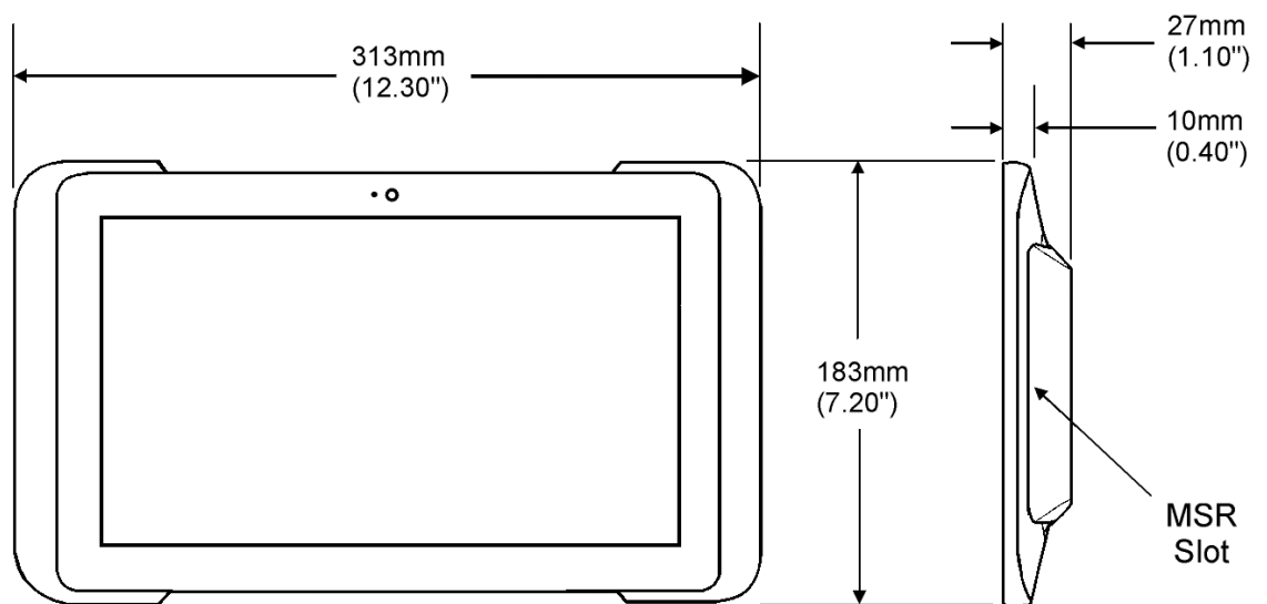
Figure 32-17 Tablet E-Series 11 Dimensions
