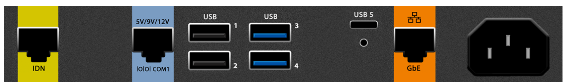
Figure 3-2 Primary I/O Panels of the MICROS Express Station 4 Series
