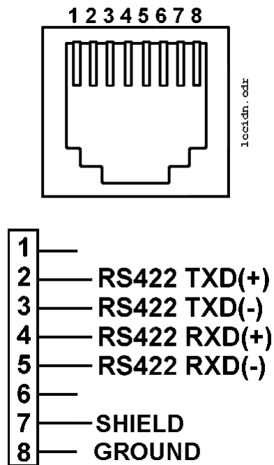
Figure 33-1 IDN or RS422-A/B Connectors Configured for IDN Printing
