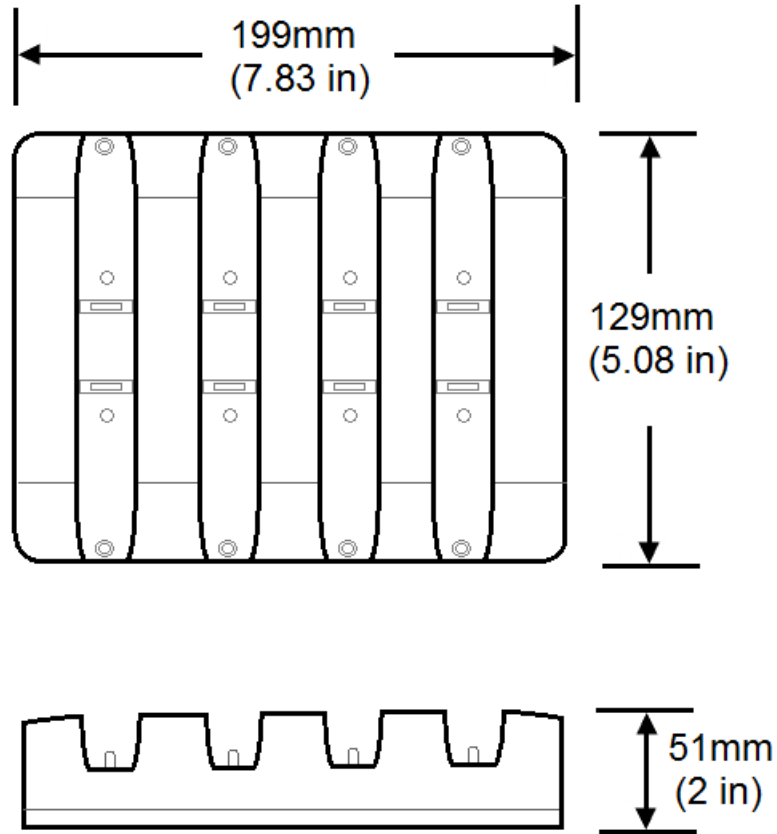
Figure 32-6 Tablet 700 Series 4-Bay Tablet Charger Dimensions
