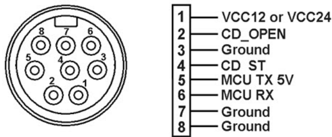
Figure 33-6 8-Pin Mini-DIN (Series 2) Cash Drawer Connector
