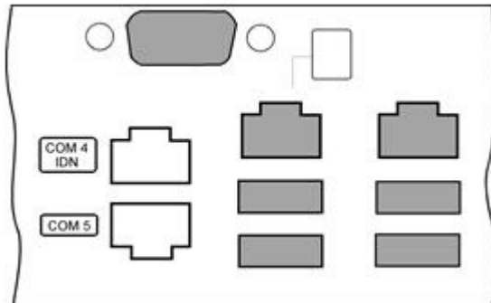
Figure 13-2 MICROS PC Workstation 2010 Connectors
