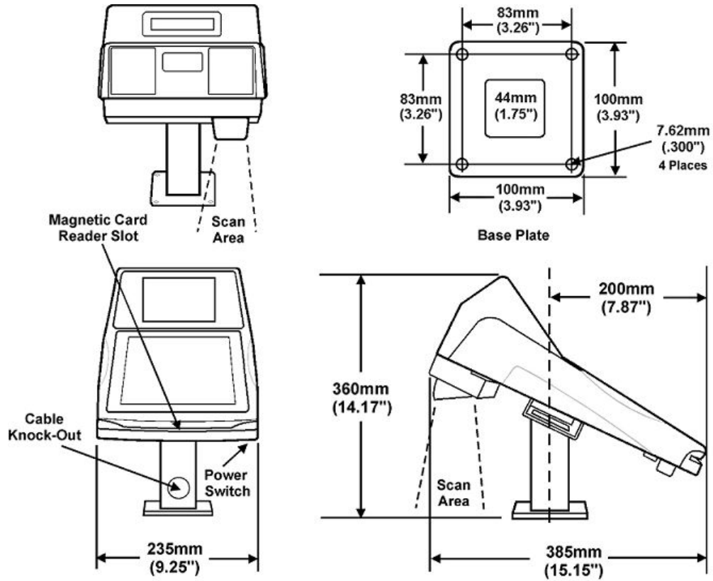
Figure 32-40 KW270 on Stand with Updated Scanner Housing Dimensions
