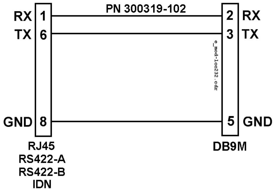
Figure 34-2 Modular LCC/RS232 to DB9 Male Connector
