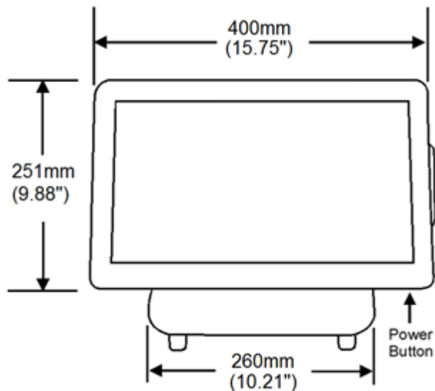
Figure 32-8 Workstation 6 Series Front Dimensions
