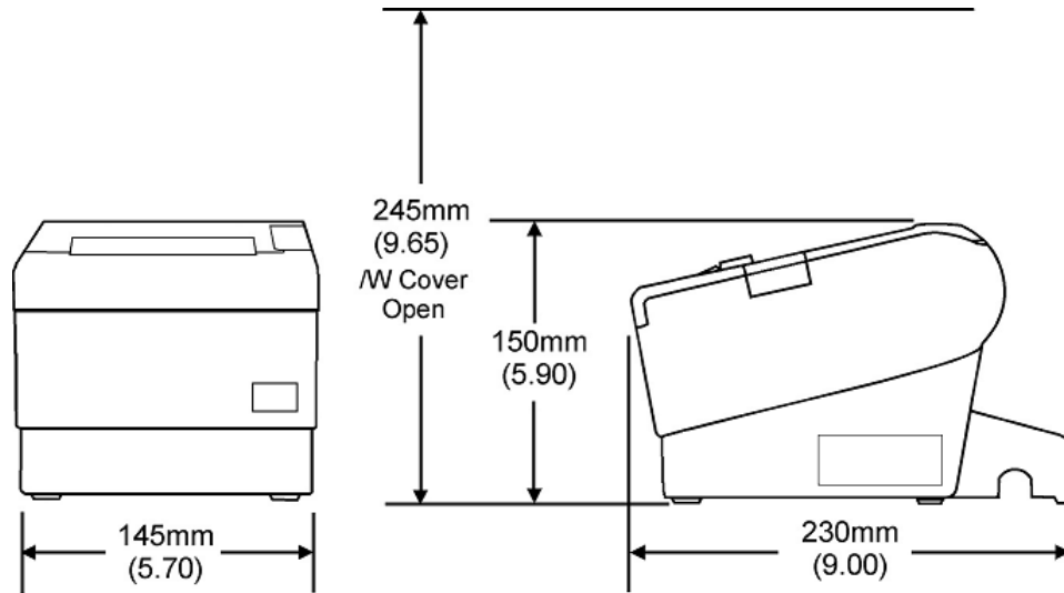
Figure 32-48 TM-T88 Thermal Roll Printer Dimensions
