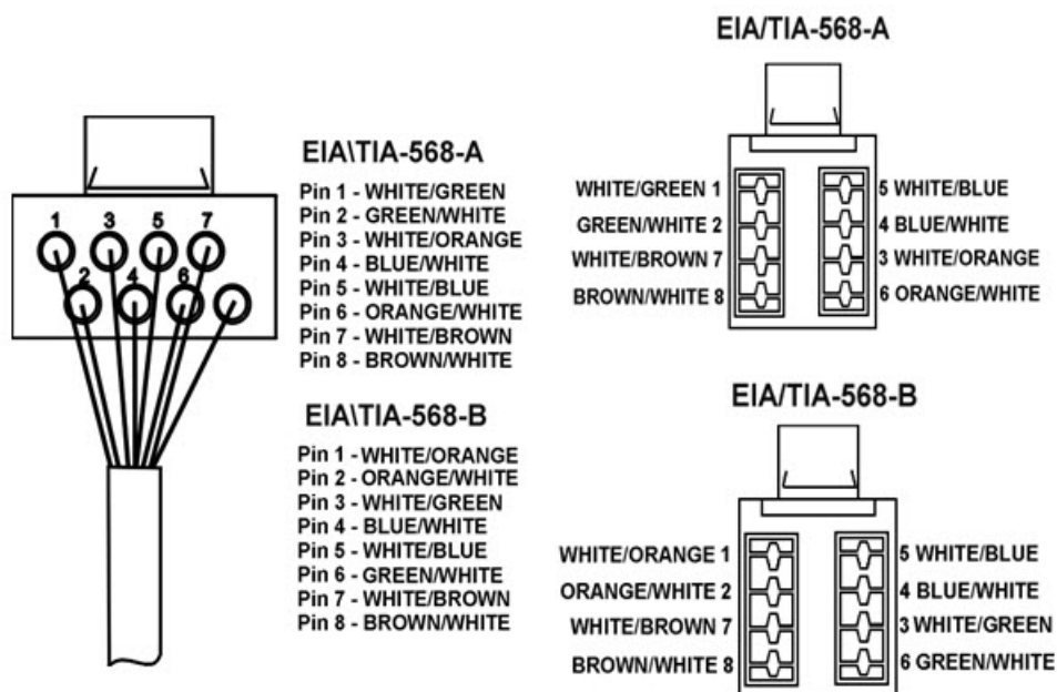
Figure 30-3 Keystone Modular (left) or 110 Connect Modular (right)
