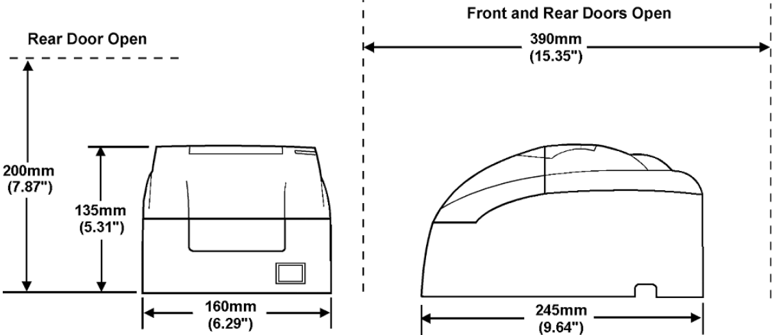
Figure 32-50 U220 Auto-Cut Roll Printer Dimensions
