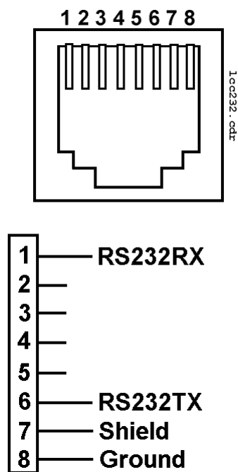
Figure 33-2 IDN or RS422-A/B Connectors Configured for RS232
