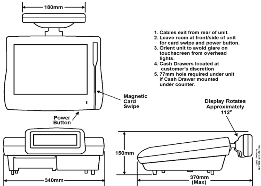
Figure 32-34 Workstation 4/4 LX – Low Profile with Rear Customer Display Dimensions
