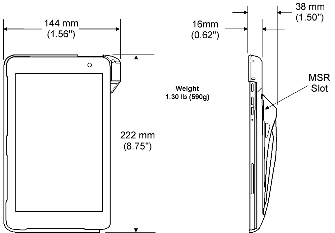
Figure 32-16 Tablet E-Series 8 Dimensions
