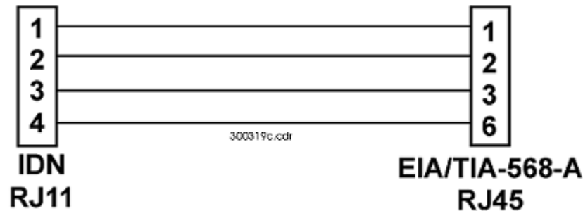
Figure 34-7 IDN to EIA/TIA-568-A Conversion Cable Diagram
