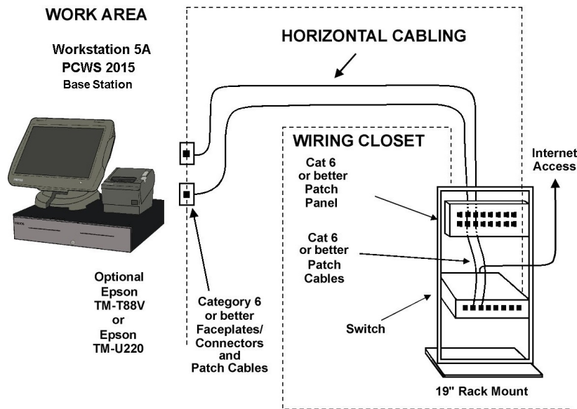
Figure 29-2 Example of a Single Workstation and Printer Installation for Symphony
