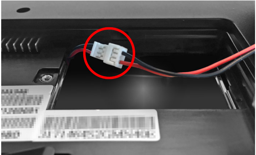
Figure 6-7 Battery Connector Cable
