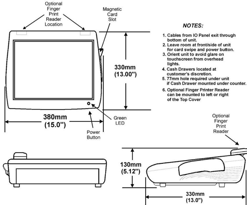
Figure 32-22 PC Workstation 2015 - Low Profile Dimensions
