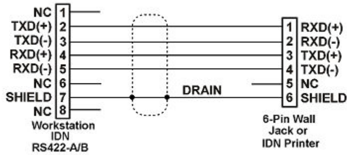
Figure 34-6 Workstation to Printer IDN Hook-up Cable Diagram
