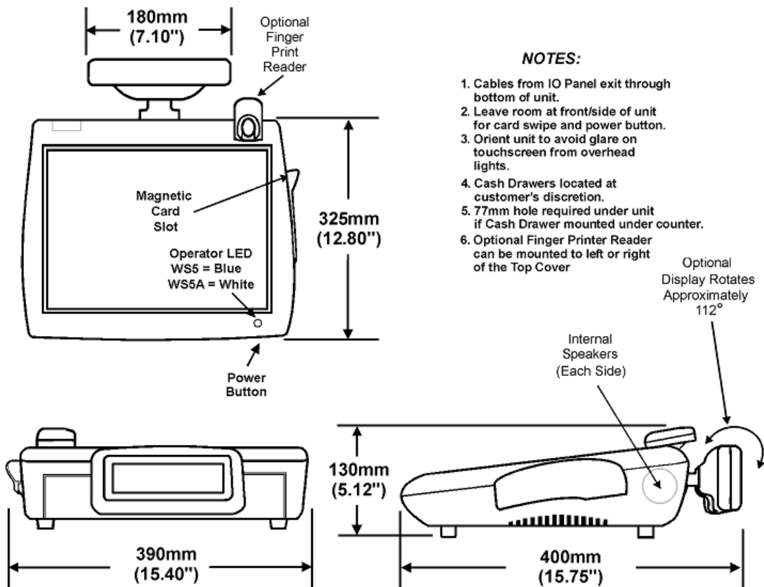
Figure 32-28 Workstation 5/5A Dimensions with Integrated LCD Customer Display
