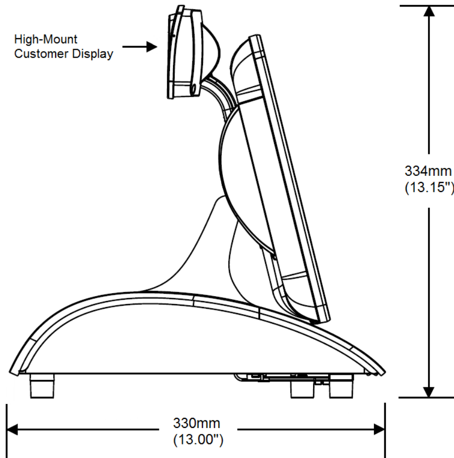
Figure 32-11 Dimensions (Side) with the High-Mount Customer Display
