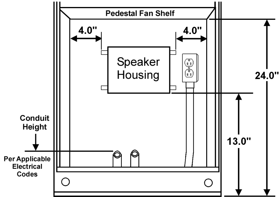
Figure 18-4 Pedestal AC Outlet - Recommended AC Outlet Location
