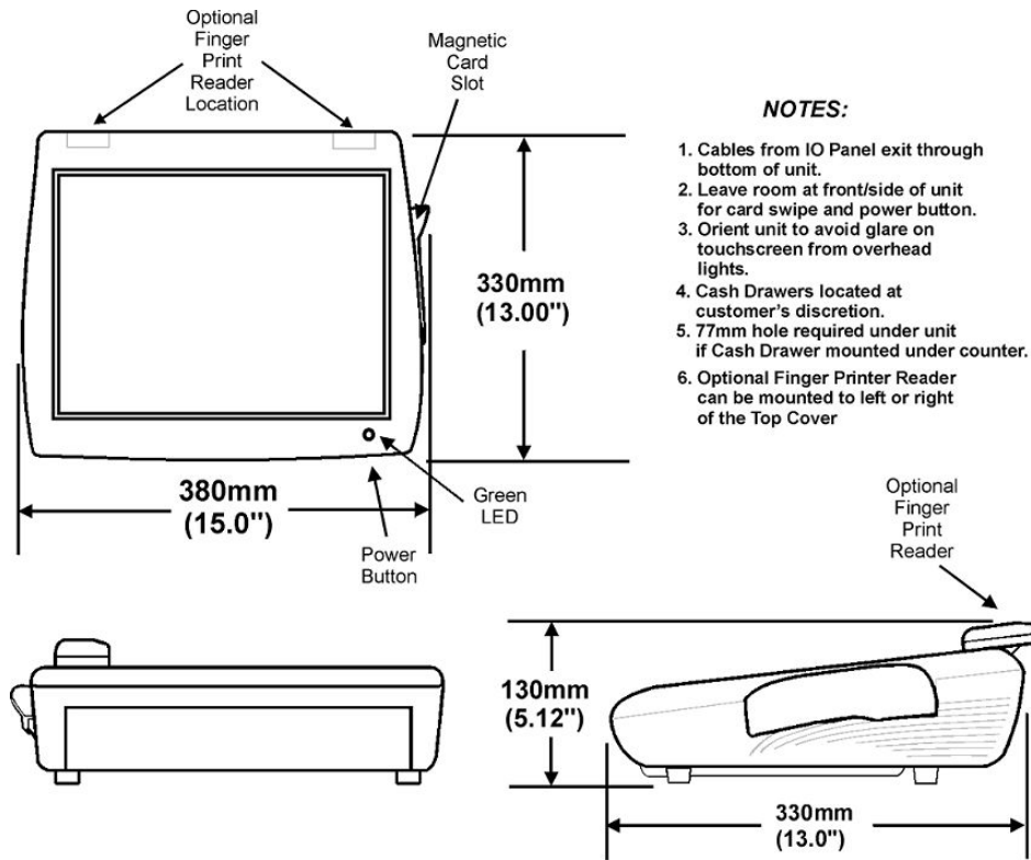
Figure 32-23 PC Workstation 2015 - Low Profile with Customer Facing Display Dimensions
