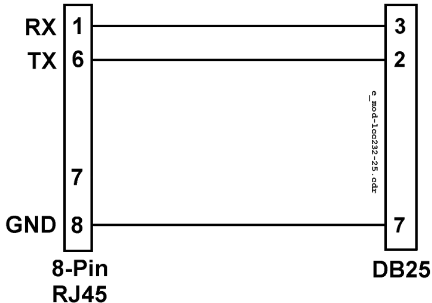
Figure 34-3 Modular LCC/RS232 to DB25 Connector
