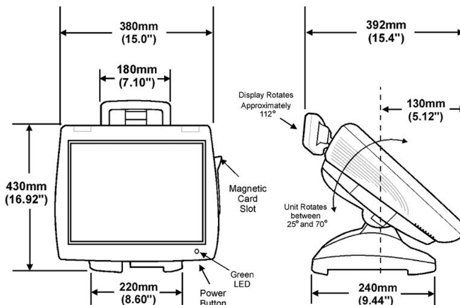
Figure 32-25 PC Workstation 2015 on Stand - LCD Customer Display Dimensions
