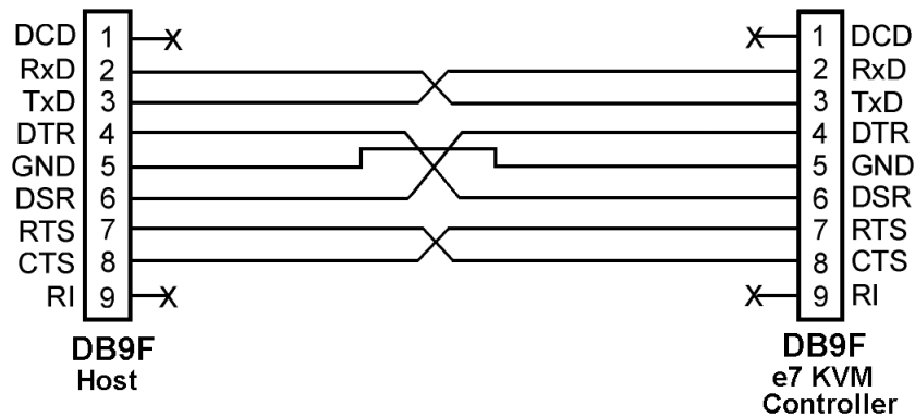
Figure 34-1 Null Modem Cable Pin-Outs
