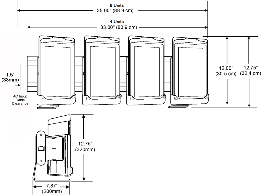
Figure 32-18 Tablet E-Series Multi-Unit Charger - Surface Mount Dimensions
