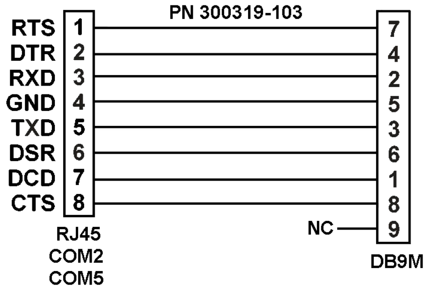
Figure 34-4 Modular RS232 Port to DB9 Male Connector
