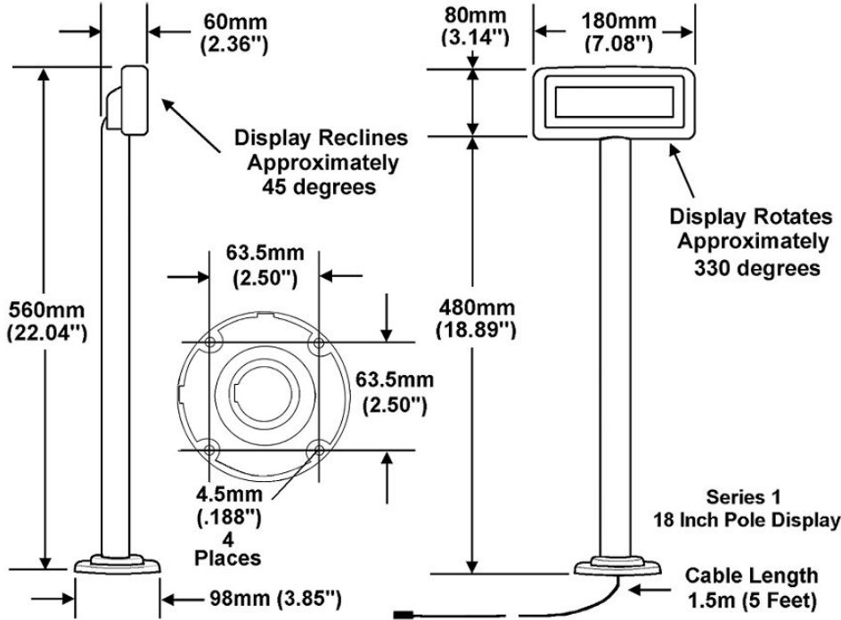
Figure 32-54 Series 1 Pole Customer Display Dimensions
