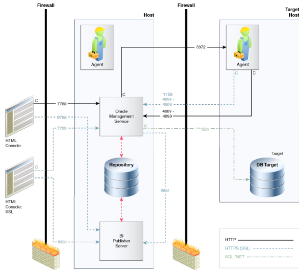
Figure 12-1 Firewall Port Requirements (Default)
