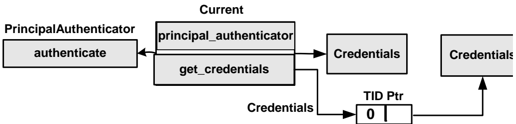
Figure 12-3 The SecurityCurrent Object
