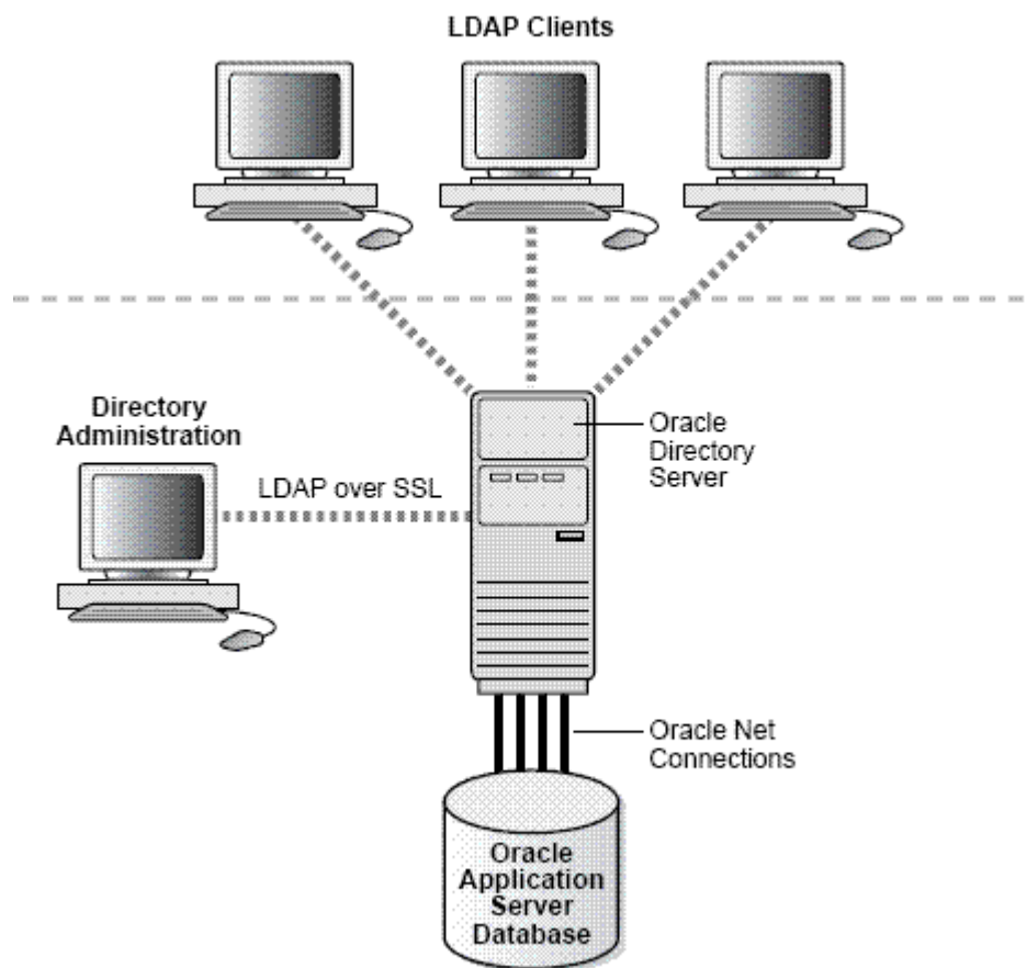
Figure 2–2 Oracle Internet Directory Illustration
